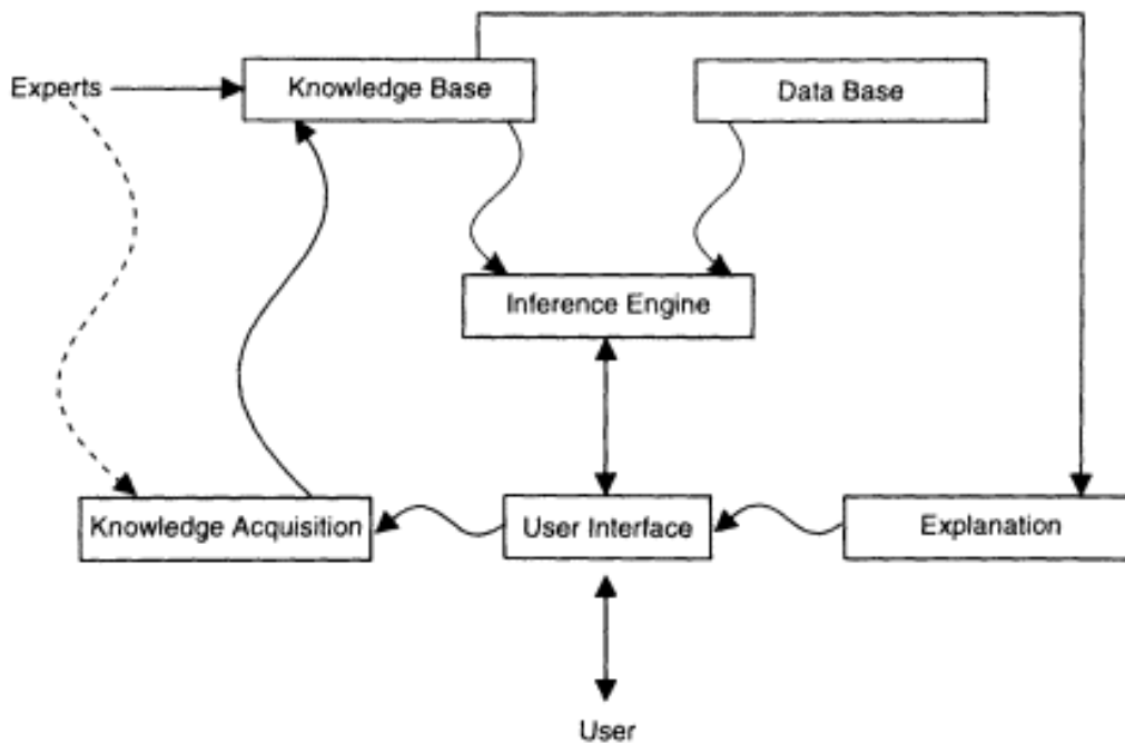
Figure 2.29 An expert system architecture.
