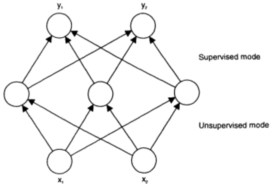
Figure 4.35 Counterpropagation neural network.
