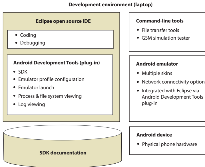
Figure 2.1 The development environment for building Android applications, including the popular open source Eclipse IDE
