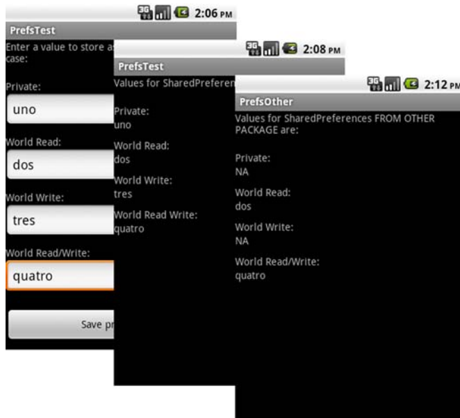
Figure 5.2 Two separate applications getting and setting SharedPreferences
