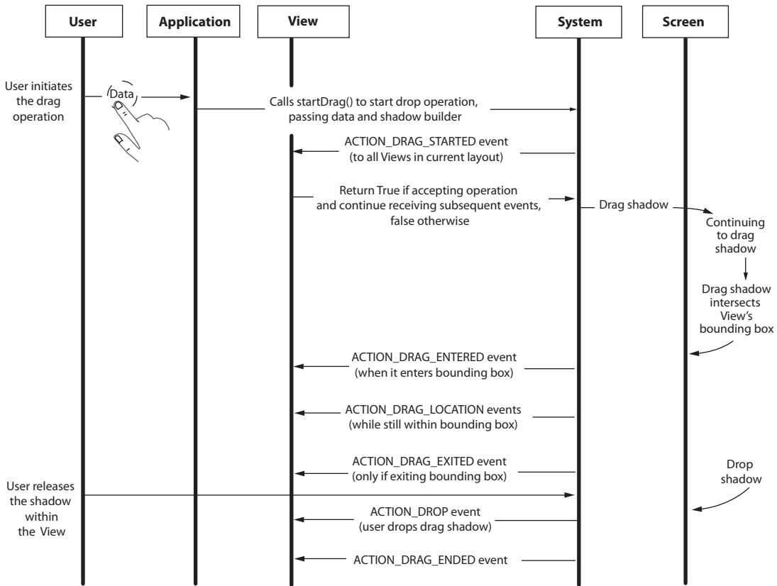
Figure 22.2 Drag-and-drop sequence diagram
