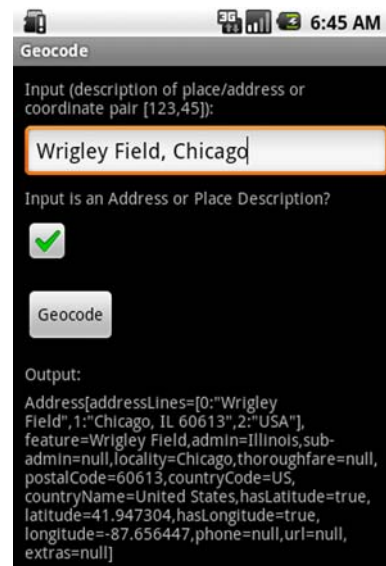
Figure 11.8 Geocoder example turning a String into an Address object that provides latitude and longitude coordinates
