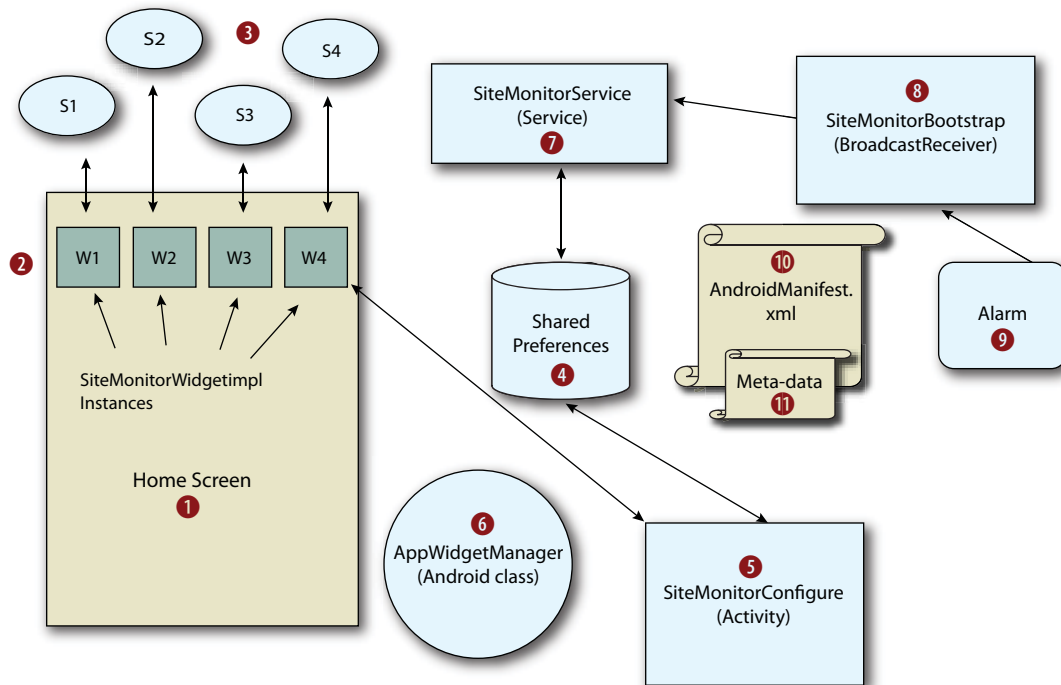
Figure 17.9 Architectural diagram of the SiteMonitor application
