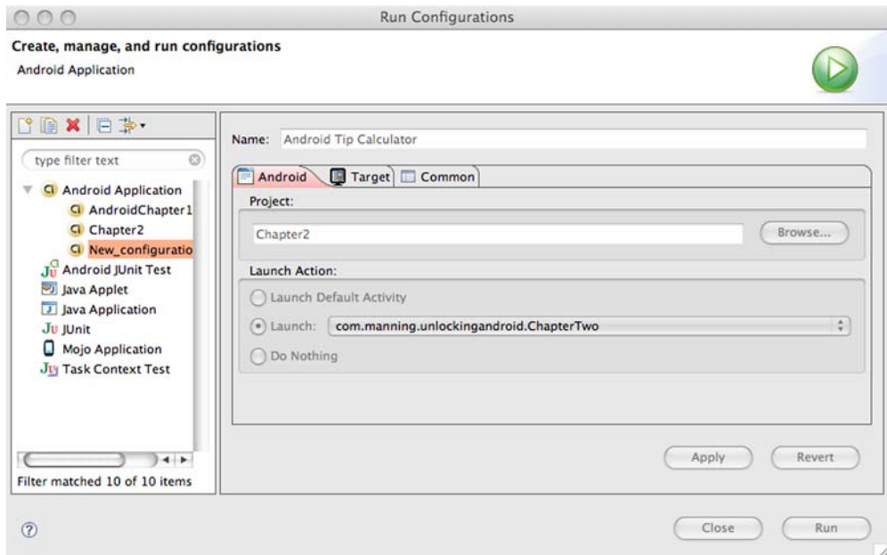
Figure 2.19 Setting up the Android emulator launch configuration
