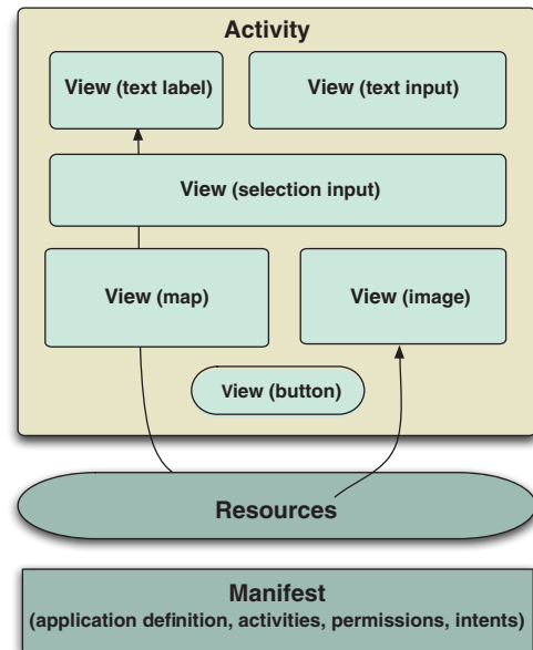
Figure 3.1 High-level diagram of Activity , view , resource , and manifest relationships, showing that activities are made up of views, and views use resources
