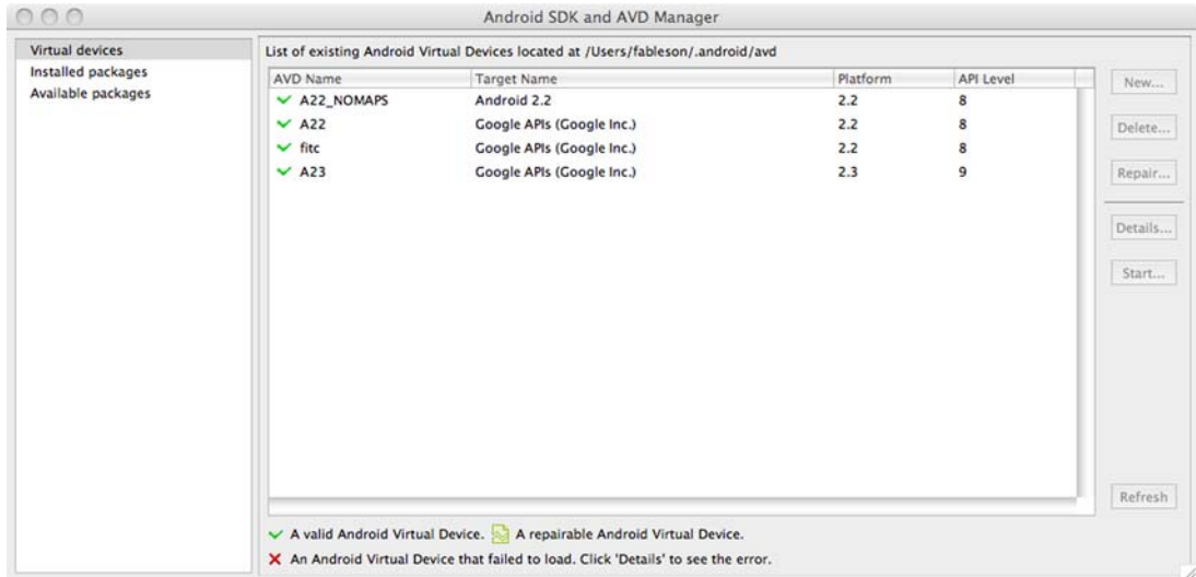
Figure A.8 Defining an Android virtual device, also known as an emulator
