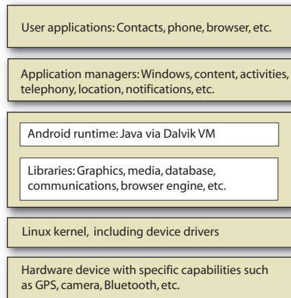
Figure 1.3 The Android stack offers an impressive array of technologies and capabilities.
