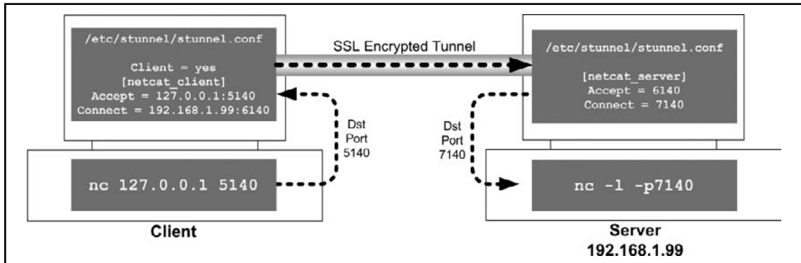
Figure 6.1 Stunnel Data Flow
