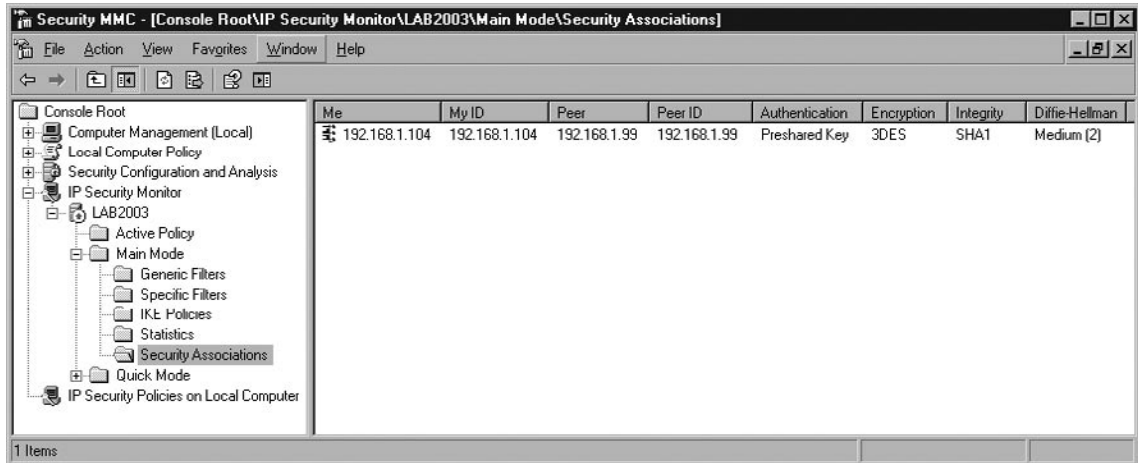
Figure 6.6 Security Associations
