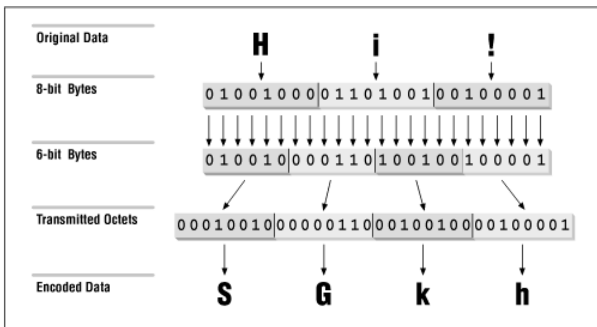
Figure 3.4: base64 encoding
