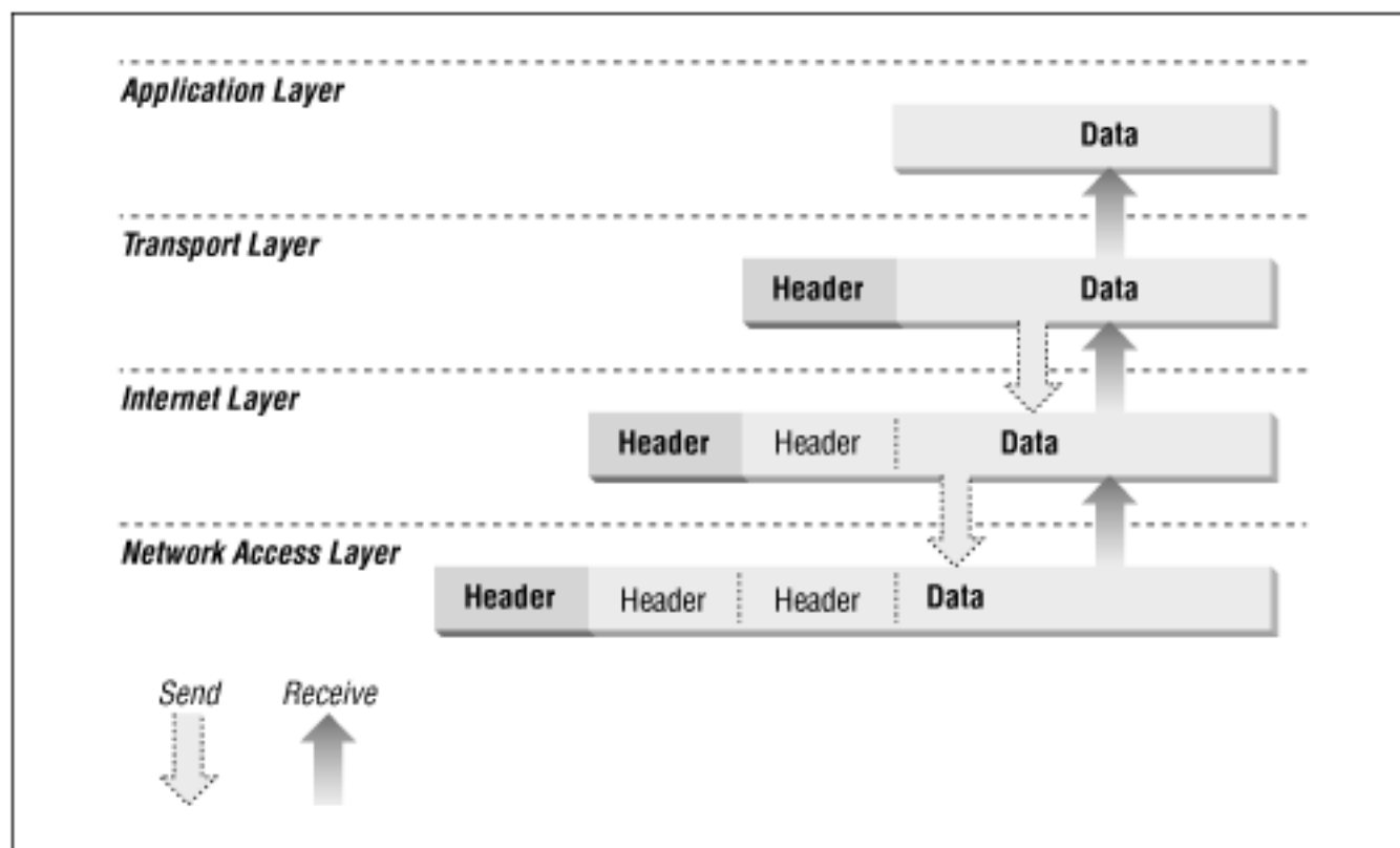
Figure 1.3: Data encapsulation
