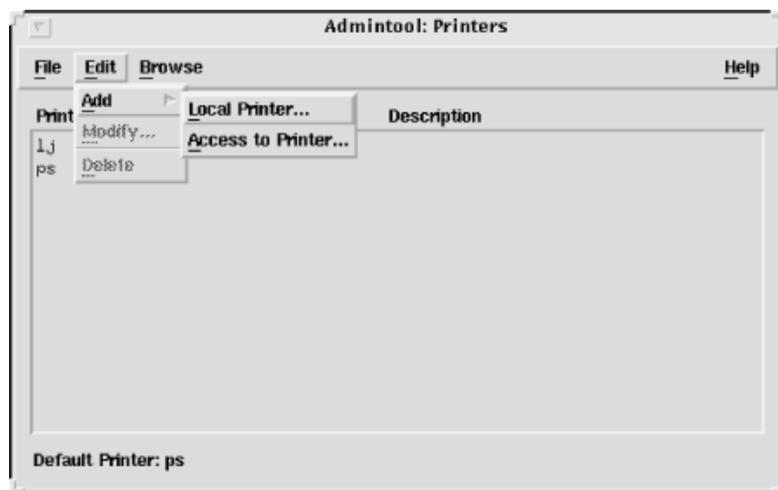
Figure 9.1: Printer Manager
