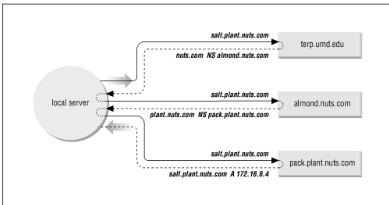
Figure 3.2: Non-recursive query
