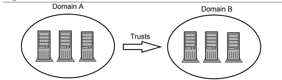
Figure 19.1 Trusts overview.
