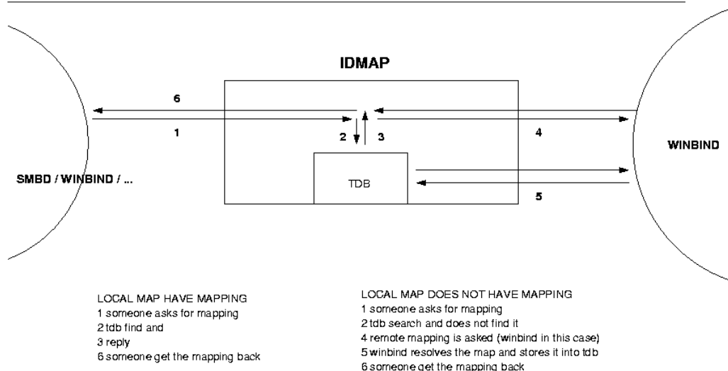
Figure 24.1 Winbind Idmap
