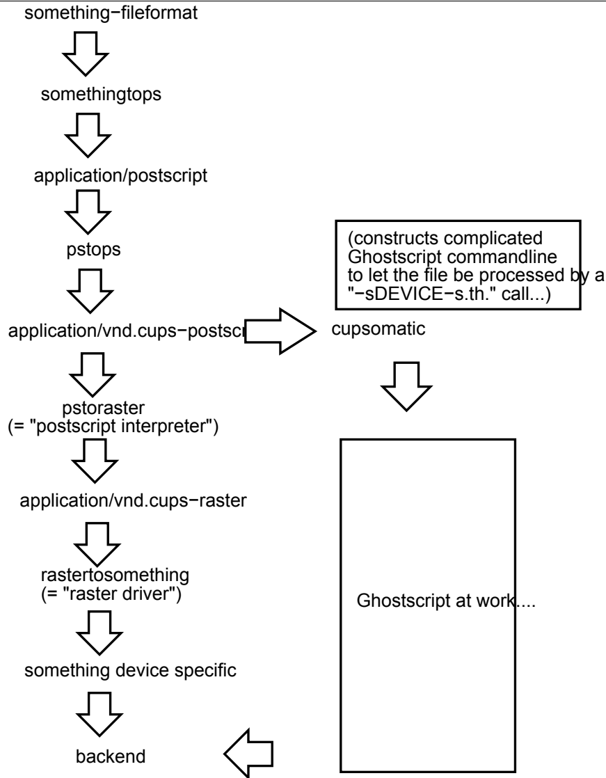
Figure 22.18 Filtering Chain with cupsomatic
