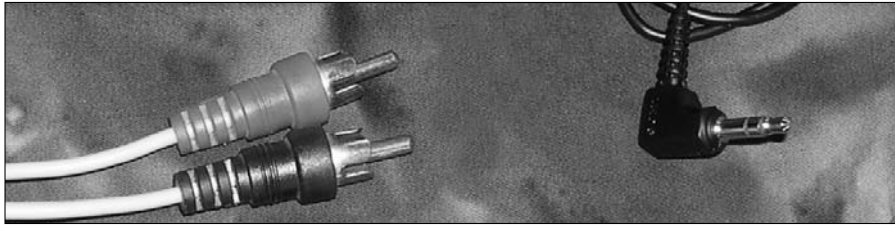
Figure 14-5: RCA-type connectors (left) and a stereo mini- plug (right).
