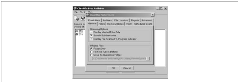
Figure 16-2. ClamWin Preferences
