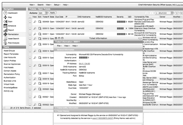
Figure 2-8: One-click assignment of a vulnerability trouble ticket.
