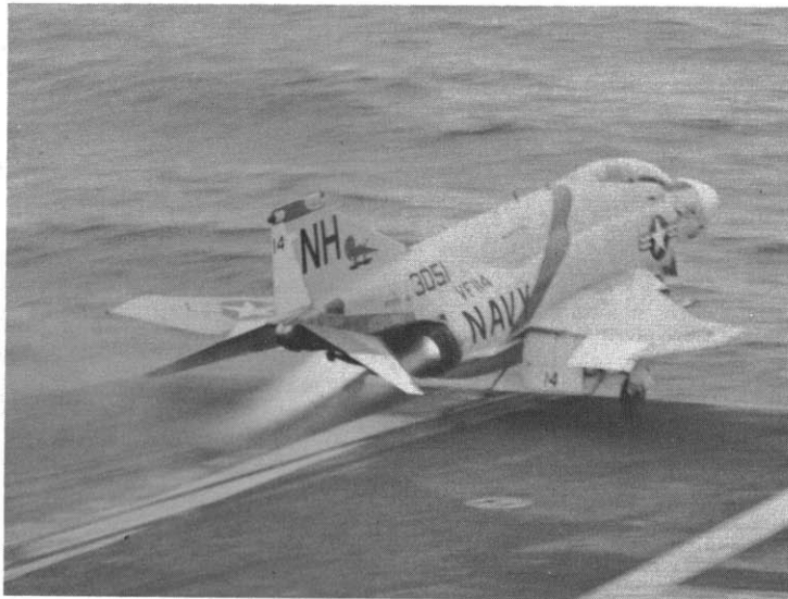
Twin tongues of searing flame burn the Pacific air as, after-burners ablaze, this F-4B roars off the waist catapult of the USS Kittyhawk (CVA-63) during a tune-up cruise prior to 1968 Westpac deployment. Combined power of the Steam catapult and the Phantom's twin J-79s have accelerated the F-4 from 0 to 120 knots in less than 300 feet. (Lou Drendel)
