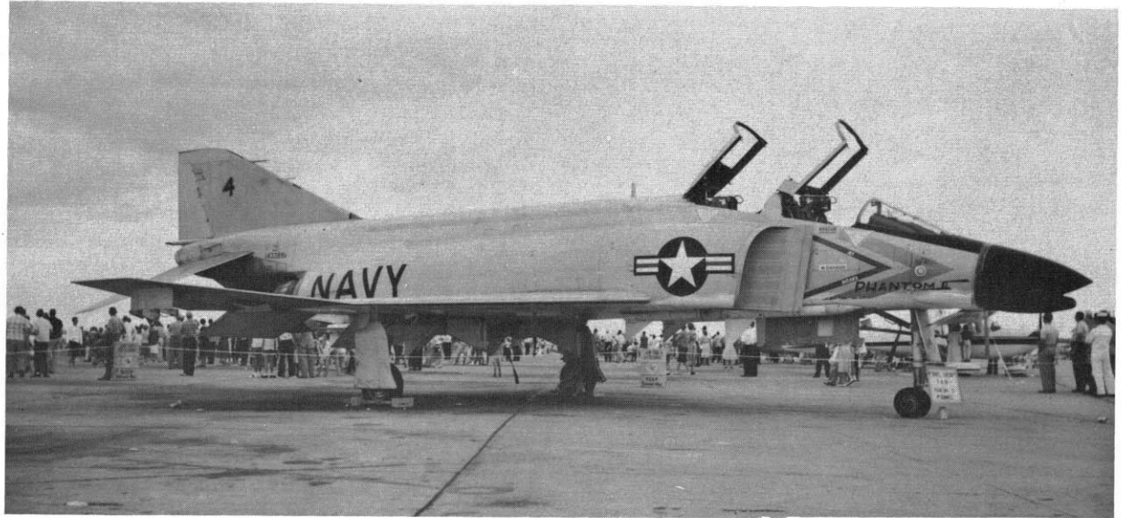
EARLY PHANTOMS—F-4A (top) has faired-in intakes used with lower powered J79-GE-3 engines. More powerful dash 8 engines required redesigned intakes. Both models have smaller nose used with 24" radar dish, and original canopy outline, later changed when seats were raised to provide better over the nose visibility for Pilot and Radar Intercept Officer. (via Paul Stevens)
