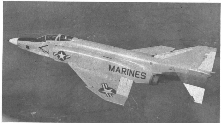
An RF-4B of the Marine Corps. The first RF-4B (151975) is illustrated above. The white strip near the leading edge of the vertical stabilizer is an antenna for long range HF communications equipment, one of several modifications made to the standard F-4B airframe to convert it to RF standard. Other differences include: a battery of cameras for forward, side and oblique reconnaissance, infra-red and radar reconnaissance equipment and flash ejectors for night-time duties. (McDonnell-Douglas)
