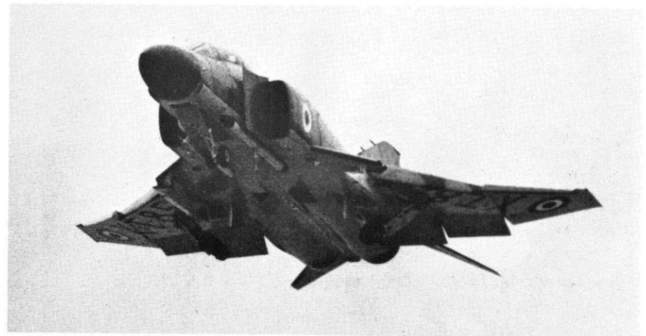
F-4M during gear retraction sequence. Also evident is the drooped flap configuration which provides additional lift during slow speed flight. (McDonnell-Douglas)
