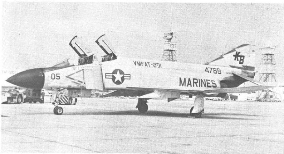
Two views of the late model F-4J for the Marine Corps. The 'J' has numerous improvements over the 'B', including AWG-10 pulse doppler radar fire control, improved AJB-7 bombing system, drooped flaps and slotted leading edges in the stabilator for better control at approach speeds, as well as a slightly larger fuel capacity. Note the position of the open drag chute door under the rudder. (USMC)
