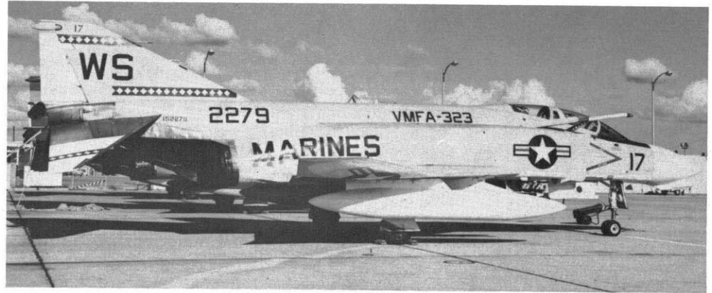
Marine Corps (former Navy) Phantom, with air refueling probe extended. The Navy uses the probe and drogue method of aerial refueling, largely because of the need to employ the 'buddy system', whereby another aircraft of similar type can be fitted with fuel tanks with extendable drogue. (Sgt. Norman Taylor)
