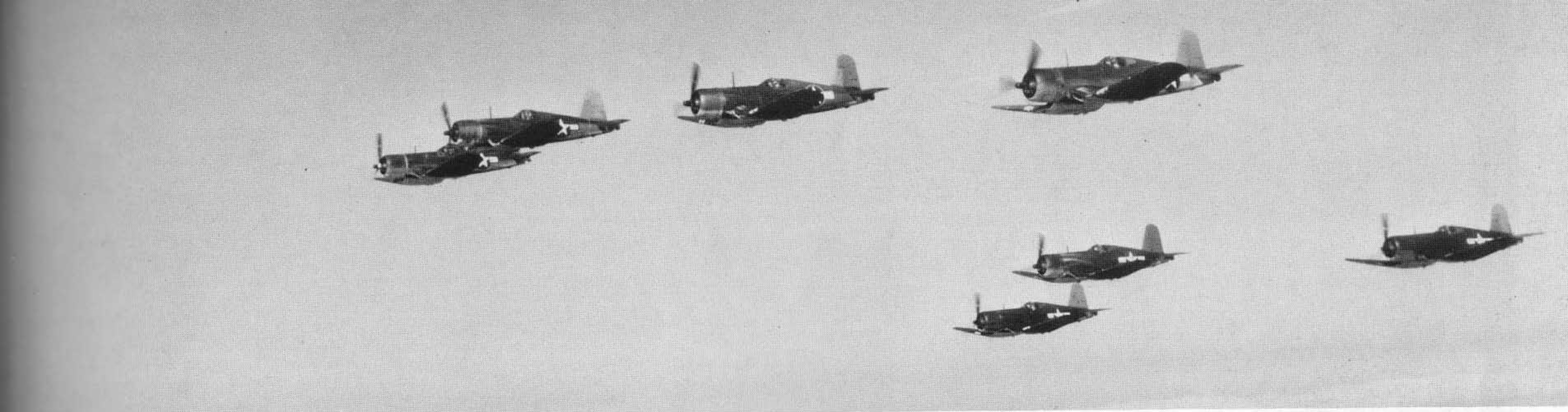
F4U-1 and F4U-1A Corsairs from MCAS Cherry Point. To compensate for the additional weight added by changes from the XF4U-1, Vought installed a P&W R-2800-8 engine with 2,000-HP for take-off. October 1943. [National Archives]
