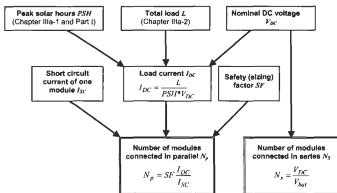
Figure 1 Sizing based on energy balance.
