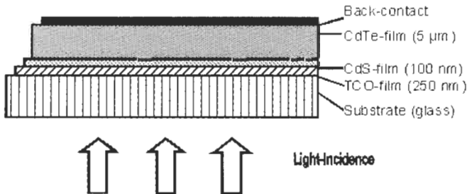
Figure 1 Film sequence of the CdTe thin-film solar cell.
