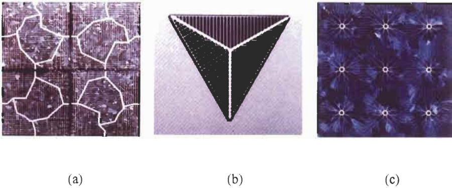
Figure 16 Patterns in photovoltaics. (a) One of the patterns developed by the Atomic Institute Vienna [5, 6]. © Photon magazine. Reprinted with permission. (b) The triangular cell developed by one of the authors (R.L.C.) at University of Southampton, UK. (c) ECN Pin-up. (Source: ECN homepage.)
