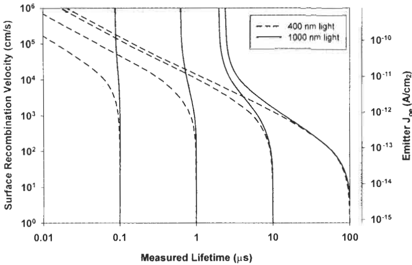
Figure 2 Effective lifetime for a 300 \mu\text{m} , 1 \Omega\text{ cm} p-type wafer as a function of the surface recombination velocity. The curves, modelled with PC1D for steady-state conditions, correspond to wafers with 0.1, 1, 10 and 100 \mu\text{s} bulk lifetimes. Two sets of curves are shown, for 400 nm and 1000 nm, monochromatic illumination, respectively.
