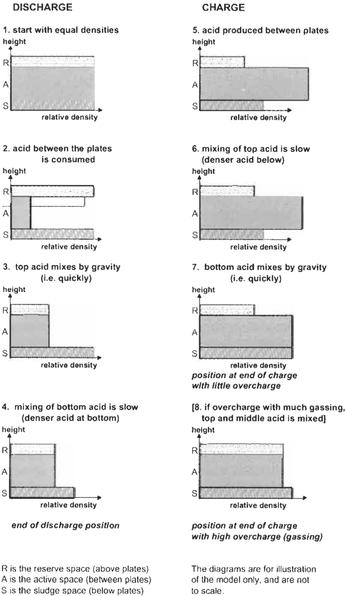
Figure 7 Principle of stratification. R denotes the reserve space (above plates), A is the active space (between plates) and S is the sludge space (below plates). The diagrams are for illustration of the model only, and are not to scale.
