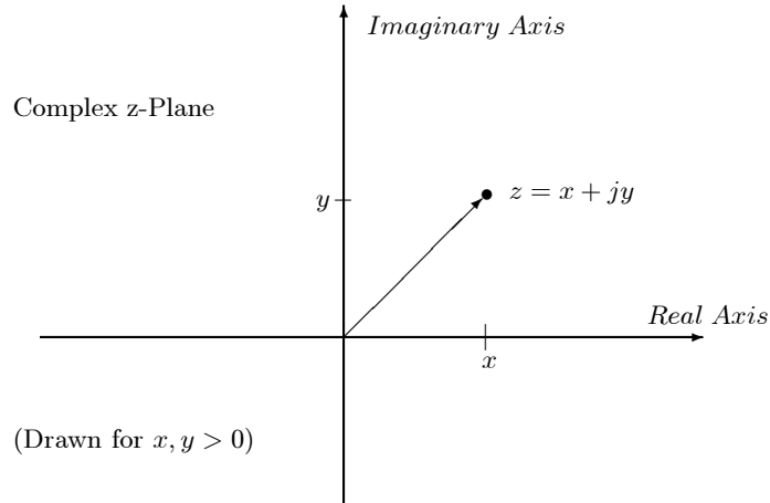
Figure 2.1: Visualizing a Complex Number z In The Complex z -Plane
