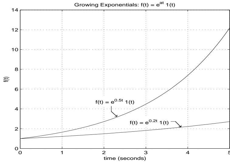
Figure 3.4: Growing Exponentials
