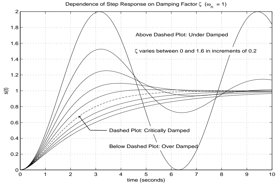
Figure 5.4: Step Response For Standard Second Order System: Dependence on Damping Factor Overhoot, Undershoot, Time-To-Peak. From the above discussion, one sees that for small \zeta , the step response of our standard second order system (5.55) exhibits oscillatory behavior. When the response goes above unity - the steady state value - we say that the response exhibits an overshoot. When it dips below unity, we say that we have an undershoot. More specifically, one observes that for small enough \zeta , the step response exhibits a rapid rise to a well defined maximum. In such a case, we say that the response exhibits overshoot. See Figure 5.5.
