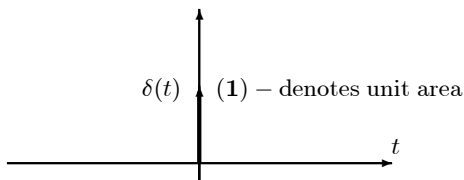
Figure 3.2: Unit Dirac Delta Distribution
