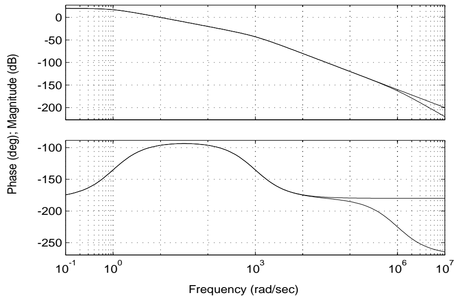
Figure 6.10: L = \left[ \frac{10}{s-1} \right] \left[ \frac{10^3}{s+10^3} \right] \left[ \frac{10^6}{s+10^6} \right] .
