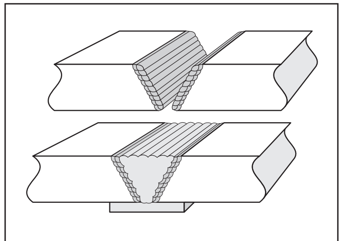
Figure 9-2 Buttering layers
