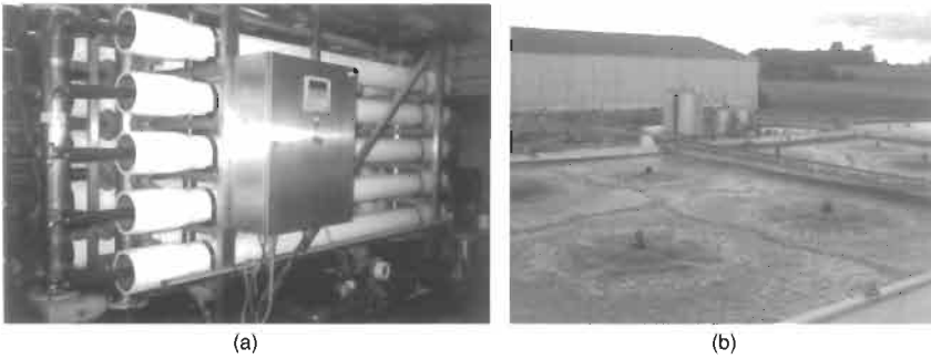
Figure 5.21 (a) Ultrafiltration and (b) bioreactors at Pasfrost
