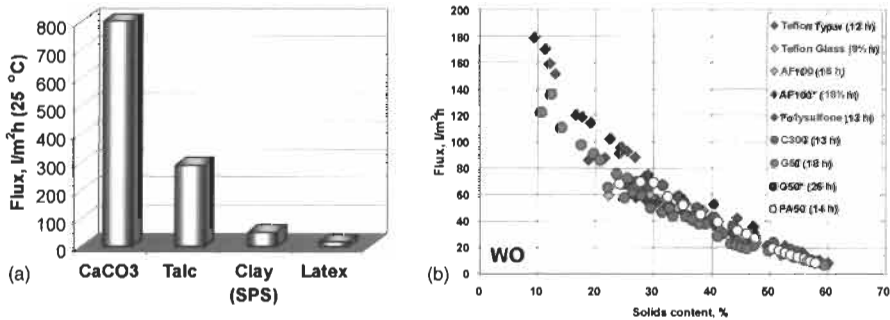
Figure 3.28 (a) Microfiltration of coating colour components; VSEP L, 465 cm 2 , Teflon Typar 0.1 μm (TetraTec), pressure 6.9–20.7 bar, amplitude 2–2.5 cm. (b) Concentration of wet offset (WO) coating colour, VSEP L, 465 cm 2 , various membranes, pressure 6.9–27.6 bar, amplitude 1.9–3.2 cm. Fluxes recalculated to 40°C (Nuortila-Jokinen and Nyström, 2000)
