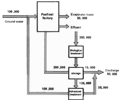
Figure 5.19 Mass balance around Pasfrost reclamation facility (data in \text{m}^3 \text{year}^{-1} )
