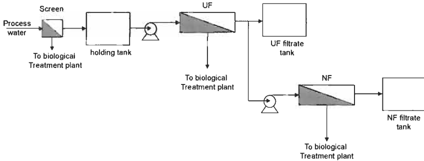
Figure 5.13 Process flow diagram of Kirknemi white water recycling plant
