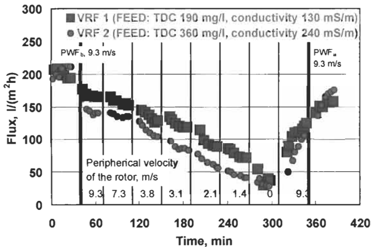
Figure 3.23 Effect of rotor blade tip speed in the CR filter on the permeate flux for the filtration of acidic clear filtrate from a paper machine. NF200 membrane from Dow-Film Tec, pH 4.9, 35°C, 10 bar TMP
