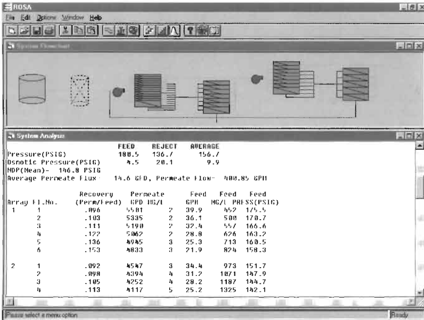
Figure 4.7 Scaling indices (Argo Analyzer, Betz-Dearbon)
