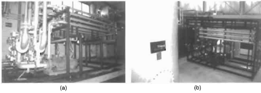
Figure 5.8 (a) Heat exchange loop (b) membrane bioreactor
