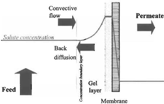
Figure 2.17 Concentration polarisation
