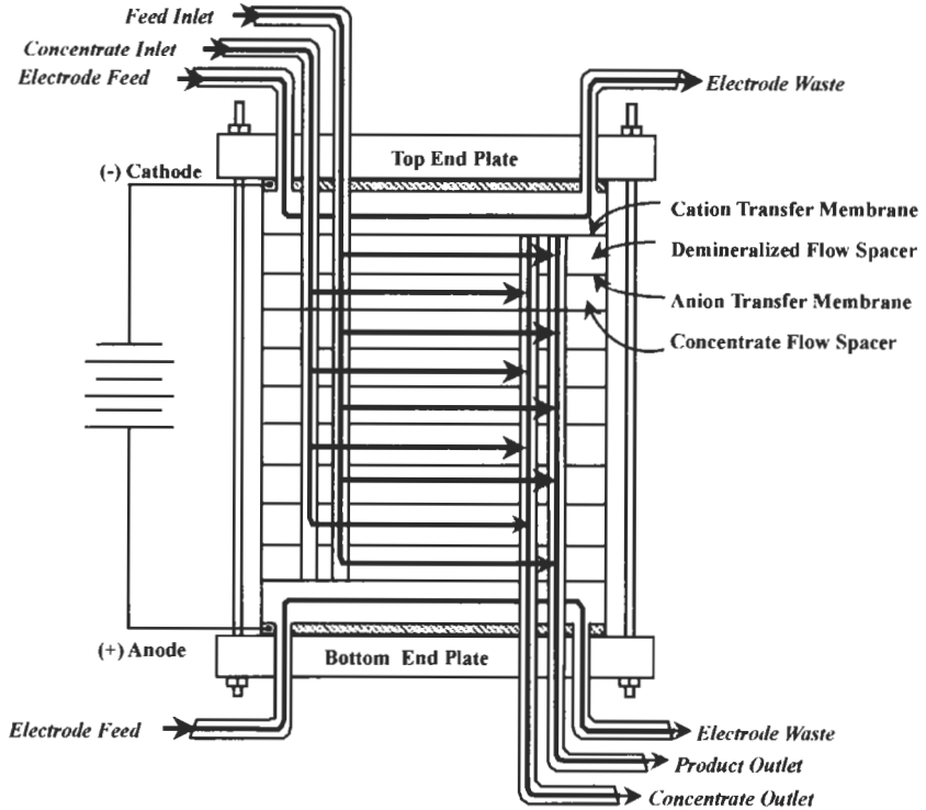
Figure 2.8 Electro dialysis stack (by kind permission of Ionics)
