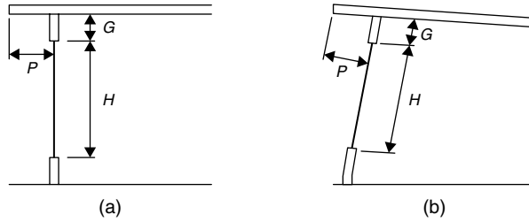
FIGURE 6.7 Window with overhang: (a) vertical window, (b) general case of tilted window.
