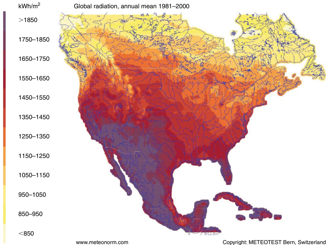
FIGURE 2.31 Annual total solar irradiation on horizontal surface for North America. Source: Meteonorm database of Meteotest ( www.Meteonorm.com ).
