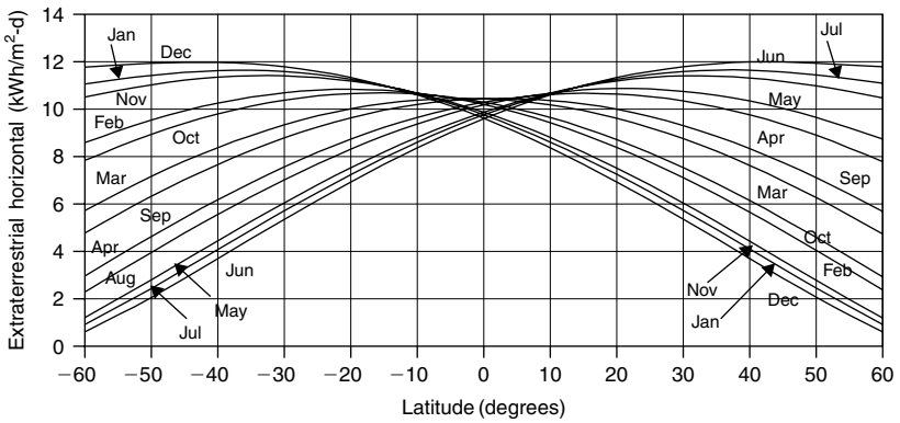
FIGURE A3.5 Monthly average daily extraterrestrial insolation on horizontal surface (kWh/m 2 -d).
