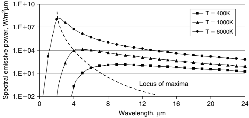
FIGURE 2.22 Spectral distribution of blackbody radiation.
