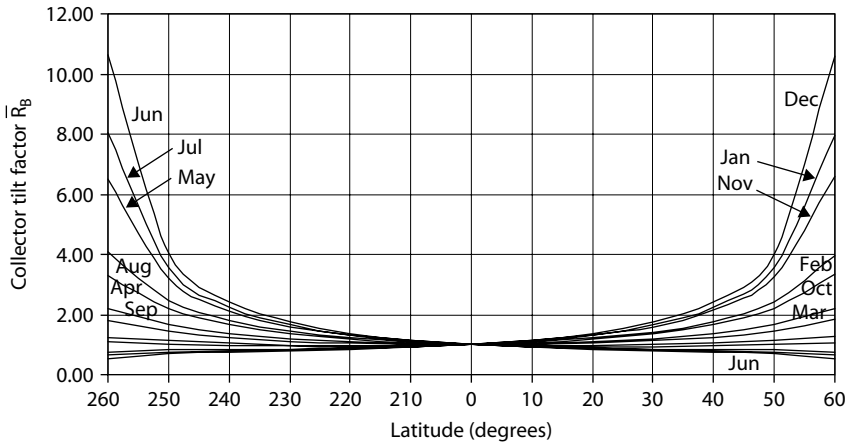
FIGURE A3.6 Values of \bar{R}_B for collector slope equal to latitude.
