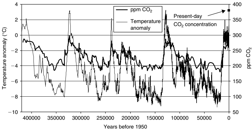
FIGURE 1.1 Temperature and CO 2 concentration from the Vostok ice core.
