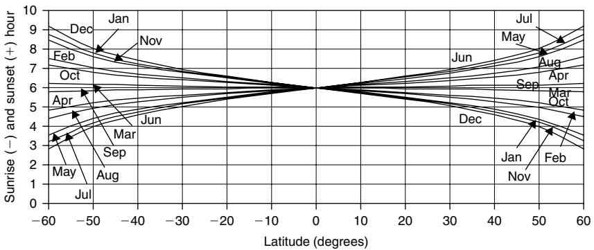
FIGURE A3.1 Sunset and sunrise angles in various months for a number of latitudes.
