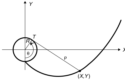
FIGURE 5.6 Mirror coordinates for ideal non-imaging cusp concentrator.
