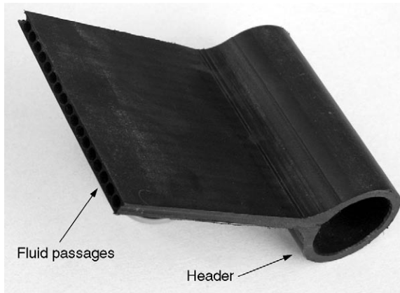
FIGURE 3.4 Photograph of a plastic collector absorber plate.
