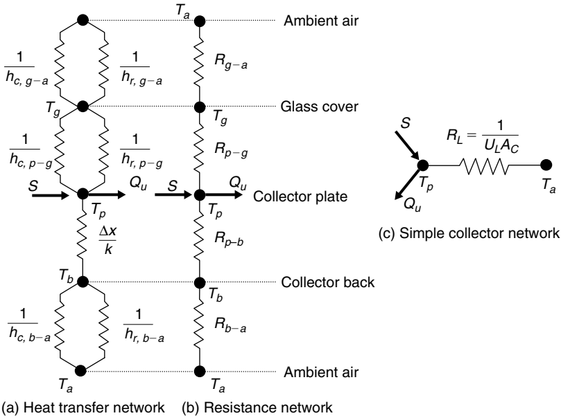
FIGURE 3.25 Thermal network for a single cover collector in terms of (a) conduction, convection, and radiation; (b) resistance between plates; and (c) a simple collector network.
