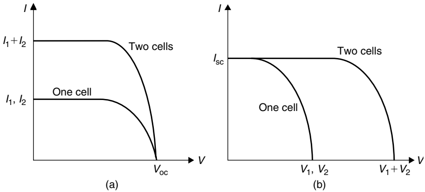
FIGURE 9.10 Parallel and series connection of two identical solar cells. (a) Parallel connection. (b) Series connection.
