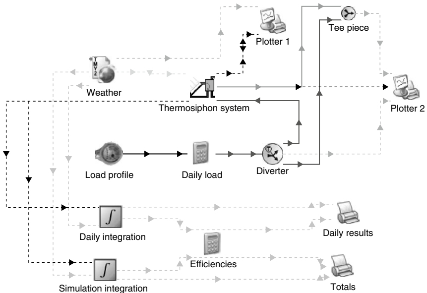
FIGURE 11.12 Model diagram of a thermosiphon solar water heating system in simulation studio.
