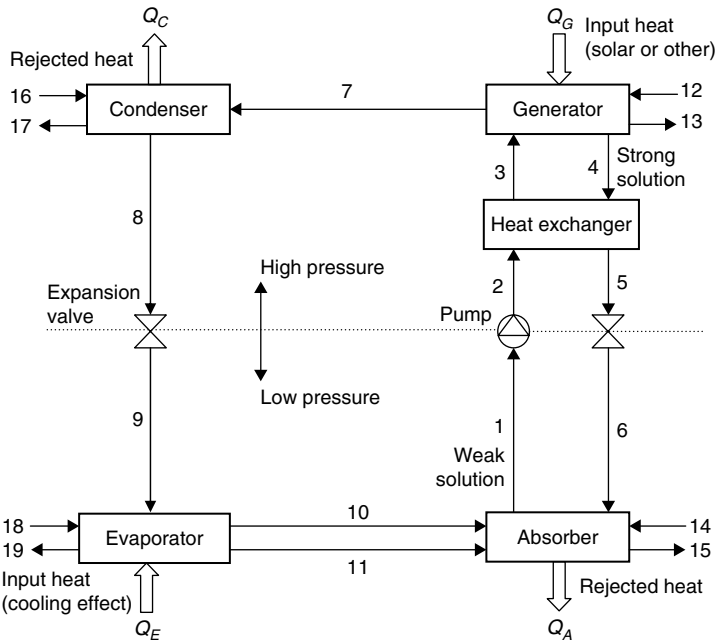
FIGURE 6.23 Schematic diagram of an absorption refrigeration system.
