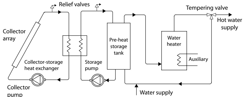
FIGURE 11.9 Schematic diagram of the standard of water heating system configuration.
