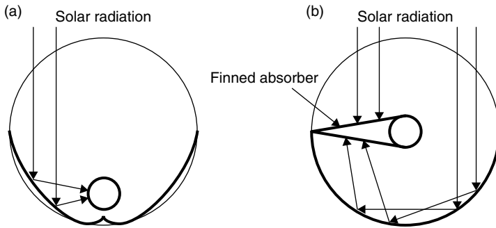
FIGURE 3.10 Integrated CPC tubes. (a) Internal compound parabolic. (b) Circular reflector with finned absorber.
