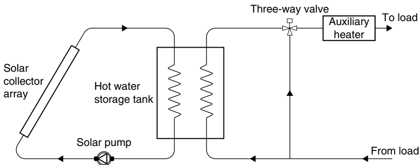
FIGURE 7.2 Simple industrial process heat system with a series configuration of auxiliary heater.
