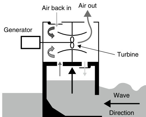
FIGURE 1.10 Principle of operation of a wave energy converter.
