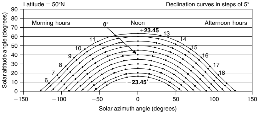
FIGURE A3.4 Sun path diagram for 50°N latitude.
