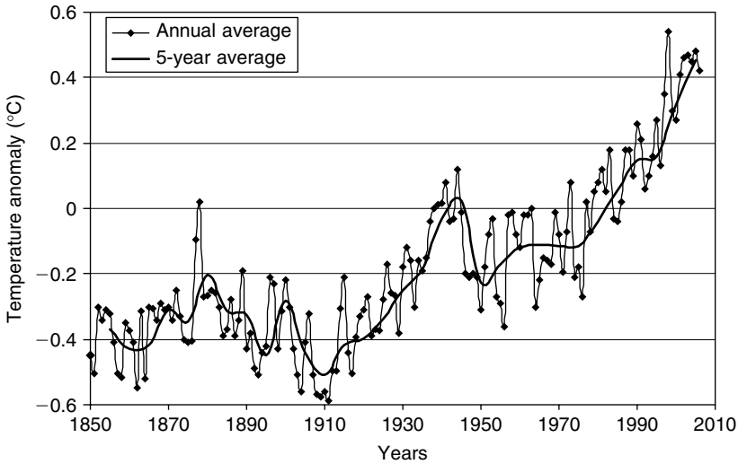
FIGURE 1.2 Global temperature since 1850.
