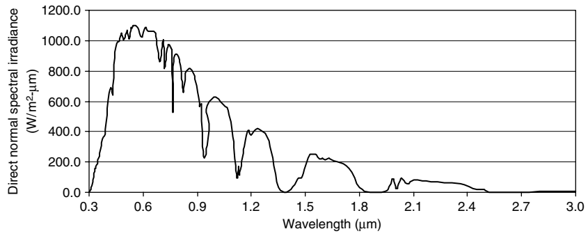
FIGURE A4.1 Direct normal solar irradiance at air mass 1.5.
