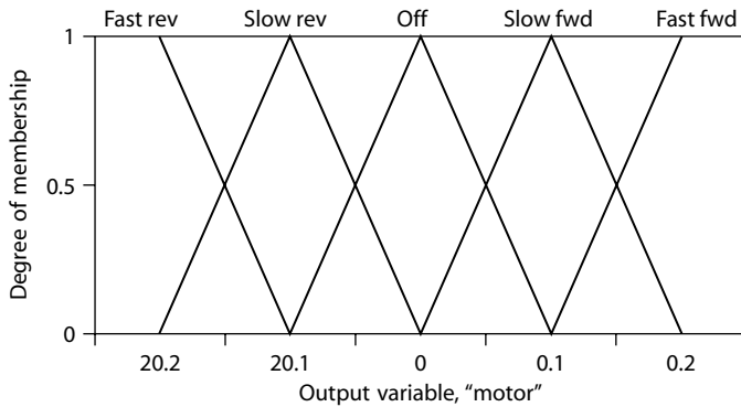
FIGURE 11.25 Membership functions for linguistic variables describing motor operation.
