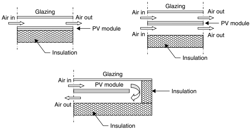
FIGURE 9.24 Details of an air PV/T collector.
