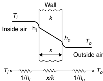
FIGURE 6.1 Heat transfer through a building element and equivalent electric circuit.
