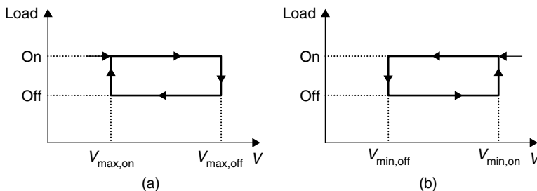
FIGURE 9.14 Operating principle of overcharge and overdischarge protection. (a) Overcharge. (b) Over-discharge.
