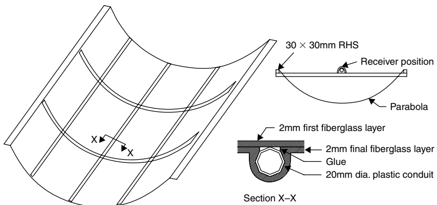
FIGURE 3.15 Fiberglass parabola details.
