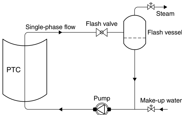
FIGURE 7.5 The steam-flash steam generation concept.
