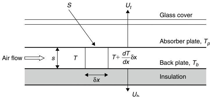
FIGURE 3.30 Schematic diagram of an air-heating collector.
