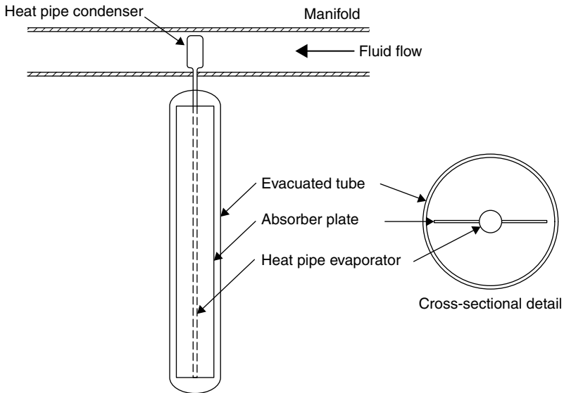
FIGURE 3.7 Schematic diagram of an evacuated tube collector.
