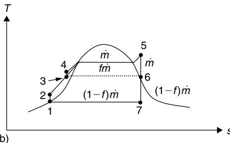
FIGURE 10.11 Rankine power plant cycle with regeneration. (a) Regenerative Rankine cycle schematic. (b) T-s diagram.
