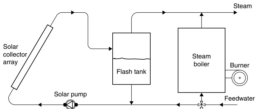
FIGURE 7.4 Simple industrial process heat steam system with a parallel configuration with an auxiliary steam boiler.
