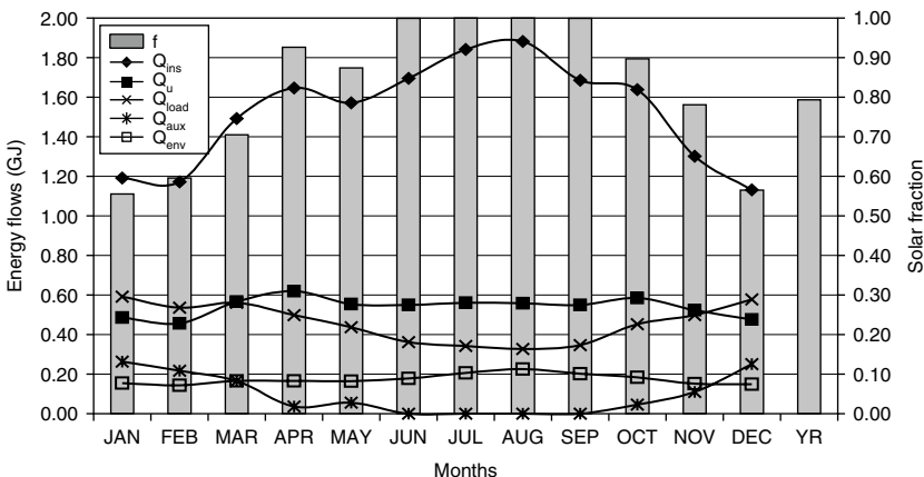
FIGURE 11.13 Energy flows of the thermosiphon solar water heater.
