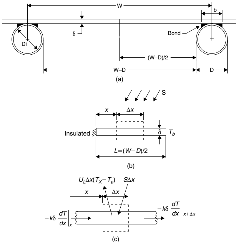
FIGURE 3.27 Flat-plate sheet and tube configuration. (a) Schematic diagram. (b) Energy balance for the fin element. (c) Energy balance for the tube element.
