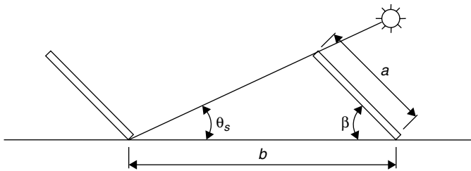
FIGURE 5.25 Row-to-row collector shading geometry.
