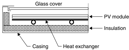
FIGURE 9.23 Details of a water PV/T collector.
