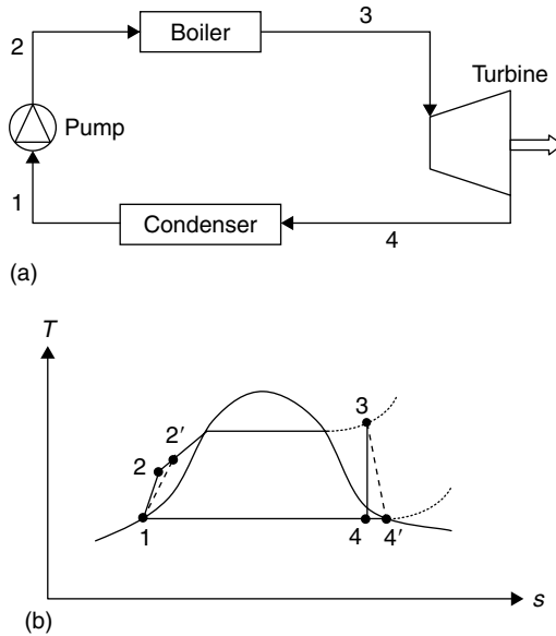
FIGURE 10.9 Basic Rankine power plant cycle. (a) Basic Rankine cycle schematic. (b) T-s diagram.
