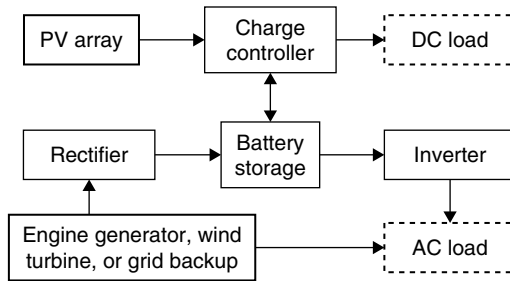
FIGURE 9.19 Schematic diagram of a hybrid connected system.
