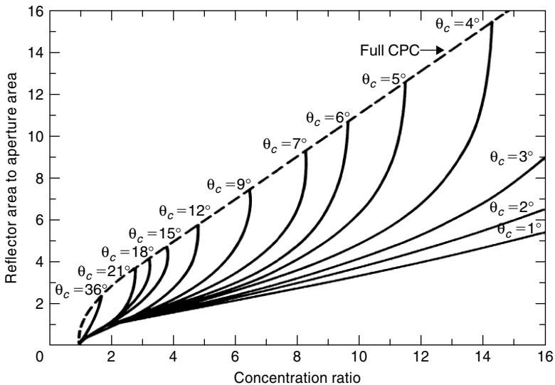
FIGURE 3.36 Ratio of reflector to aperture area for full and truncated CPCs. (Reprinted from Rabl (1976) with permission from Elsevier.)
