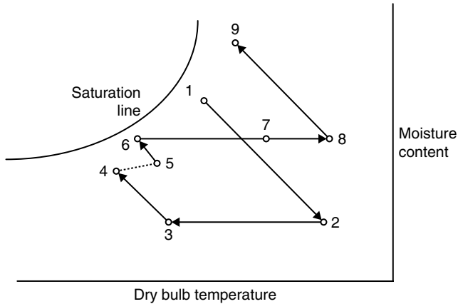
FIGURE 6.20 Psychrometric diagram of a solar adsorption process.
