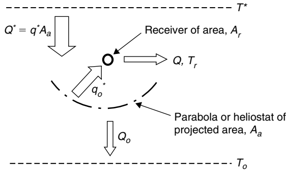
FIGURE 3.44 Imaging concentrating collector model.
