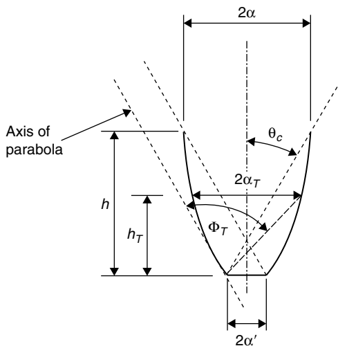
FIGURE A6.1 A truncated CPC. Its height-to-aperture ratio is about one half the full height of a CPC.
