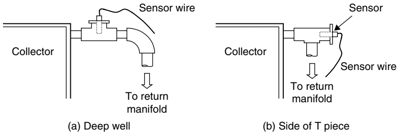
FIGURE 5.30 Placement of collector sensor.
