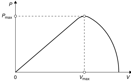
FIGURE 9.8 Representative power-voltage curve for photovoltaic cells.
