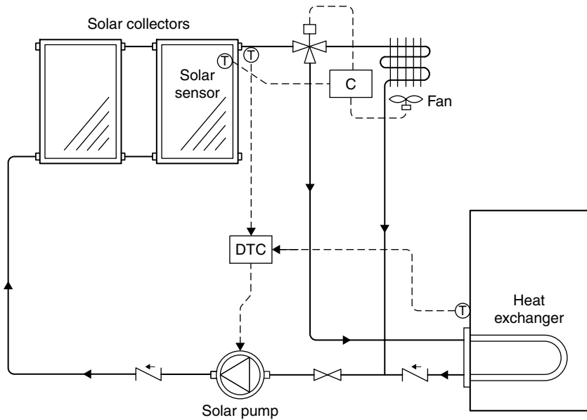
FIGURE 5.28 Heat rejection by a solar heating system using a liquid-to-air heat exchanger.
