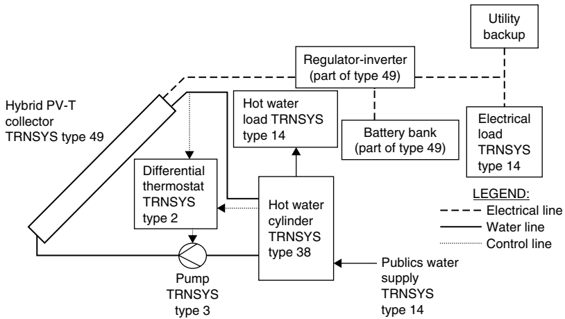
FIGURE 9.25 Hybrid PV/T system schematic.
