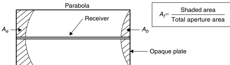
FIGURE 3.39 End effect and blocking in a parabolic trough collector.
