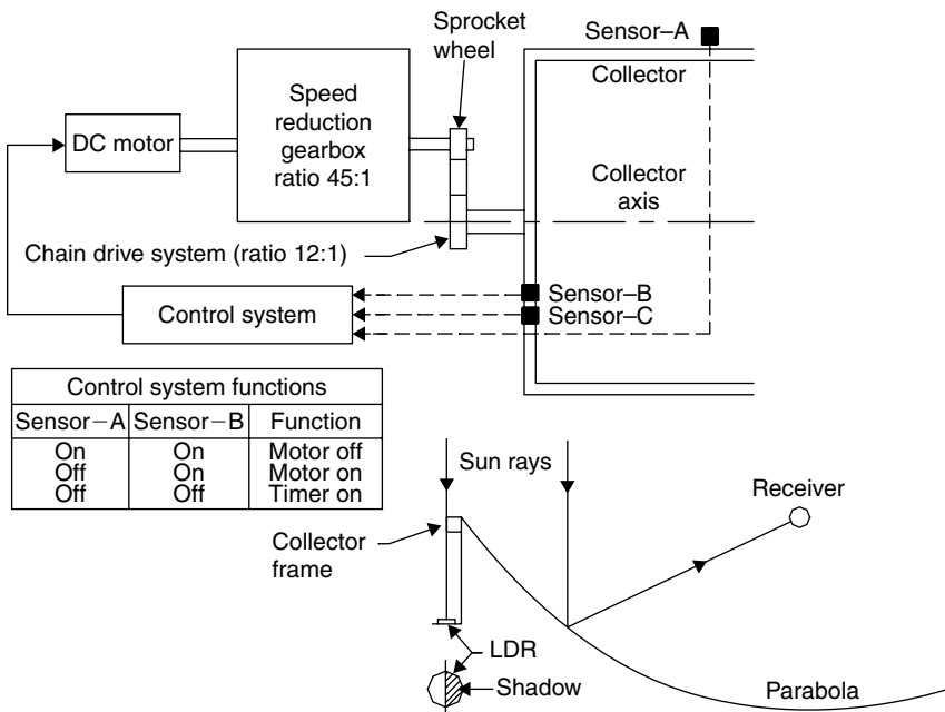
FIGURE 3.16 Tracking mechanism, system diagram.
