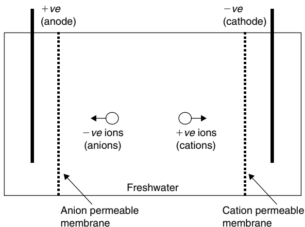
FIGURE 8.11 Principle of operation of electrodialysis (ED).
