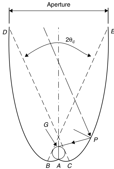
FIGURE 3.33 Schematic diagram of a CPC collector.
