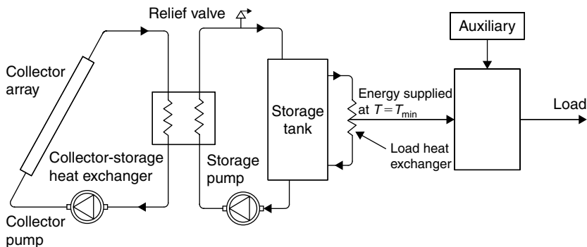
FIGURE 11.10 Schematic diagram of a closed loop solar energy system.
