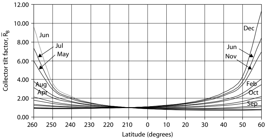
FIGURE A3.7 Values of \bar{R}_B for collector slope equal to latitude +10°.
