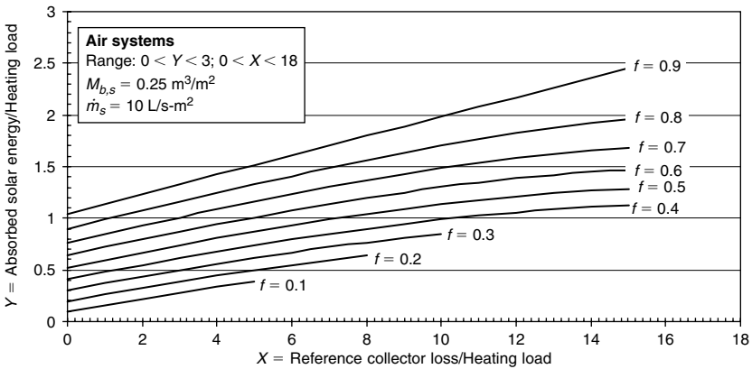
FIGURE 11.6 The f -chart for air-based solar heating systems.
