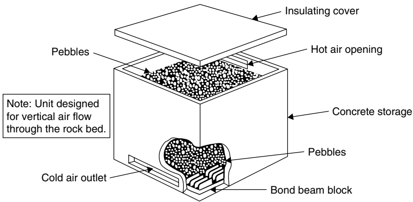
FIGURE 5.15 Vertical flow packed rock bed.
