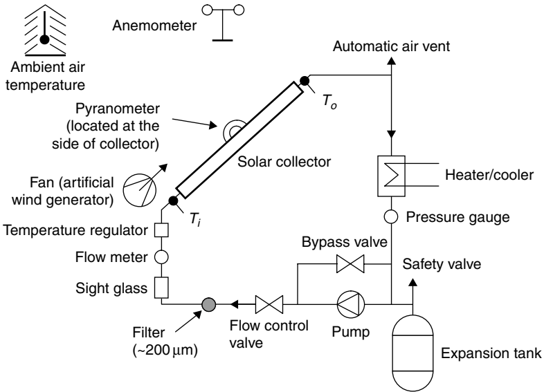
FIGURE 4.1 Closed loop test system.
