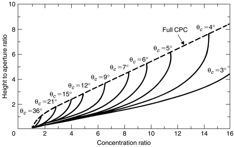
FIGURE 3.35 Ratio of height to aperture for full and truncated CPCs. (Reprinted from Rabl (1976) with permission from Elsevier.)
