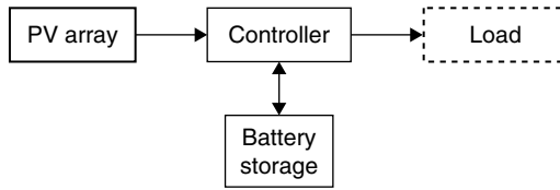
FIGURE 9.15 Basic principle of a solar energy system.
