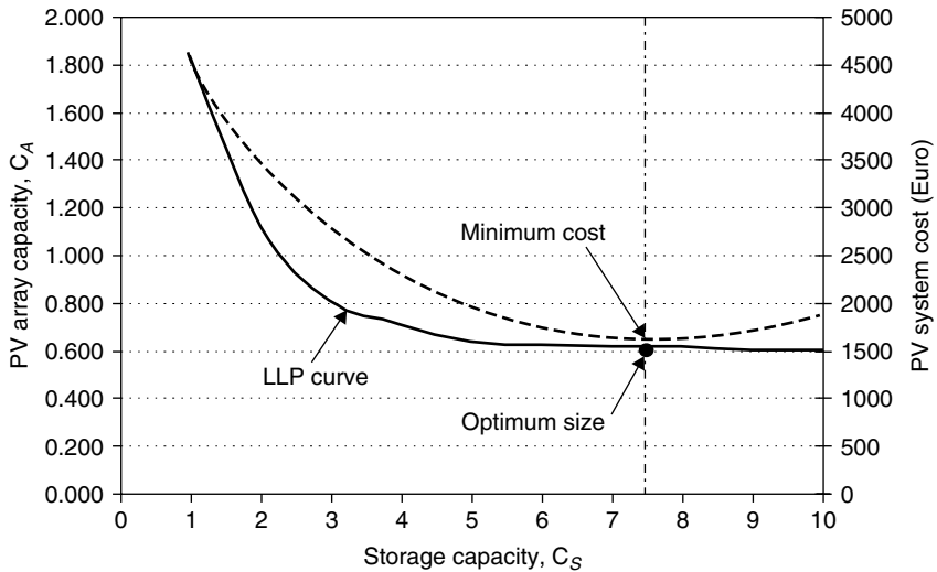
FIGURE 9.21 LLP curve for LLP = 0.01 and cost curve of a PV system.
