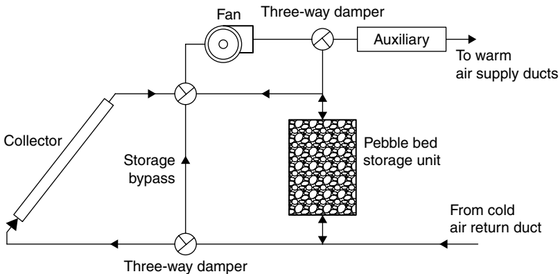
FIGURE 6.11 Schematic of basic hot air system.
