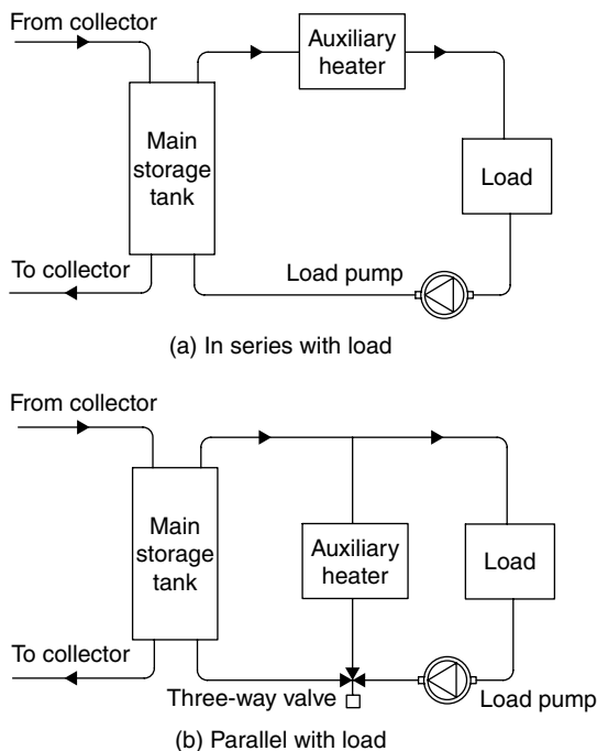
FIGURE 6.15 Auxiliary energy supply in water-based systems.
