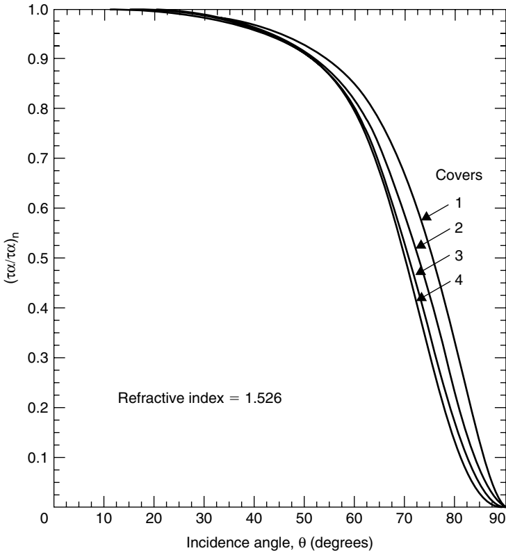
FIGURE 3.24 Typical (\tau\alpha)/(\tau\alpha)_n curves for one to four glass covers. (Reprinted from Klein (1979), with permission from Elsevier.)
