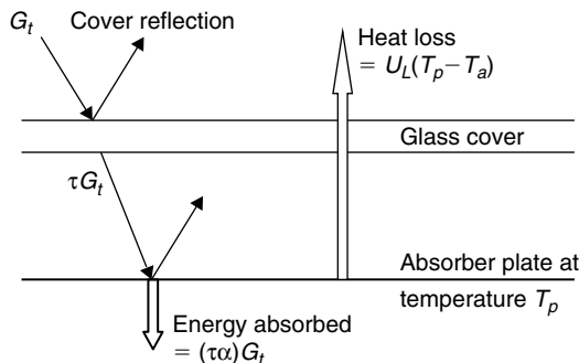
FIGURE 3.26 Radiation input and heat loss from a flat-plate collector.
