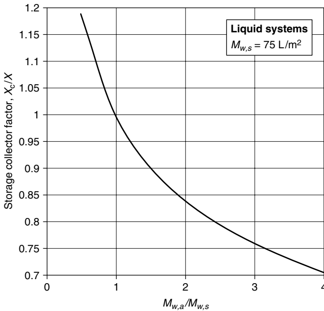
FIGURE 11.3 Storage correction factor for liquid-based systems.
