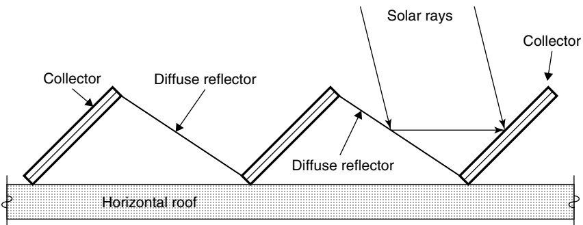
FIGURE 3.12 Flat-plate collectors with saw-toothed reflectors.
