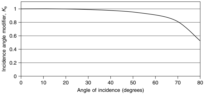
FIGURE 4.5 Incidence angle modified graph.
