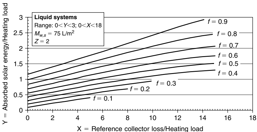
FIGURE 11.2 The f -chart for liquid-based solar heating systems.
