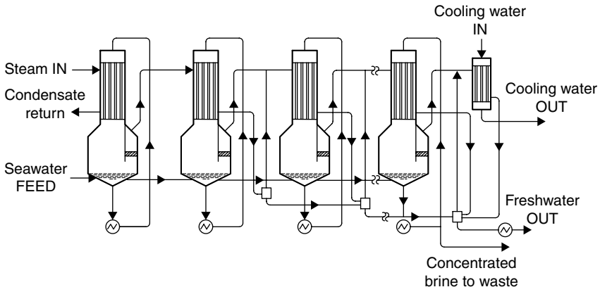
FIGURE 8.7 Long tube vertical MEB plant.
