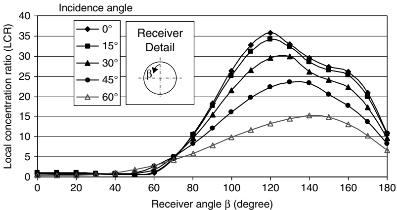
FIGURE 3.40 Local concentration ratio on the receiver of a parabolic trough collector.
