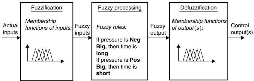
FIGURE 11.22 Operation of a fuzzy controller.
