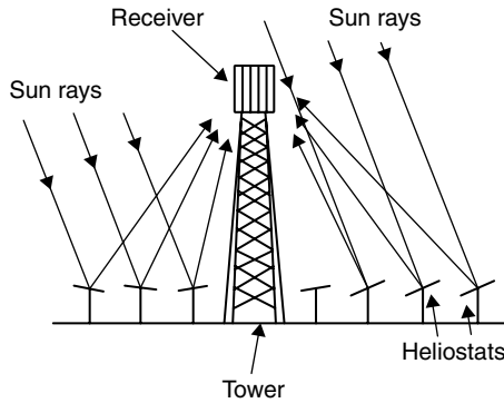
FIGURE 3.21 Schematic of central receiver system.
