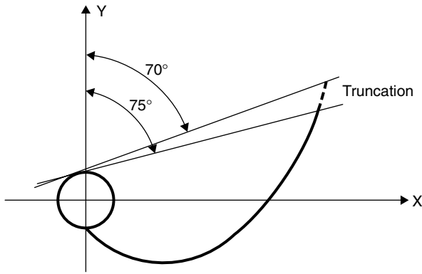
FIGURE 5.7 Truncation of non-imaging concentrator.
