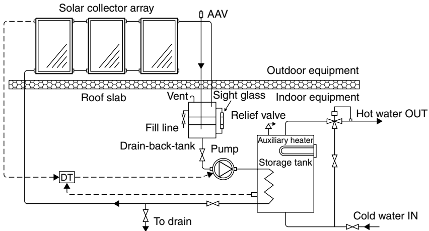
FIGURE 5.13 Drain-back system.
