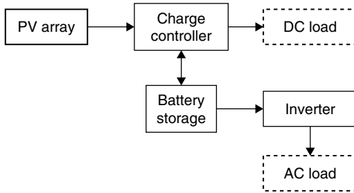
FIGURE 9.17 Schematic diagram of a stand-alone PV application.
