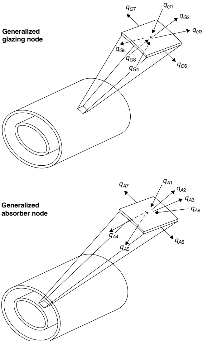
FIGURE 3.43 Generalized glazing and absorber nodes, showing the various modes of heat transfer (Karimi et al., 1986).
