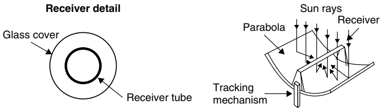
FIGURE 3.13 Schematic of a parabolic trough collector.
