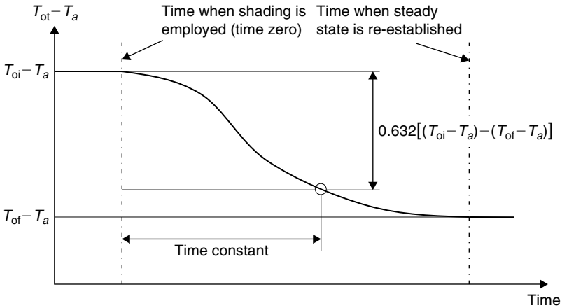
FIGURE 4.10 Time constant as specified in ASHRAE 93:2003.
