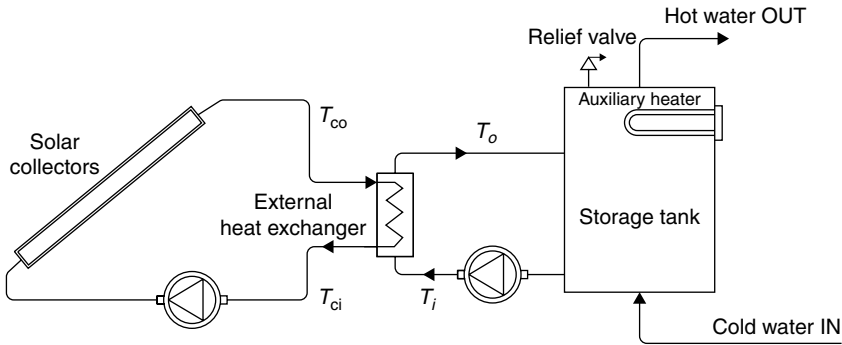
FIGURE 5.27 Schematic diagram of a liquid system with an external heat exchanger between the solar collectors and storage tank.
