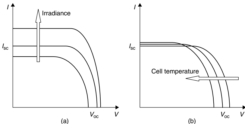
FIGURE 9.9 Influence of irradiation and cell temperature on PV cell characteristics. (a) Effect of increased irradiation. (b) Effect of increased cell temperature.
