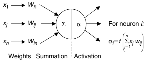
FIGURE 11.18 Information processing in a neural network unit.
