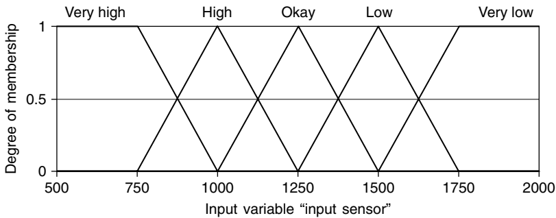
FIGURE 11.24 Membership functions for linguistic variables describing an input sensor.
