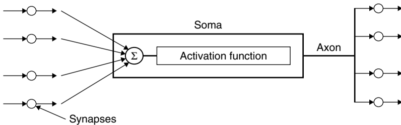
FIGURE 11.16 A simplified model of an artificial neuron.
