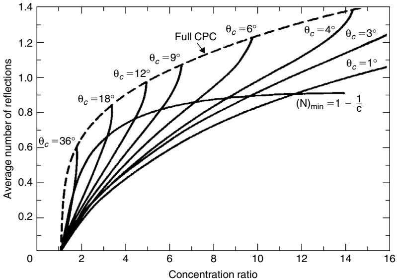
FIGURE 3.34 Average number of reflections for full and truncated CPCs. (Reprinted from Rabl (1976) with permission from Elsevier.)
