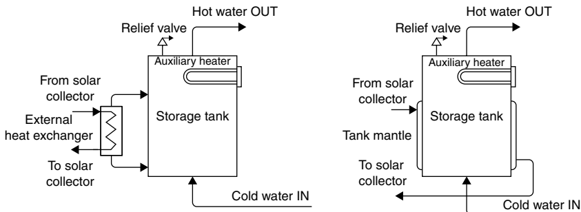
FIGURE 5.12 External and mantle heat exchangers. (a) External heat exchanger. (b) Mantle heat exchanger.
