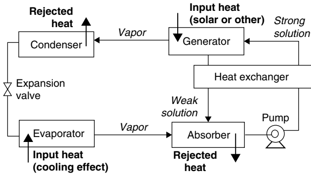
FIGURE 6.22 Basic principle of the absorption air-conditioning system.
