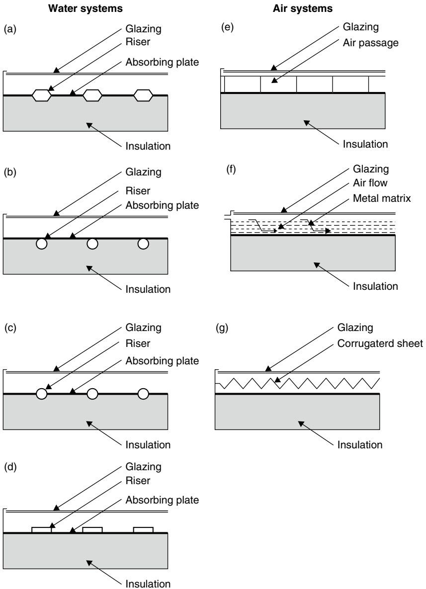
FIGURE 3.3 Various types of flat-plate solar collector absorber configurations for water and air.
