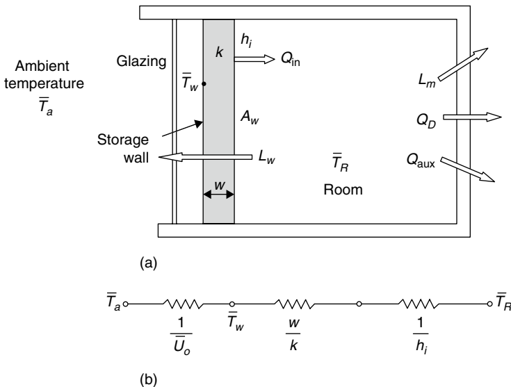
FIGURE 6.5 (a) Schematic of a thermal storage wall. (b) Equivalent electric circuit for the heat flow through the wall.
