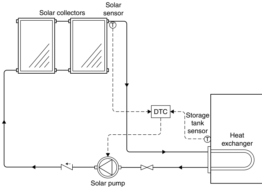
FIGURE 5.29 Basic collector control with a differential temperature controller.
