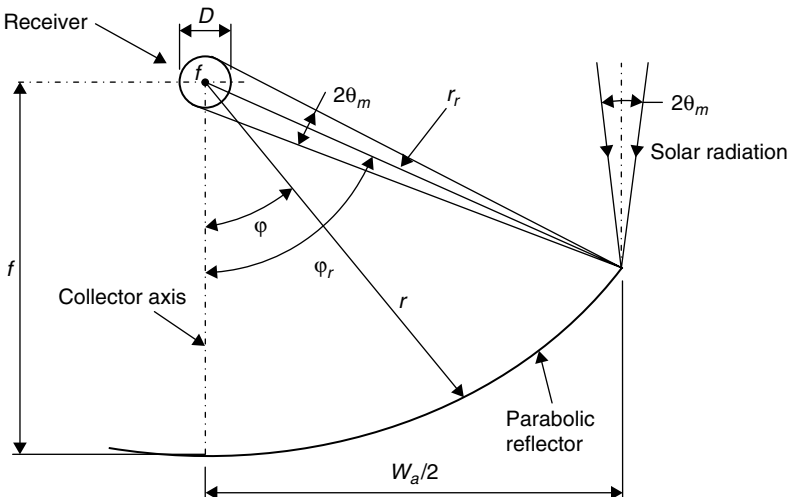
FIGURE 3.37 Cross-section of a parabolic trough collector with circular receiver.
