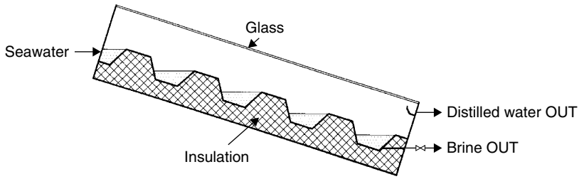
FIGURE 8.3 Schematic of a cascaded solar still.
