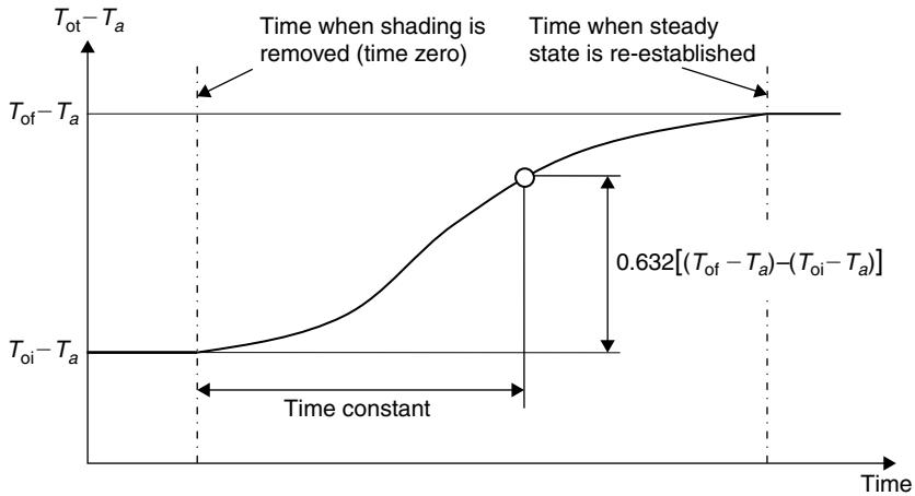
FIGURE 4.9 Time constant as specified in ISO 9806-1:1994.
