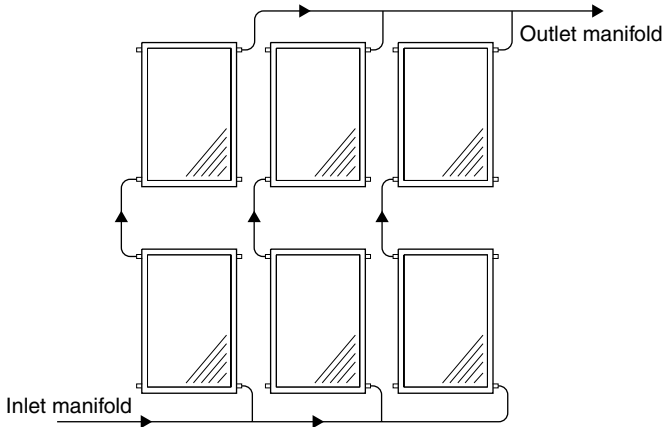
FIGURE 5.21 Collector manifolding arrangement for combined series-parallel flow modules.
