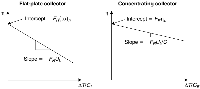
FIGURE 4.3 Typical collector performance curves.
