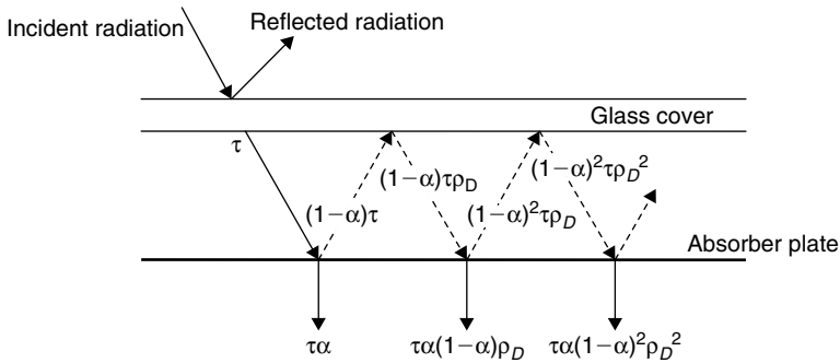
FIGURE 3.23 Radiation transfer between the glass cover and absorber plate.
