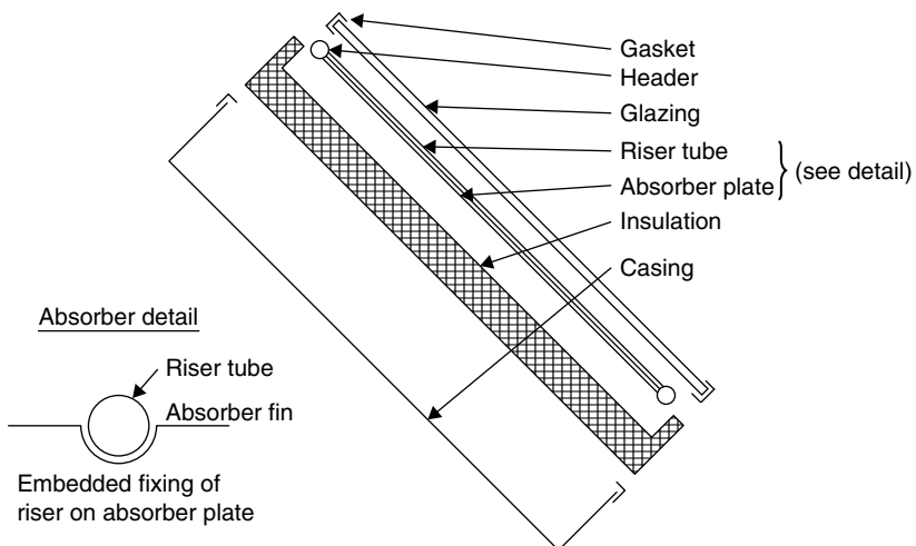
FIGURE 3.2 Exploded view of a flat-plate collector and absorber details.
