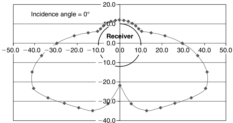
FIGURE 3.41 A more representative view of LCR for a collector with receiver diameter of 20 mm and rim angle of 90°.
