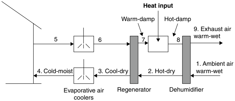
FIGURE 6.19 Schematic of a solar adsorption system.
