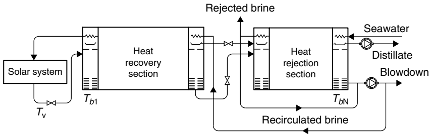
FIGURE 8.5 A multi-stage flash (MSF) process plant.
