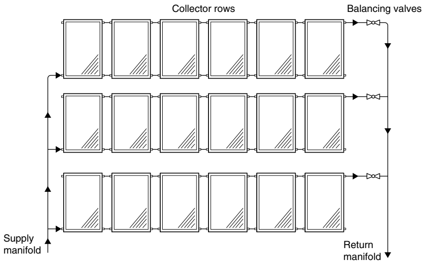
FIGURE 5.22 Direct-return array piping.
