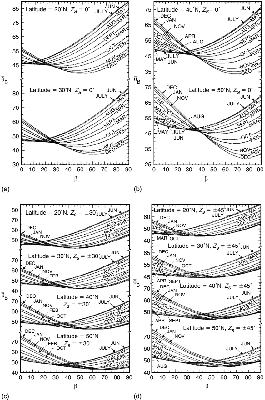
FIGURE A3.8 Monthly average beam incidence angle for various surface locations and orientations (reprinted from Klein, 1979, with permission from Elsevier). Note: For Southern Hemisphere, interchange January with July, February with August, March with September, April with October, May with November, June with December, July with January, August with February, September with March, October with April, November with May, and December with June.
