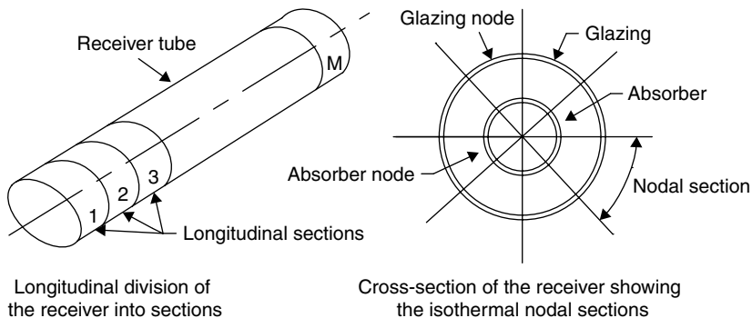
FIGURE 3.42 Piecewise two-dimensional model of the receiver assembly (Karimi et al., 1986).
