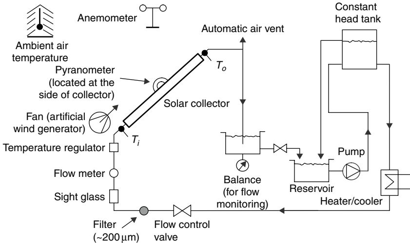
FIGURE 4.2 Open loop test system.
