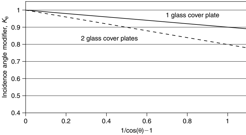
FIGURE 4.6 Plot of incidence angle modifier against 1/\cos(\theta) - 1 for two types of flat-plate collectors.
