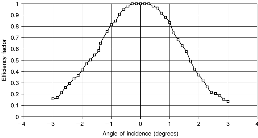
FIGURE 4.8 Parabolic trough collector acceptance angle test results.
