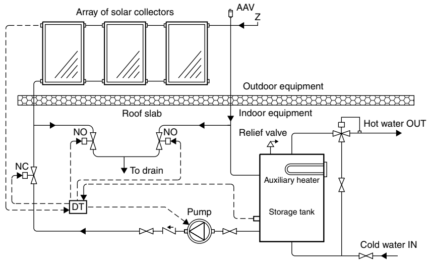
FIGURE 5.10 Drain-down system.
