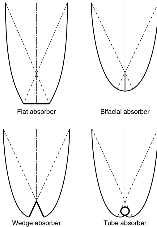
FIGURE 3.5 Various absorber types of CPCs.
