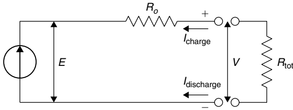
FIGURE 9.13 Schematic diagram of a battery.
