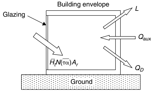
FIGURE 11.11 Monthly energy flows of a direct gain building.
