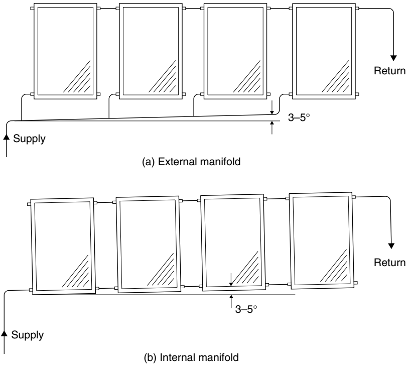
FIGURE 5.24 Mounting for drain-back collector modules.
