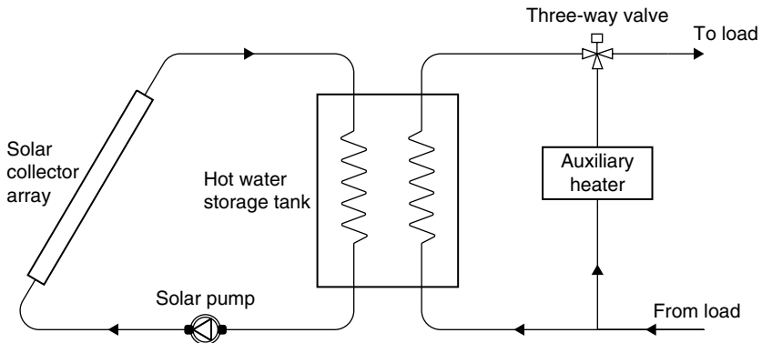
FIGURE 7.3 Simple industrial process heat system with a parallel configuration of auxiliary heater.
