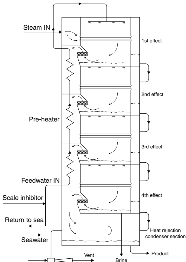
FIGURE 8.8 Schematic of the MES evaporator.
