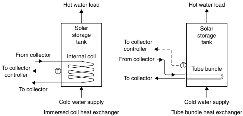
FIGURE 5.16 Pressurized storage with internal heat exchanger.
