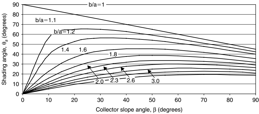
FIGURE 5.26 Graphical solution of collector row shading.
