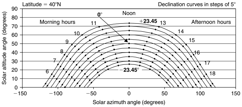
FIGURE A3.3 Sun path diagram for 40°N latitude.
