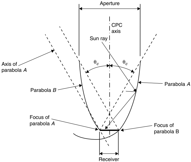
FIGURE 3.32 Construction of a flat-receiver compound parabolic collector.
