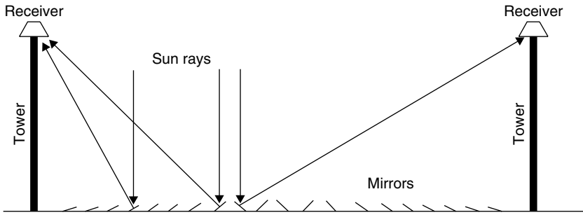
FIGURE 3.19 Schematic diagram showing interleaving of mirrors in a CLFR with reduced shading between mirrors.
