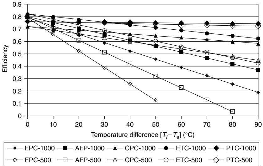
FIGURE 4.4 Comparison of the efficiency of various collectors at two irradiation levels: 500 and 1000 W/m 2 .
