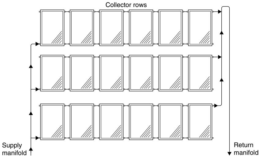
FIGURE 5.23 Reverse-return array piping.
