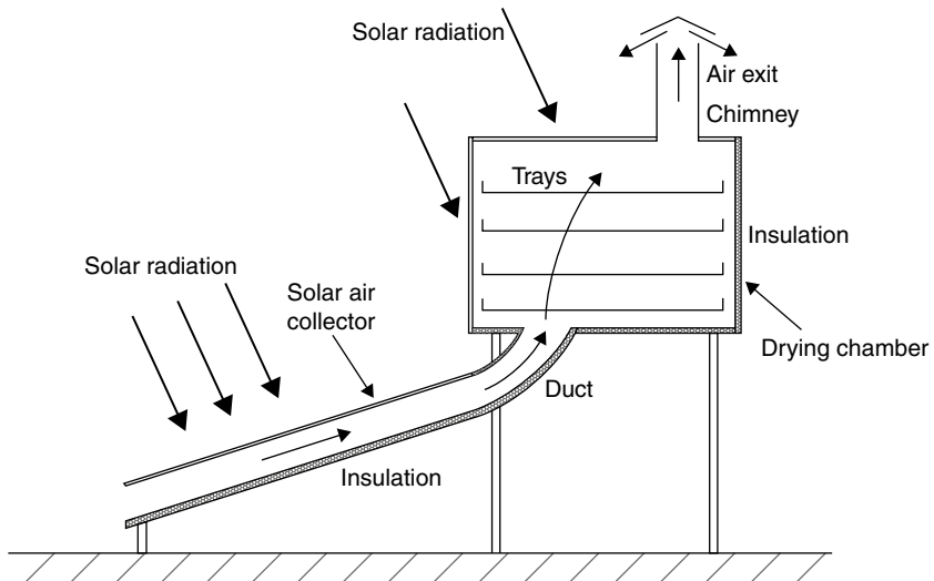
FIGURE 7.16 Schematic diagram of a natural circulation, mixed-mode solar energy dryer.
