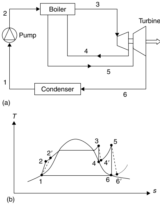
FIGURE 10.10 Reheat Rankine power plant cycle. (a) Reheat Rankine cycle schematic. (b) T-s diagram.
