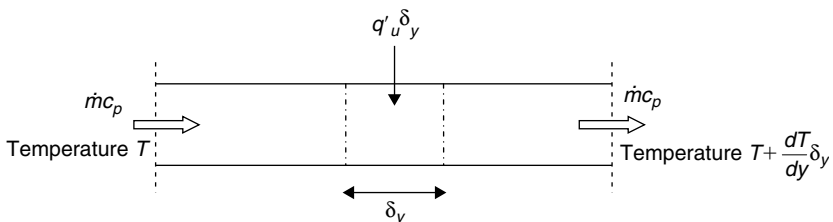
FIGURE 3.28 Energy flow through an element of riser tube.
