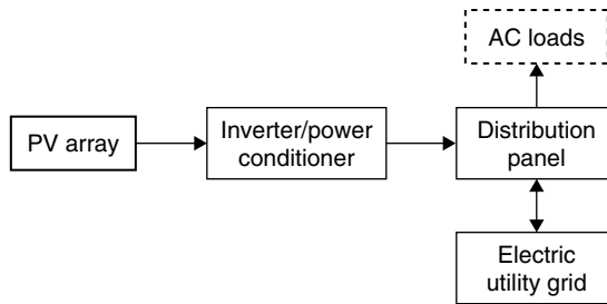
FIGURE 9.18 Schematic diagram of a grid-connected system.
