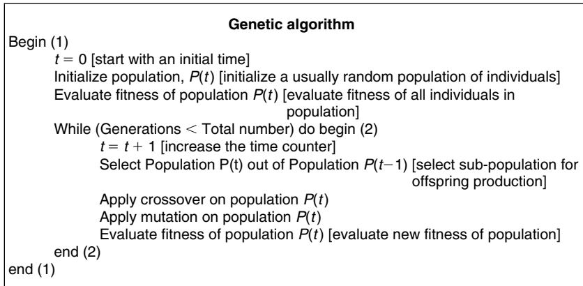
FIGURE 11.21 The structure of a standard genetic algorithm.
