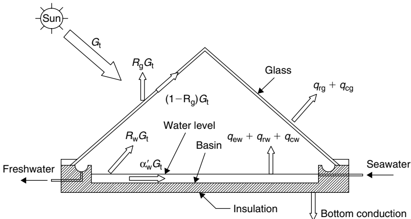
FIGURE 8.1 Schematic of a solar still.
