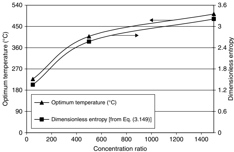
FIGURE 3.46 Entropy generated and optimum temperatures against collector concentration ratio.
