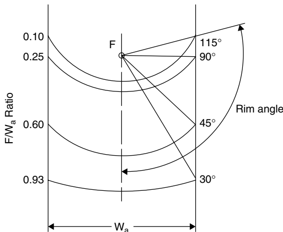
FIGURE 3.38 Parabola focal length and curvature.
