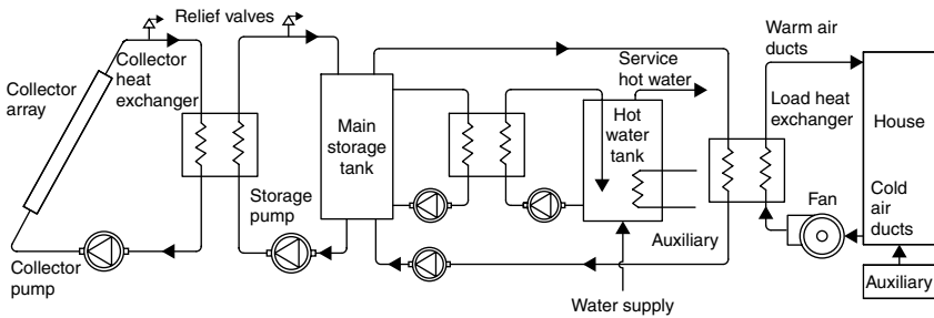
FIGURE 11.1 Schematic diagram of a standard liquid-based solar heating system.
