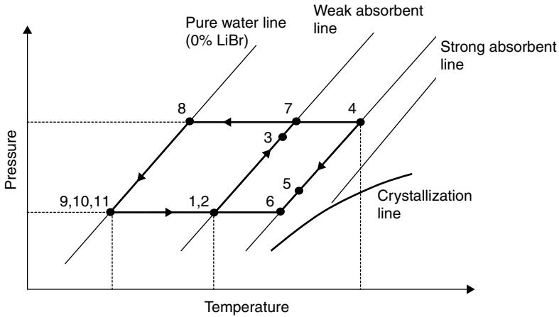
FIGURE 6.25 Dühring chart of the water–lithium bromide absorption cycle.
