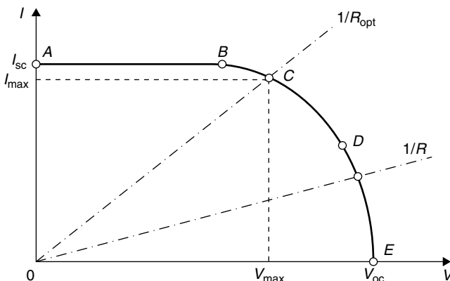
FIGURE 9.7 Representative current-voltage curve for photovoltaic cells.
