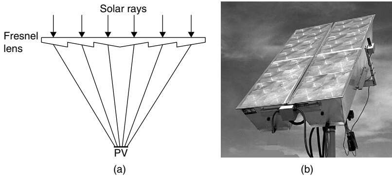
FIGURE 9.22 Schematic diagram and a photograph of a CPV Fresnel system. (a) Schematic diagram. (b) Photograph of an actual system.
