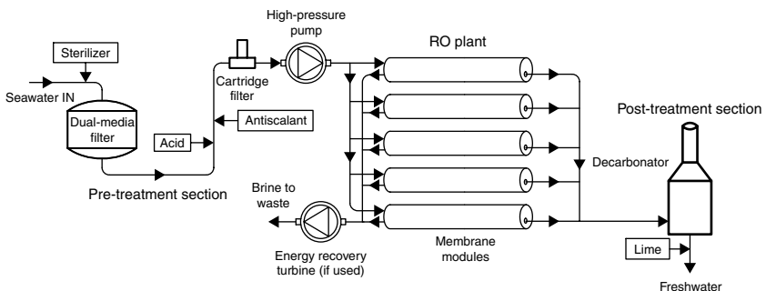
FIGURE 8.10 Principle of operation of a reverse osmosis (RO) system.
