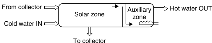
FIGURE 5.3 Configuration of a segmented tank with an insulating baffle.
