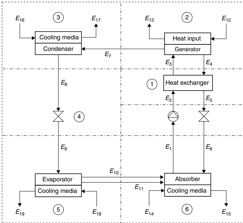
FIGURE 6.26 Availability flow balance of the absorption system.
