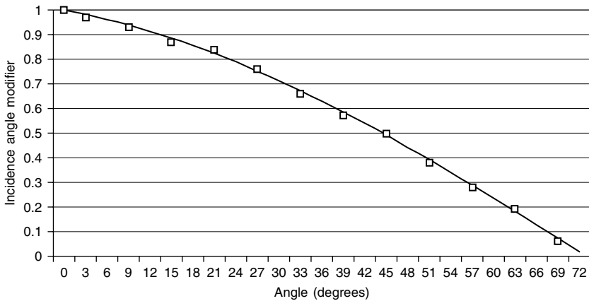
FIGURE 4.7 Parabolic trough collector incidence angle modifier test results.
