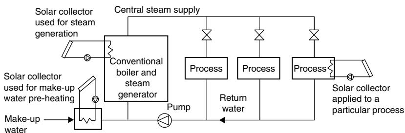
FIGURE 7.1 Possibilities of combining the solar energy system with the existing heat supply.
