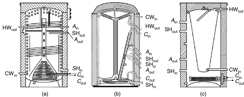
FIGURE 6.10 (a) Immersed heat exchanger, (b) natural circulation heat exchanger, (c) tank-in-tank (adapted from Druck and Hahne, 1998).
