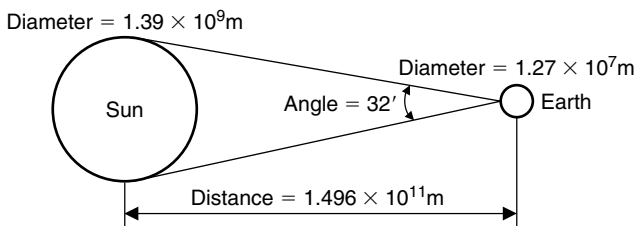
FIGURE 2.1 Sun-earth relationship.
