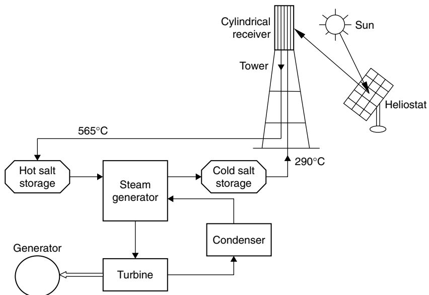
FIGURE 10.5 Schematic of the Solar Two plant.
