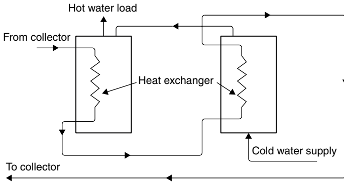
FIGURE 5.17 Multiple-tank storage arrangement with internal heat exchangers.
