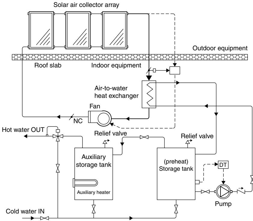
FIGURE 5.14 Air system.
