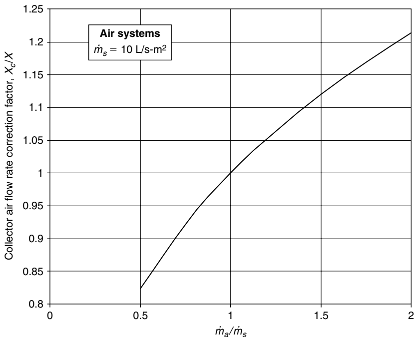
FIGURE 11.8 Correction factor for air flow rate to account for stratification in pebble bed.
