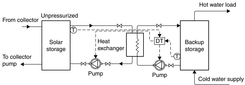
FIGURE 5.19 Unpressurized storage system with external heat exchanger.
