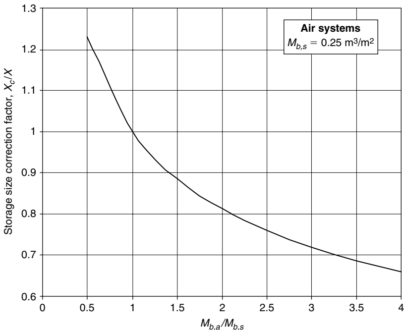
FIGURE 11.7 Storage size correction factor for air-based systems.
