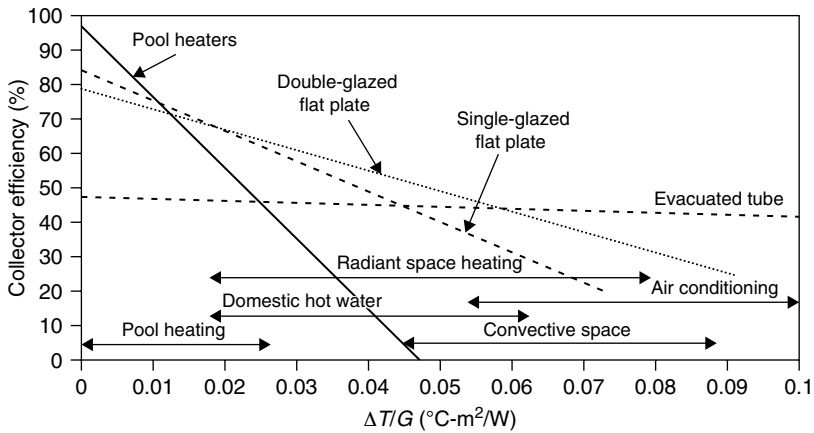
FIGURE 4.11 Collector efficiencies of various liquid collectors.
