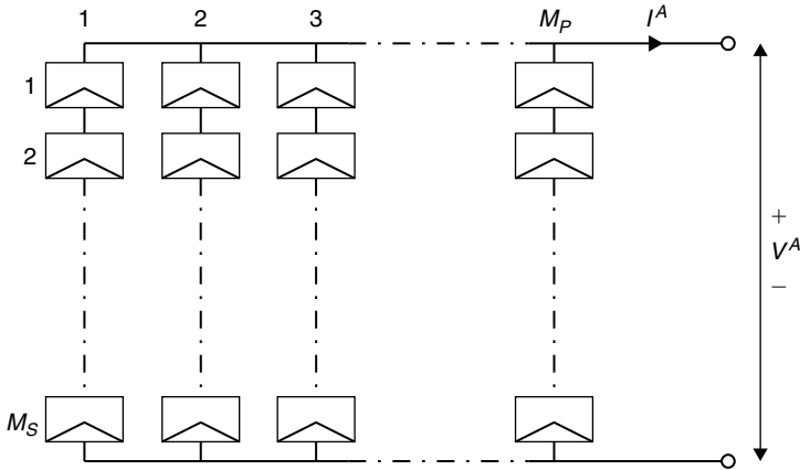
FIGURE 9.12 Cell array consisting of M_p parallel branches, each with M_s modules in series.
