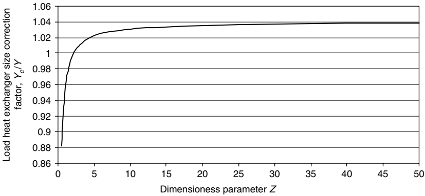
FIGURE 11.4 Load heat exchanger size correction factor.
