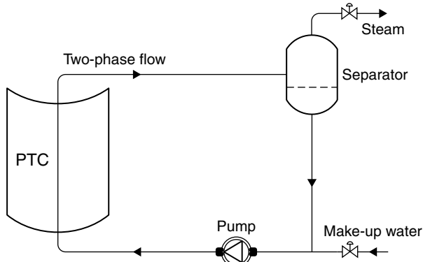
FIGURE 7.6 The direct steam generation concept.
