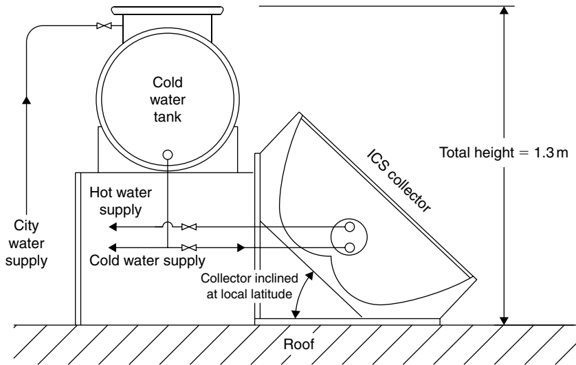
FIGURE 5.8 The complete solar ICS hot water system.
