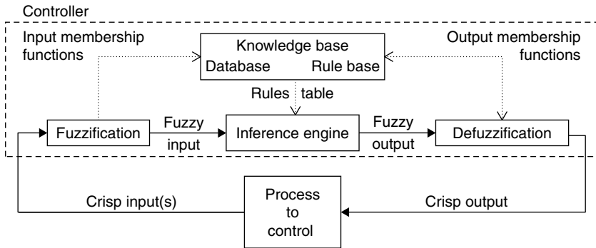
FIGURE 11.23 Basic configuration of fuzzy logic controller.
