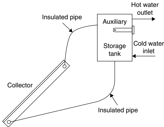
FIGURE 5.1 Schematic diagram of a thermosiphon solar water heater.
