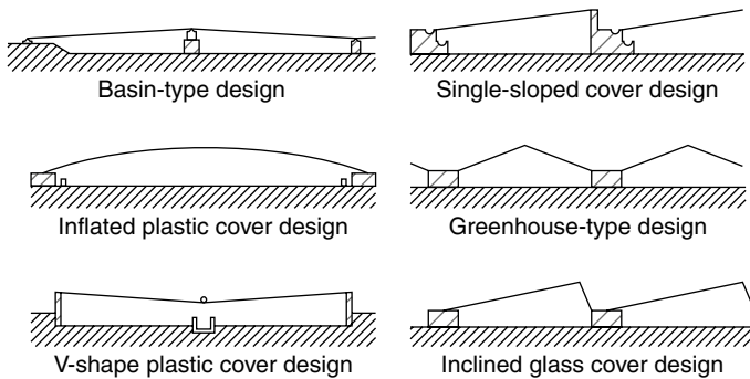
FIGURE 8.2 Common designs of solar stills.
