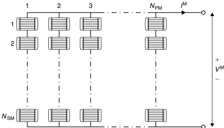
FIGURE 9.11 Schematic diagram of a PV module consisting of N_{PM} parallel branches, each with N_{SM} cells in series.
