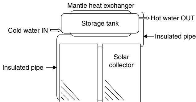
FIGURE 5.4 Mantle heat exchanger concept.
