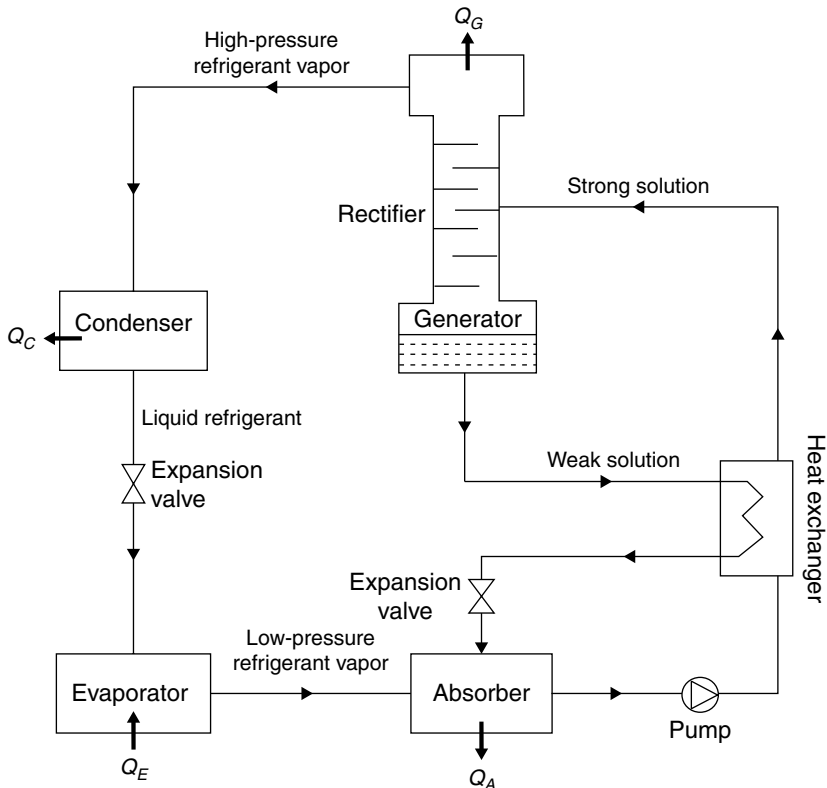
FIGURE 6.27 Schematic of the ammonia-water refrigeration system cycle.
