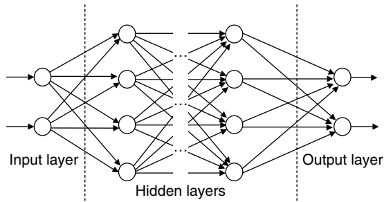
FIGURE 11.17 Schematic diagram of a multilayer feed-forward neural network.
