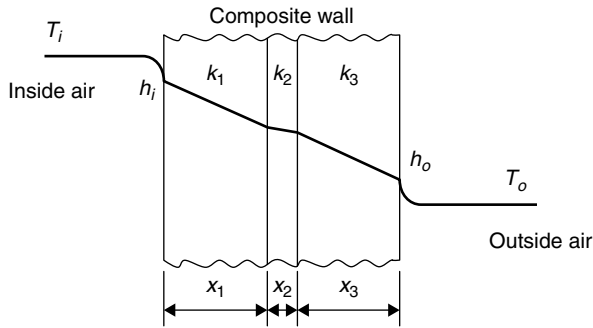
FIGURE 6.2 Multilayer wall heat transfer.
