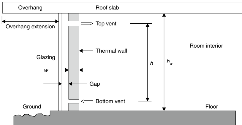
FIGURE 6.4 Schematic of the thermal storage wall.
