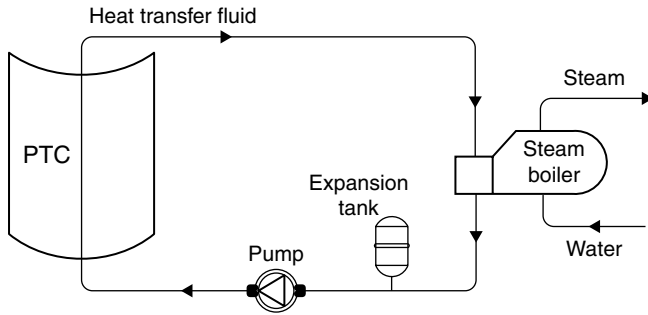
FIGURE 7.7 The unfired boiler steam generation concept.
