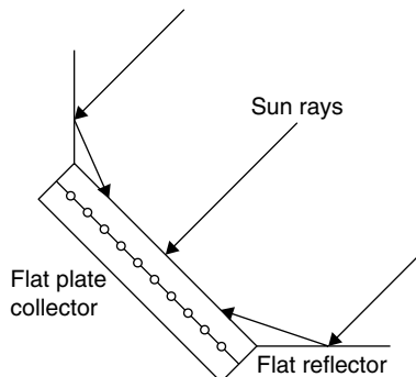
FIGURE 3.11 Flat-plate collector with flat reflectors.
