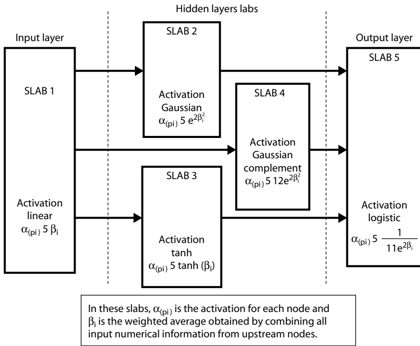
FIGURE 11.19 Feed-forward architecture with multiple hidden slabs.
