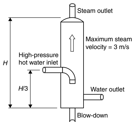
FIGURE 7.8 Flash vessel schematic diagram.
