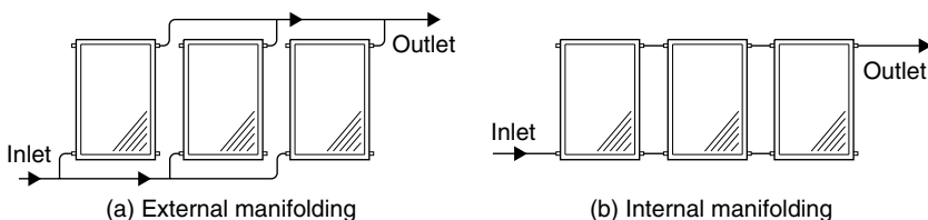
FIGURE 5.20 Collector manifolding arrangements for parallel flow modules.
