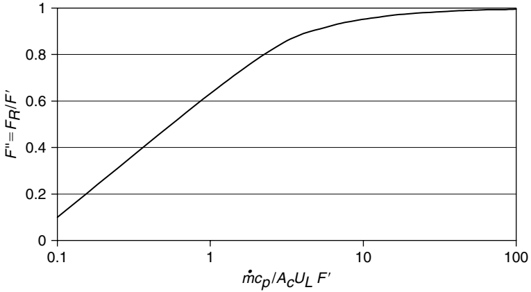
FIGURE 3.29 Collector flow factor as a function of the dimensionless capacitance rate.
