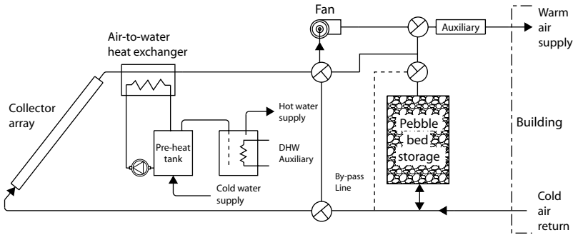
FIGURE 11.5 Schematic diagram of the standard air-based solar heating system.
