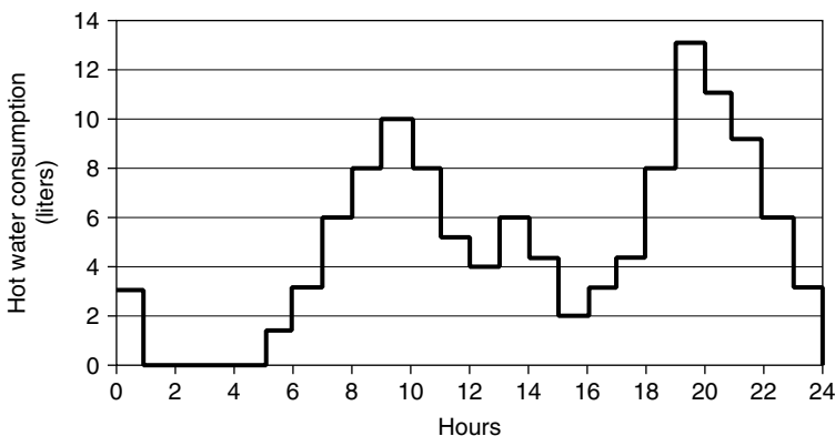
FIGURE 5.31 Hot water daily consumption profile.
