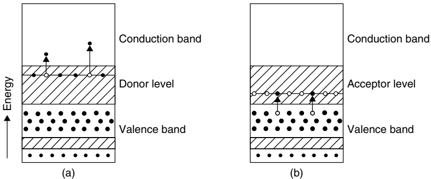
FIGURE 9.4 Energy band diagrams of n- and p-type semiconductors. (a) n-type semiconductor. (b) p-type semiconductor.
