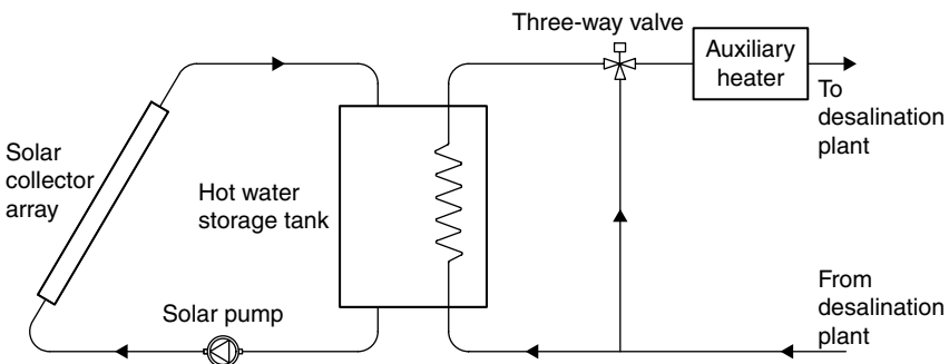
FIGURE 8.12 Connection of a solar system with a desalination system.
