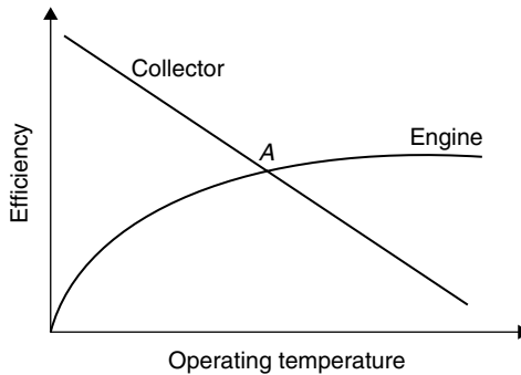
FIGURE 6.18 Collector and power cycle efficiencies as a function of operating temperature.
