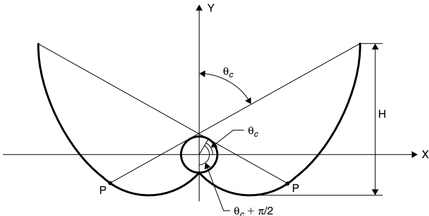
FIGURE 5.5 Fully developed cusp.
