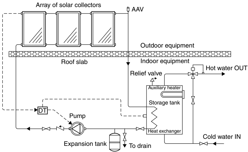
FIGURE 5.11 Indirect water heating system.
