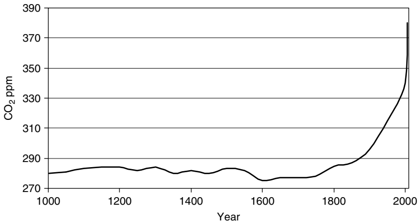
FIGURE 1.3 CO 2 levels in the last 1000 years.
