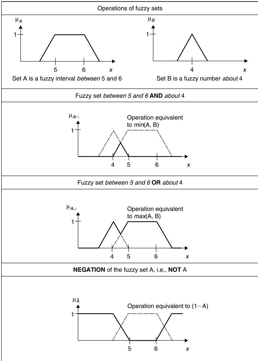
FIGURE 11.26 Operations on fuzzy sets.
