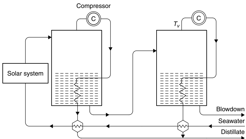
FIGURE 8.9 Principle of operation of a vapor compression (VC) system.
