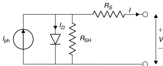
FIGURE 9.6 Single solar cell model.
