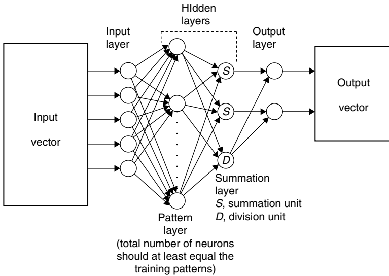
FIGURE 11.20 General regression neural network architecture.
