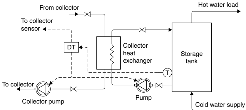
FIGURE 5.18 Pressurized storage system with external heat exchanger.
