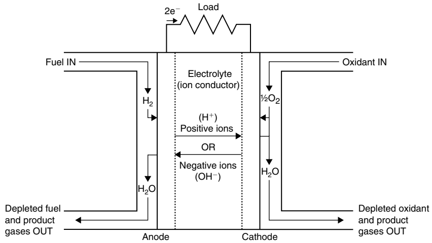
FIGURE 7.9 Schematic diagram of a fuel cell.
