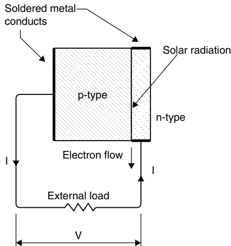
FIGURE 9.5 Photovoltaic effect.
