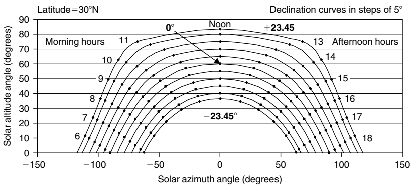
FIGURE A3.2 Sun path diagram for 30°N latitude.
