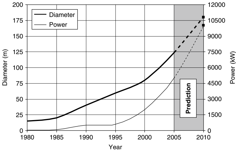
FIGURE 1.8 Evolution of wind turbine rotor diameter and power between 1980 and 2010.
