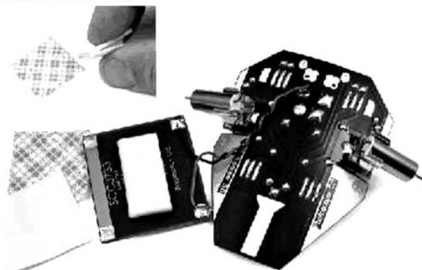
Figure 16-18 Attaching the solar cell. Image courtesy Solarbotics.
