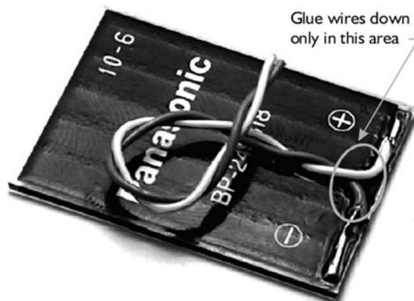
Figure 15-14 Step 9— assembling the Solarroller . Image courtesy Solarbotics.
