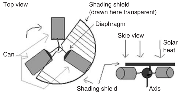
Figure 12-12 Diagram of the radial can engine.
