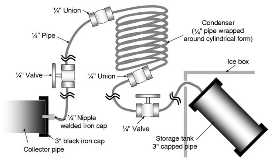
Figure 5-4 Solar cooler plumbing details.
