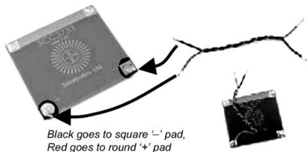
Figure 16-16 Connecting the solar cell. Image courtesy Solarbotics.
