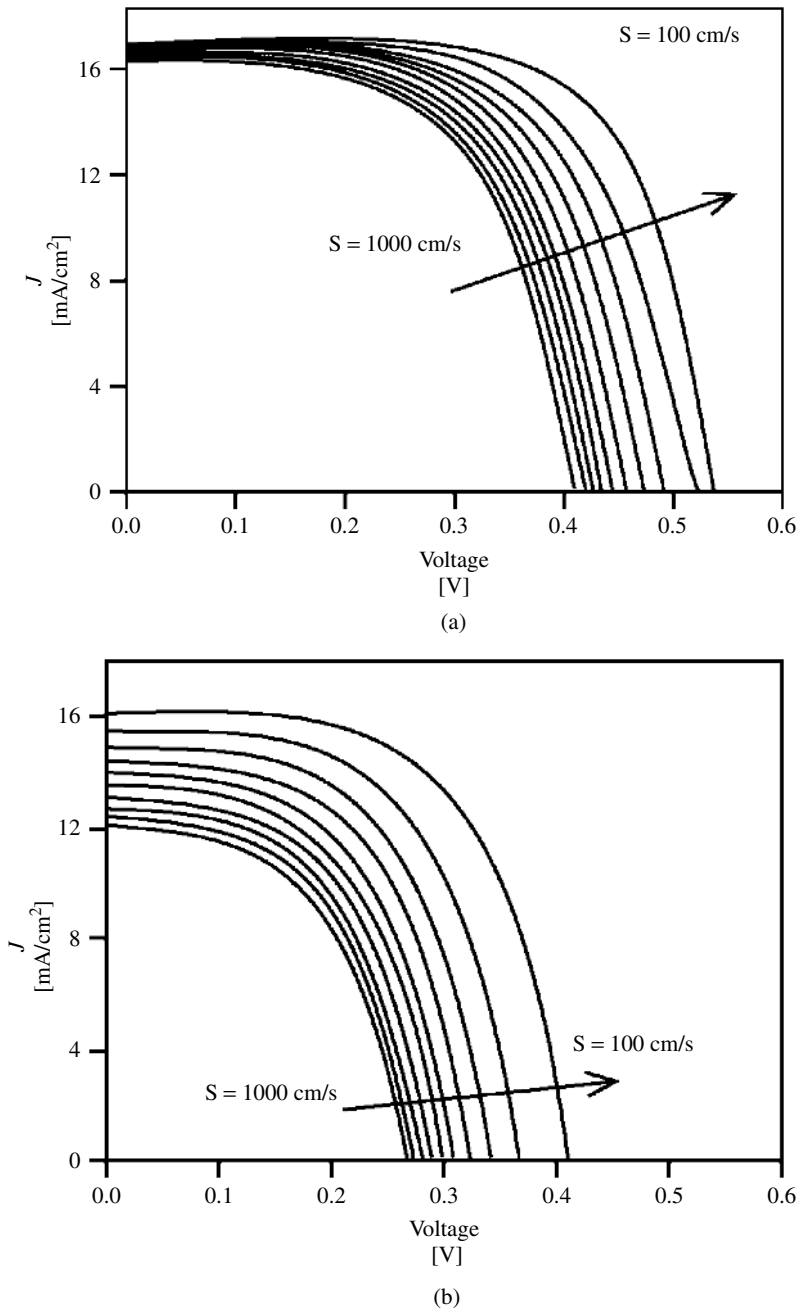
Figure 8.25 The calculated J - V curves for different grain boundary interface recombination velocities ( S ). In the figures, S changes from 1000 \text{cm}/\text{s} to 100 \text{cm}/\text{s} in steps of 100 \text{cm}/\text{s} . Other parameters are given in Table 8.4. The grain sizes used in the calculations are: (a) 5 \mu\text{m} ; (b) 0.5 \mu\text{m} [19]
