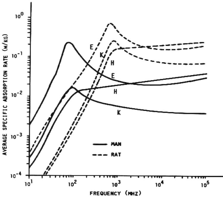
Figure 10 Average SAR (W/kg) vs. frequency (MHz)
