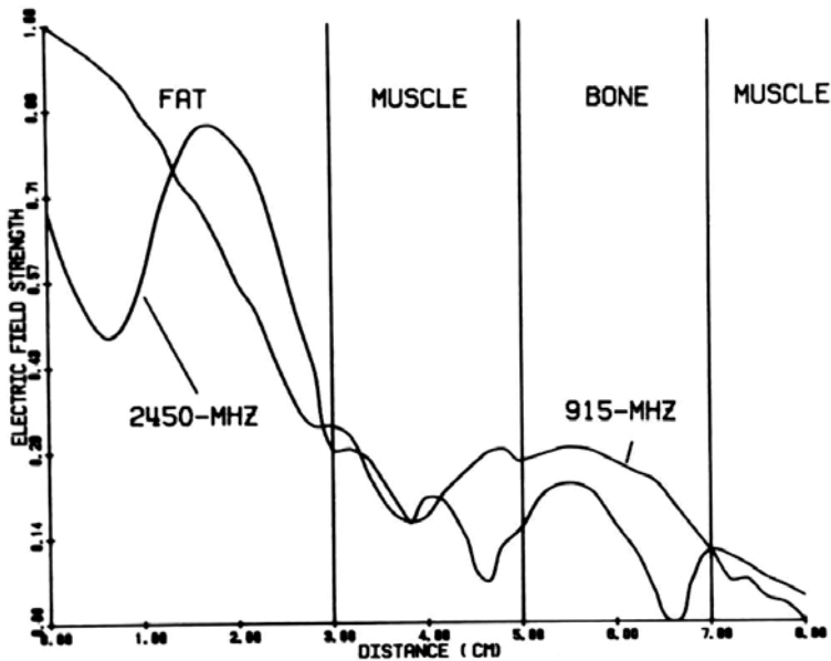
Figure 4 Attenuation of E-field through 8 cm of bodily tissue
