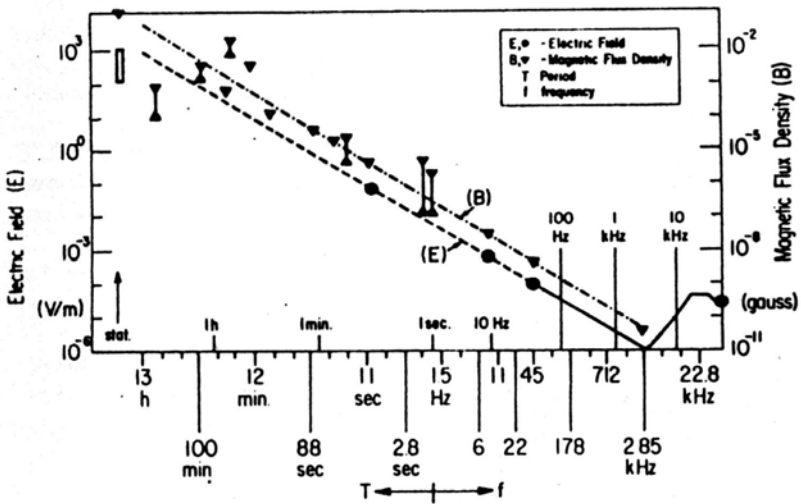
Figure 13 Earth Schumann cavity E and B fields from 0 to 50 kHz
