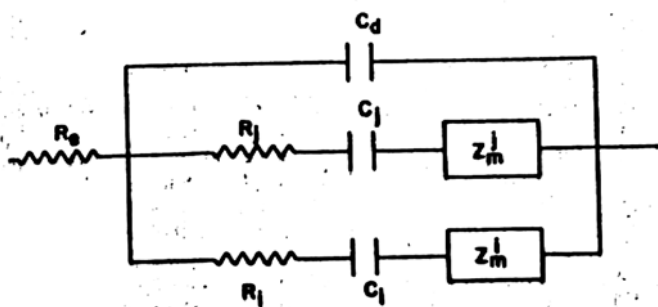
Equivalent circuit for cell membrane
