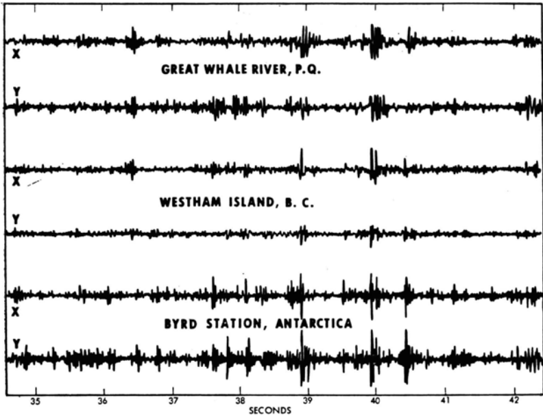
Fig. 12 Earth micropulsations (2 -- 30 Hz) recorded simultaneously. Source: Galejs, Terrestrial Propagation of Long Electromagnetic Waves , Pergamon Press, 1972
