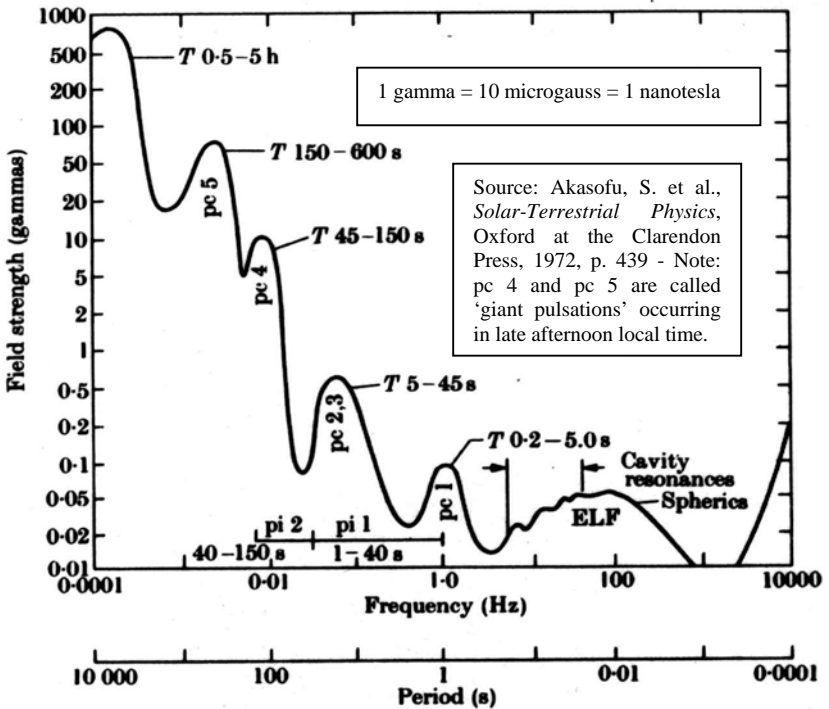
Figure 14 Geomagnetic pulsations of earth-ionosphere cavity
