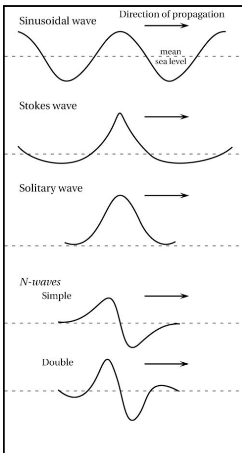
Figure 2.4. Idealized forms characterizing the cross-section of a tsunami wave. Based on Geist (1997b). Note that the vertical dimension is greatly exaggerated.
