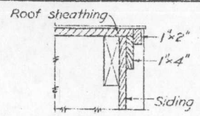
SECTION J-J
