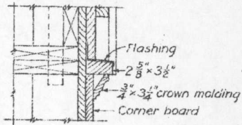
SECTION S-S
