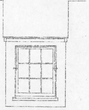
EXTERIOR ELEVATION Scale \frac{1}{2} " = 1'-0"
