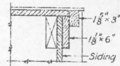
SECTION T-T
