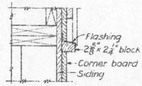
SECTION I-I
