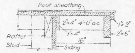
SECTION F-F
