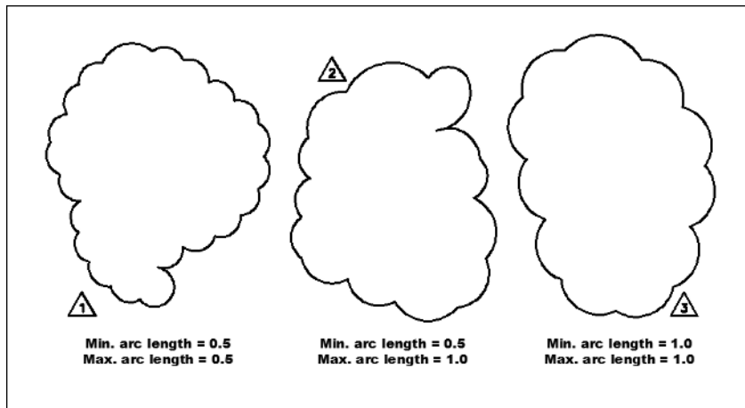
Figure 6-11: Cloud cover.
