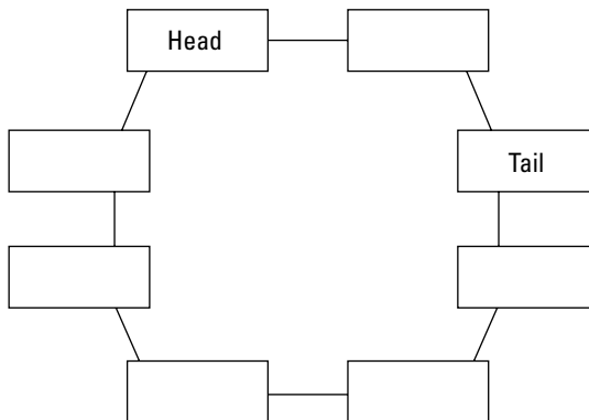
Figure 11-12: When you read an item, the head advances.
