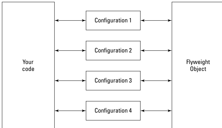
Figure 5-5: Using a flyweight object.
