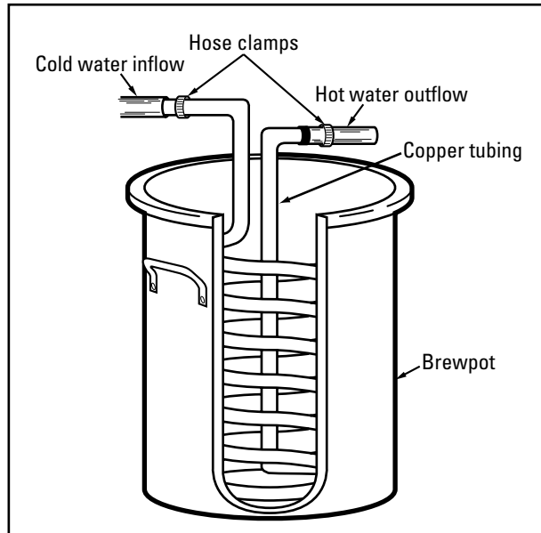
Figure 12-2: An immersion wort chiller, shown here in a brewpot, works like a reverse radiator.
