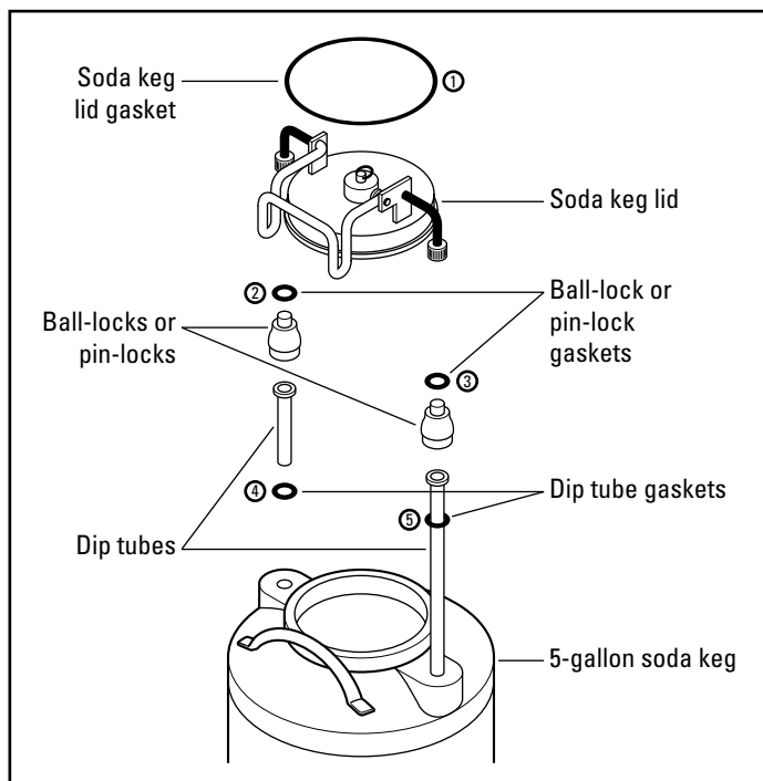
Figure 14-2: Locations of the five rubber gaskets on a typical soda keg.
