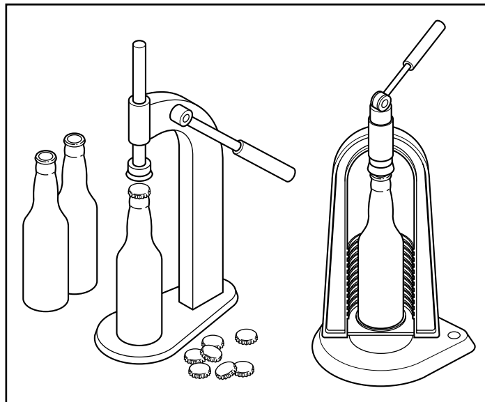
Figure 2-3: You can attach a bench-type bottle capper to a work surface for easy use.
