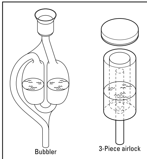
Figure 2-2: An airlock allows carbon dioxide to escape from the fermenter.
