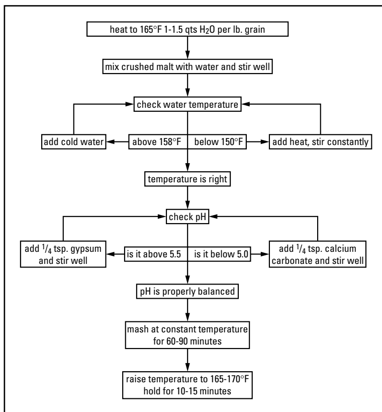
Figure 12-1: Just follow the arrows for a perfect infusion- mashing procedure.
