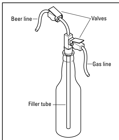
Figure 13-2: Typical counterpres- sure bottle filler setup.
