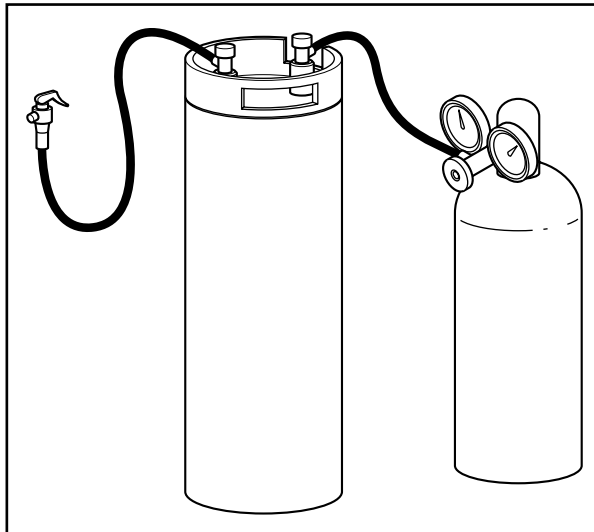
Figure 14-1: The typical soda keg setup for homebrewers, including a 5-gallon keg, CO 2 tank, dual CO 2 gauges, and dispensing hoses and fittings.
