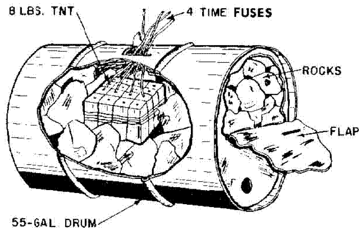
Figure 19 (UNCLASSIFIED). North Korean oil-drum mine (U).
