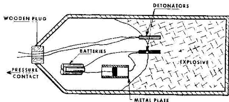
Figure 24 (UNCLASSIFIED). FN ontillift mine (U).
