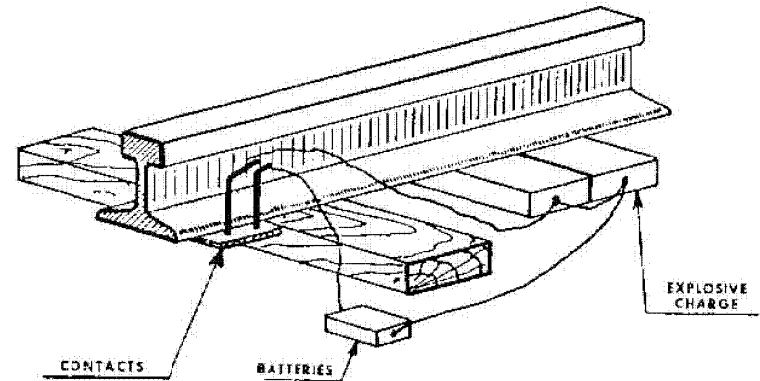
Figure 32 (UNCLASSIFIED). FN wheel-flange firing device (U).
