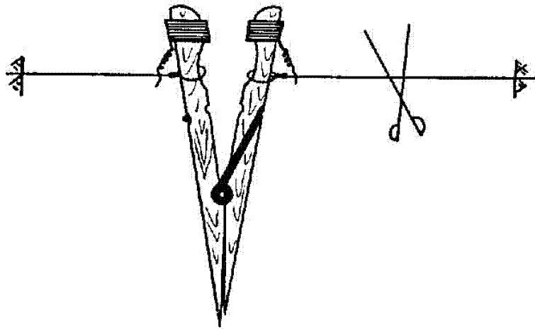
Figure 30 (UNCLASSIFIED). FN clotheshpin firing device (tension-release-operated) (U).
