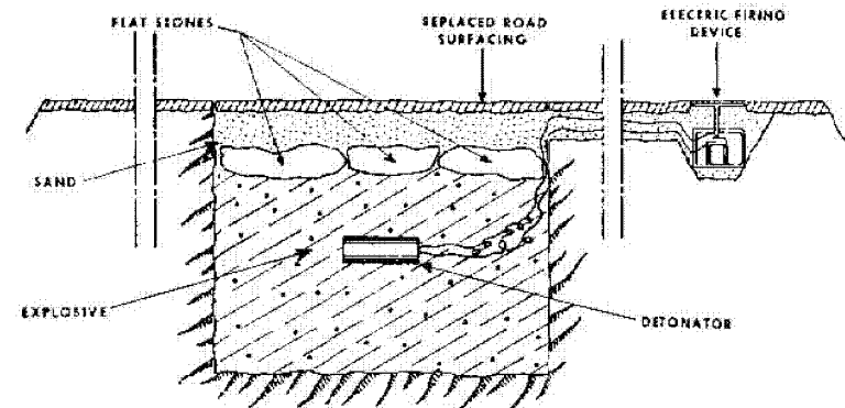
Figure 23 (UNCLASSIFIED). FLM antivehicle mine (U).
