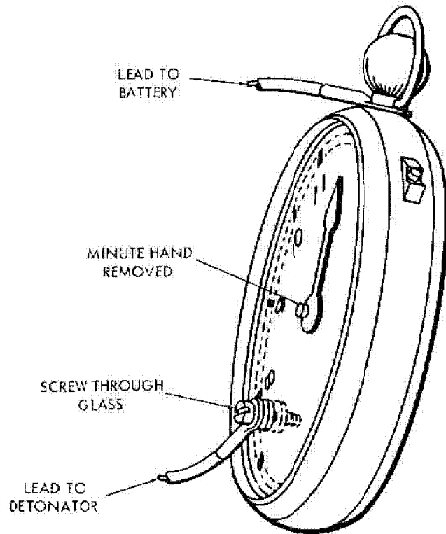
Figure 37 (UNCLASSIFIED). German pocket watch delay. (U).
