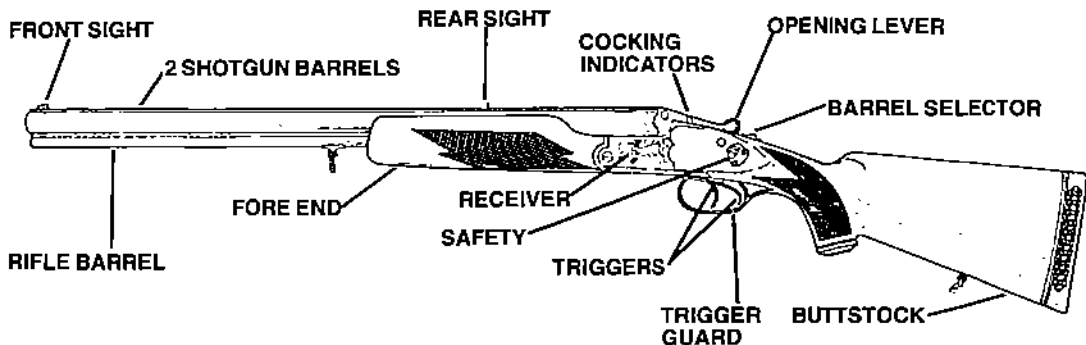
FIGURE 2—COLT SAUER DRILLING FEATURES
