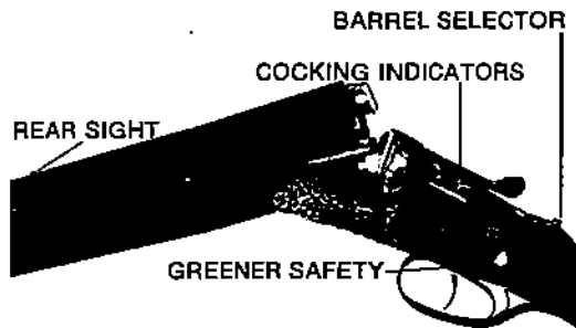
FIGURE 6—ACTION OPEN
