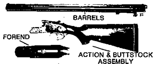
FIGURE 5—MAIN COMPONENT PARTS
