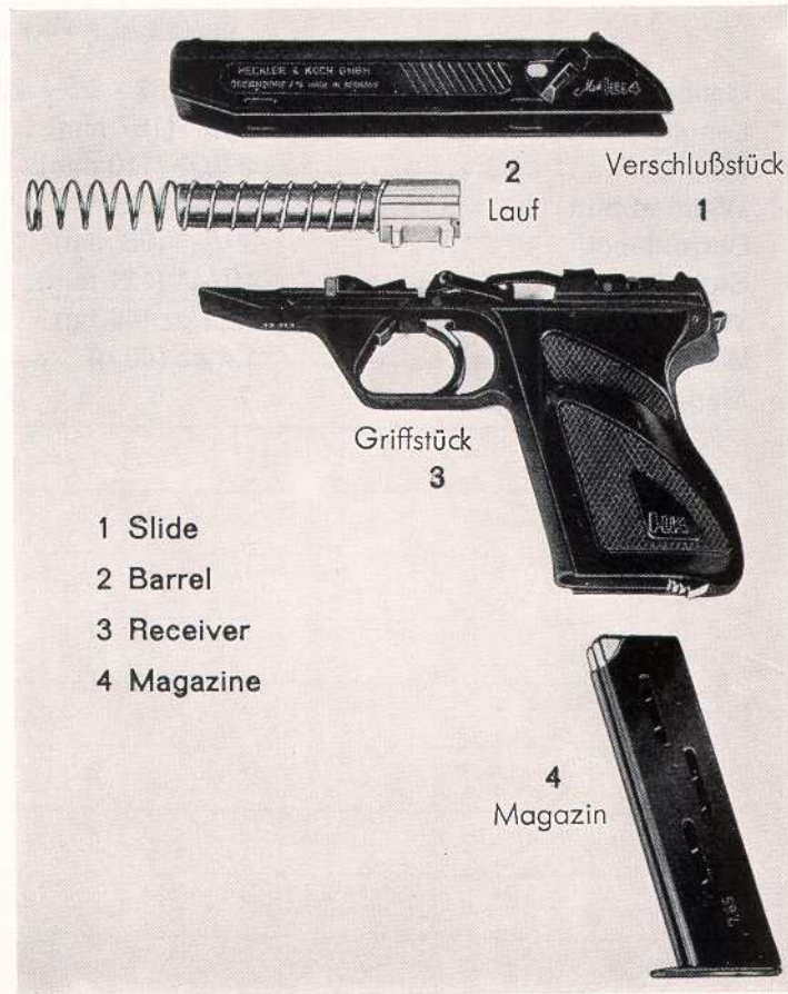
Fig. 18: Pistol stripped for cleaning
