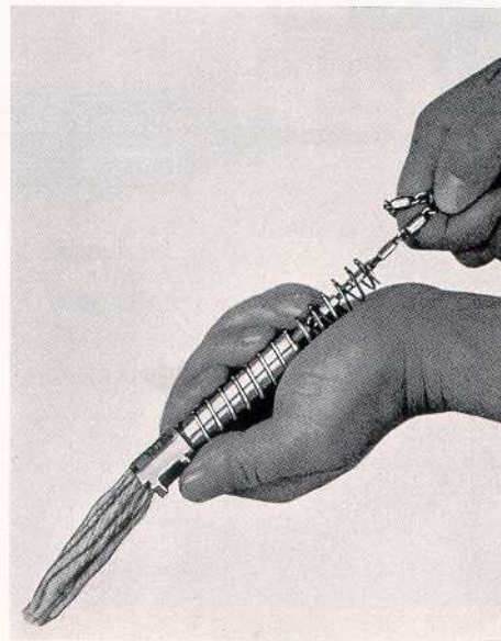
Fig. 16: Clean barrel
