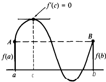
FIGURE 4.10 Geometric interpretation of Rolle's theorem.
