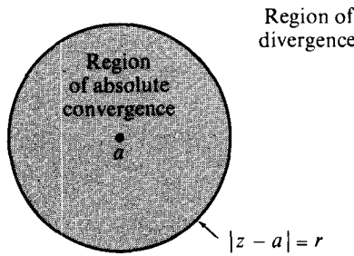
FIGURE 11.4 The circle of convergence of a power series.
