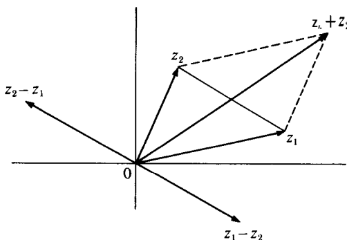
FIGURE 9.2 Addition and subtraction of complex numbers represented geometrically by the parallelogram law.
