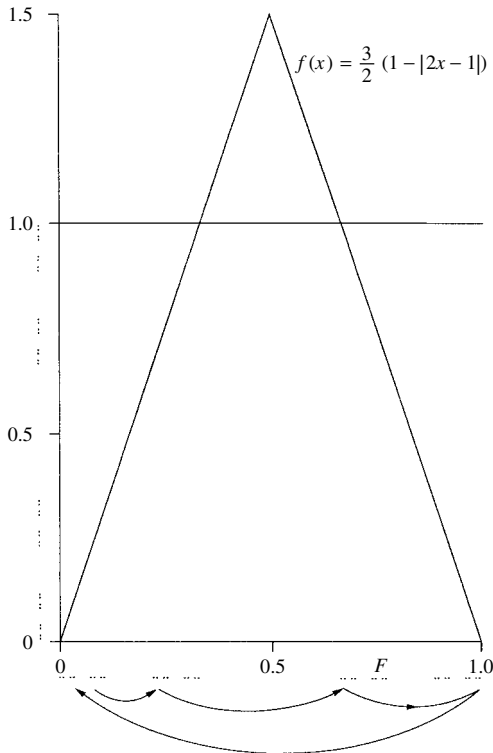
Figure 13.1 The tent map f . Notice that the middle third Cantor set F is mapped onto itself by f and is an invariant repeller. Notice, also, the chaotic nature of f on F : the iterates of a point are indicated by the arrows
