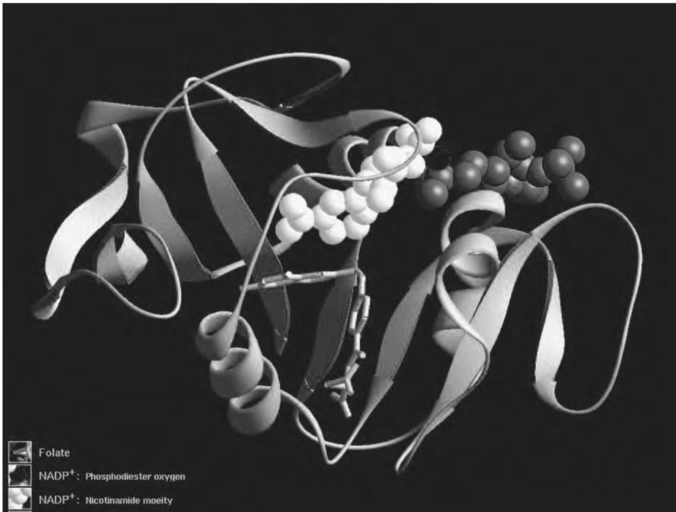
Computer image of a protein molecule, showing regions of different three-dimensional shape.
