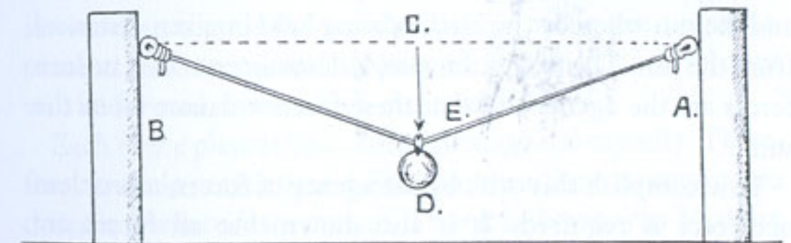
Action of sun's forces on magnetic needle
