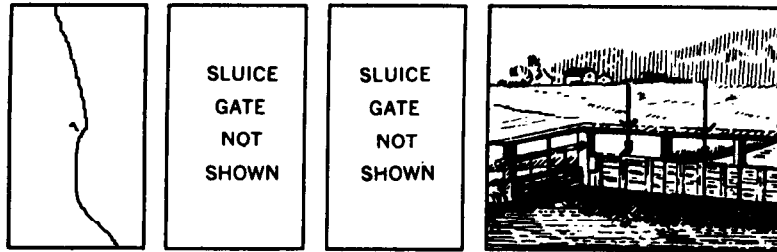
Figure 192. Sluice Gate or Small Canal Lock. The angle of the symbol always points upstream.
