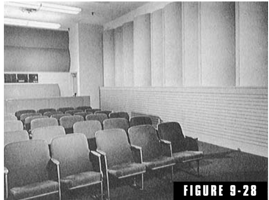
Finished poly array of Fig. 9-26 mounted on the wall above a low-frequency absorber structure. Note that the axes of the polys on the rear wall are perpendicular to the axes of the polys on the other wall. (Moody institute of Science photo, reprinted with permission of Journal of the Audio Engineering Society . 21 )
