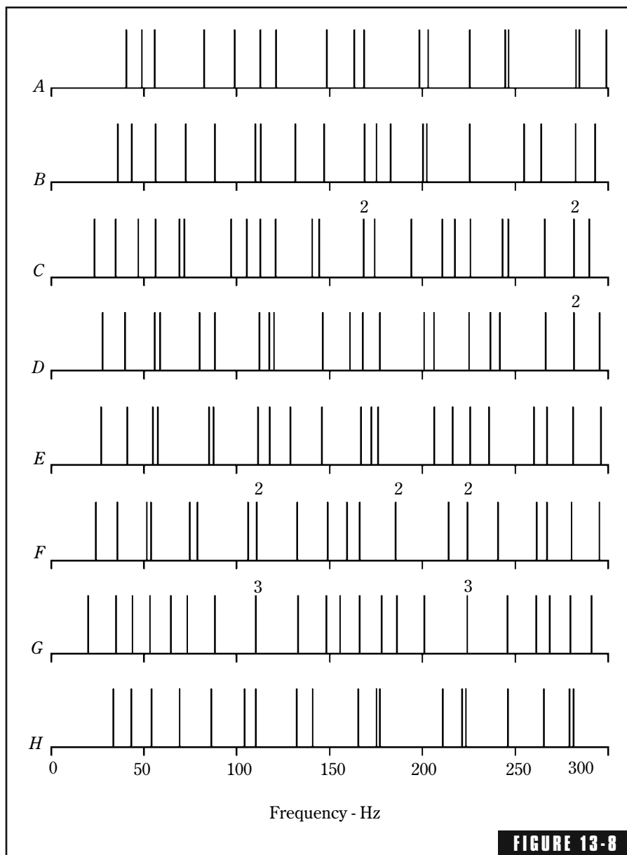
Plots of axial mode distribution for the eight “best” room proportions of Table 13-2. The small numbers indicate the number of modes coincident at those particular frequencies. A room height of 10 ft is assumed.
