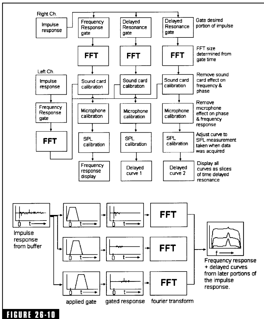
Block diagram of ETF 5's time slice frequency response computation methodology. (Courtesy of Doug Plumb, AcoustiSoft.)
