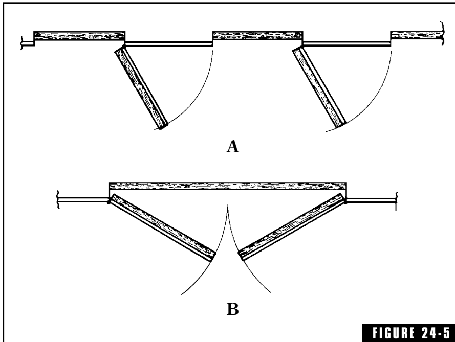
An inexpensive and effective method of incorporating variability in room acoustics is through the use of hinged panels, hard on one side and absorbent on the other.
