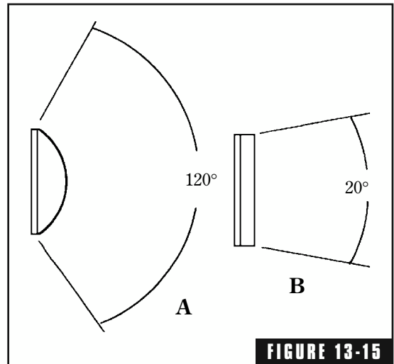
(A) A polycylindrical diffusor reradiates sound energy not absorbed through an angle of about 120^\circ . (B) A similar flat element reradiates sound in a much smaller angle.
