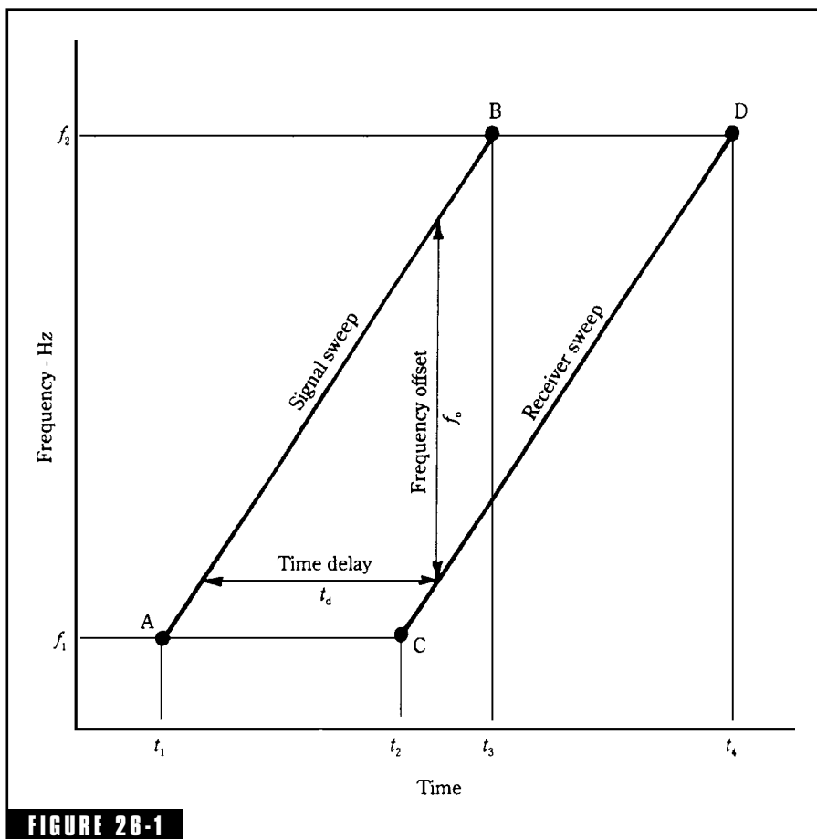
FIGURE 26-1 The basic principles of Heyser's time-delay spectrometry measurements. The outgoing signal is swept linearly from A to B. After a delay appropriate to select out the reflection desired, the receiver is swept from C to D. Only energy from the desired reflection is accepted; the receiver is detuned to all others.
