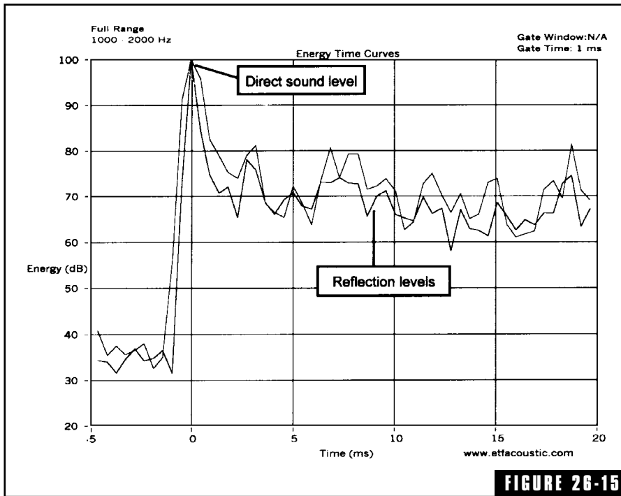
Energy-time curve of a loudspeaker measured at 1 m distance with minimal reflections. (Courtesy of Doug Plumb, AcoustiSoft.)
