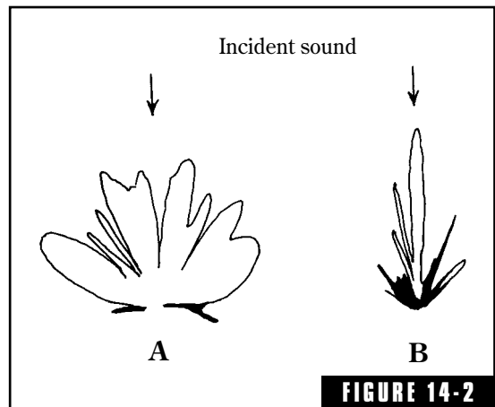
When the wells of Fig. 14-1 were accidentally made 1/2 wavelength deep, the almost pure specular reflection of B resulted, the same as for a flat sheet of metal. When another diffuser was made with the correct 1/4 wavelength depths, the very favorable diffusion pattern of A was obtained. With permission of M.R. Schroeder and Applied Science Publishers, Ltd., London.
