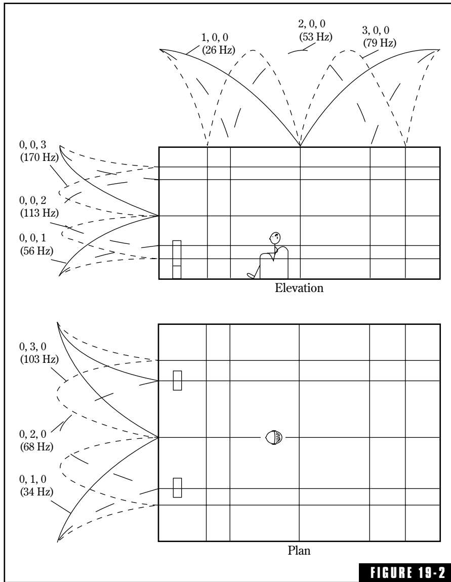
Plan and elevation views of listening room of Fig. 19-1 showing the low-frequency modal pressure distributions of the first three axial modes of Table 19-1.
