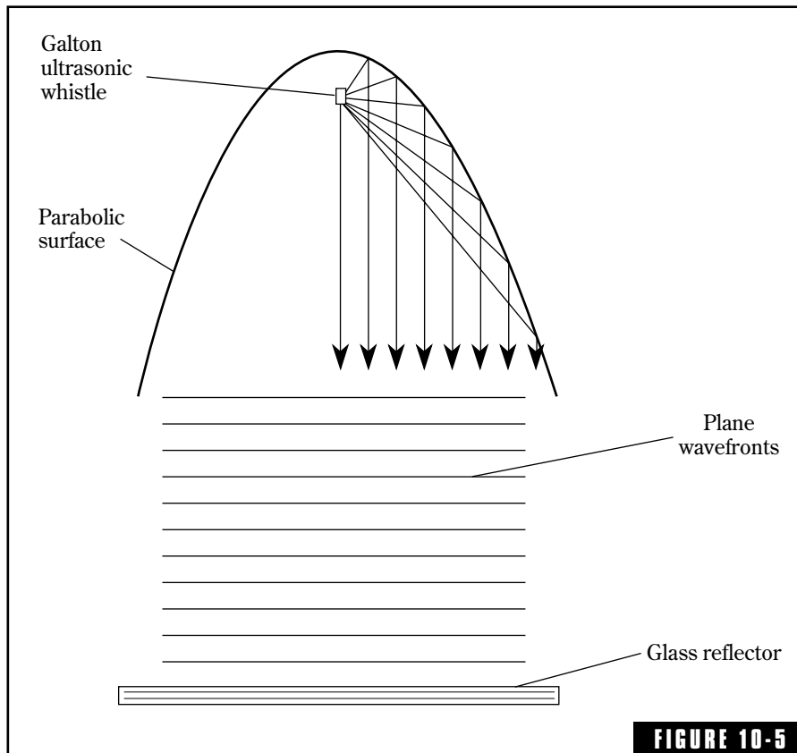
FIGURE 10-5 A parabolic surface can focus sound precisely at a focal point or, the converse, a sound source placed at the focal point can produce plane, parallel wavefronts. In this case, the source is an ultrasonic Galton Whistle blown by compressed air with the results shown in Figs. 10-6 and 10-7.
