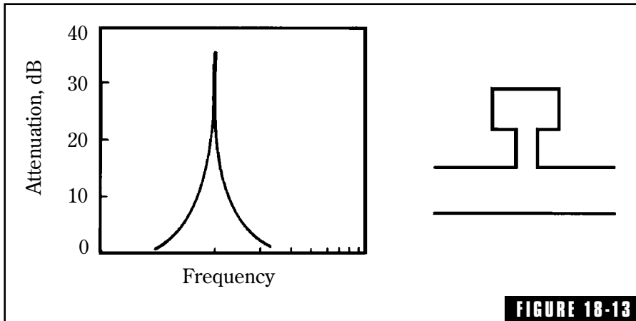
FIGURE 18-13 Attenuation characteristics of the tuned-stub silencer. Adapted from Sanders. 4
