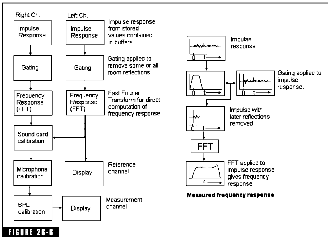
Block diagram of ETF 5’s frequency response measurement methodology. (Courtesy of Doug Plumb, AcustiSoft.)
