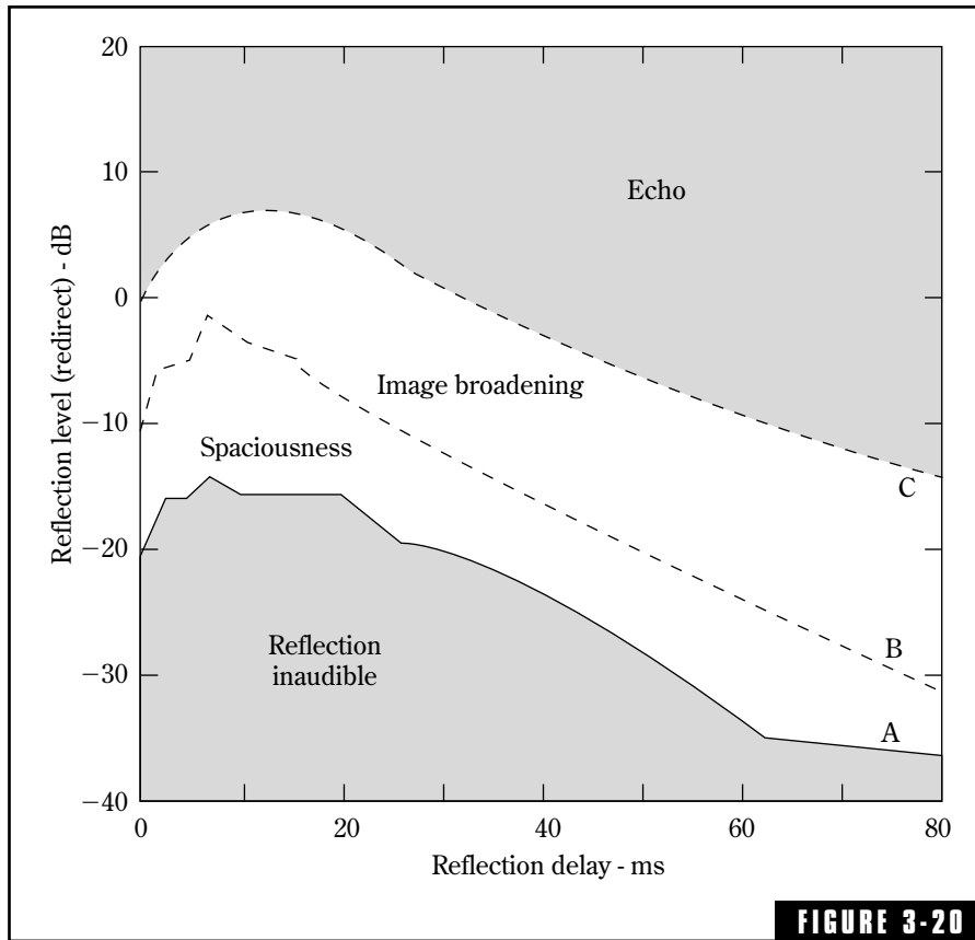
FIGURE 3-20 The effects of lateral reflections on the perception of the direct sound in a simulated stereo arrangement. These measurements were made in anechoic conditions, lateral angles 45–90 degrees, with speech as the signal. (A) Absolute threshold of audibility of the reflection. (B) Image shift/broadening threshold (A & B After Olive and Toole, 22 and Toole. 23 ) (C) Lateral reflection perceived as a discrete echo (After Meyer and Schodder, 24 and Lochner and Burger 25 ).
