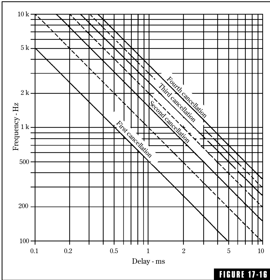
FIGURE 17-16 The magnitude of the delay determines the frequencies at which destructive interference (cancellations) and constructive interference (peaks) occur. The broken lines indicate the peaks between adjacent cancellations.
