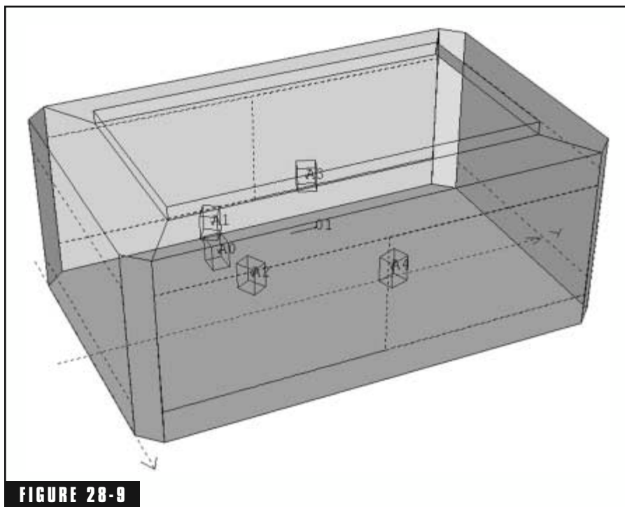
FIGURE 28-9 3D model of a listening room with five matching speakers in the ITU configuration. The model illustrates how the chosen variables describe the corner detail, soffit, and allocation of acoustical treatment to various sections on the room's boundaries.
