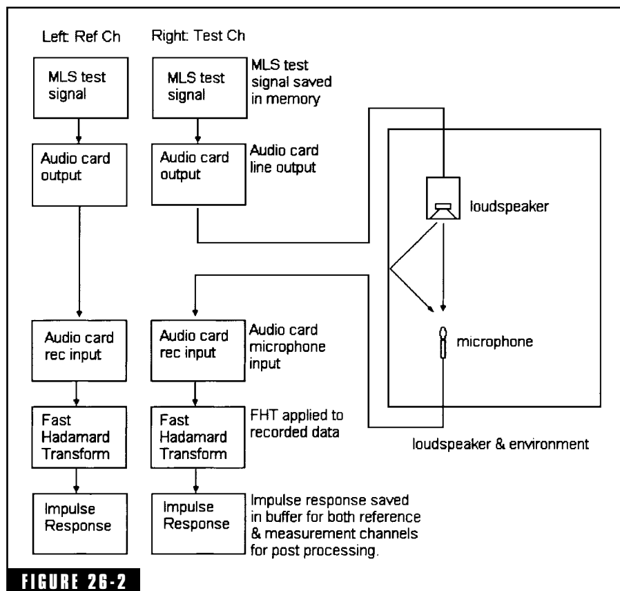
Block diagram of ETF 5's impulse response measurement methodology. (Courtesy of Doug Plumb, AcustiSoft.)
