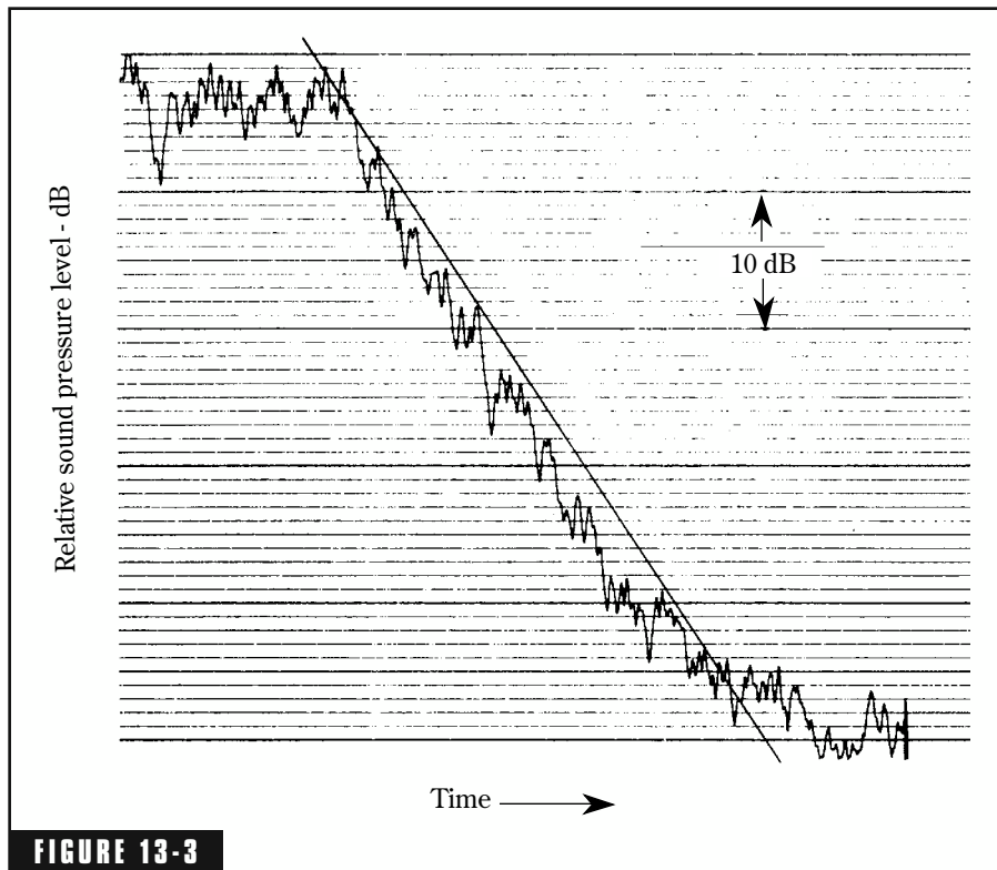
FIGURE 13-3 The nonexponential form of this decay, taken in a 400-seat chapel, is attributed to acoustically coupled spaces. The absence of a diffuse sound field is indicated.
