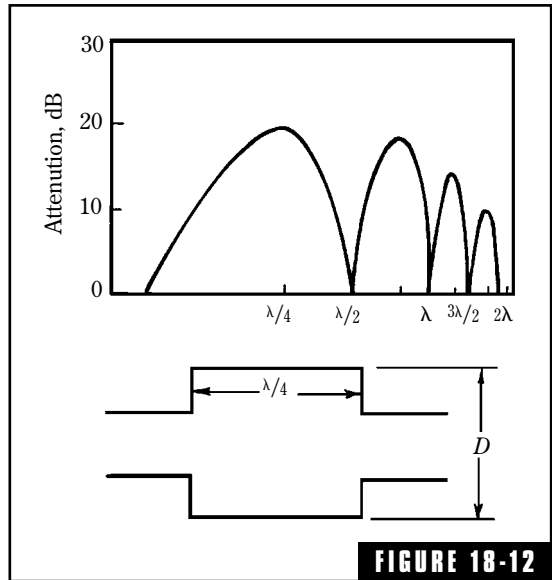
FIGURE 18-12 Attenuation characteristics of a reactive type of silencer, the expansion chamber. Sound is attenuated by virtue of the energy reflected back toward the source, canceling some of the oncoming sound. Adapted from Sanders. 4
