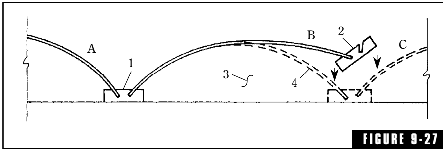
The method of stretching the plywood or hardboard skin over the poly bulkheads shown in Fig. 9-26.
