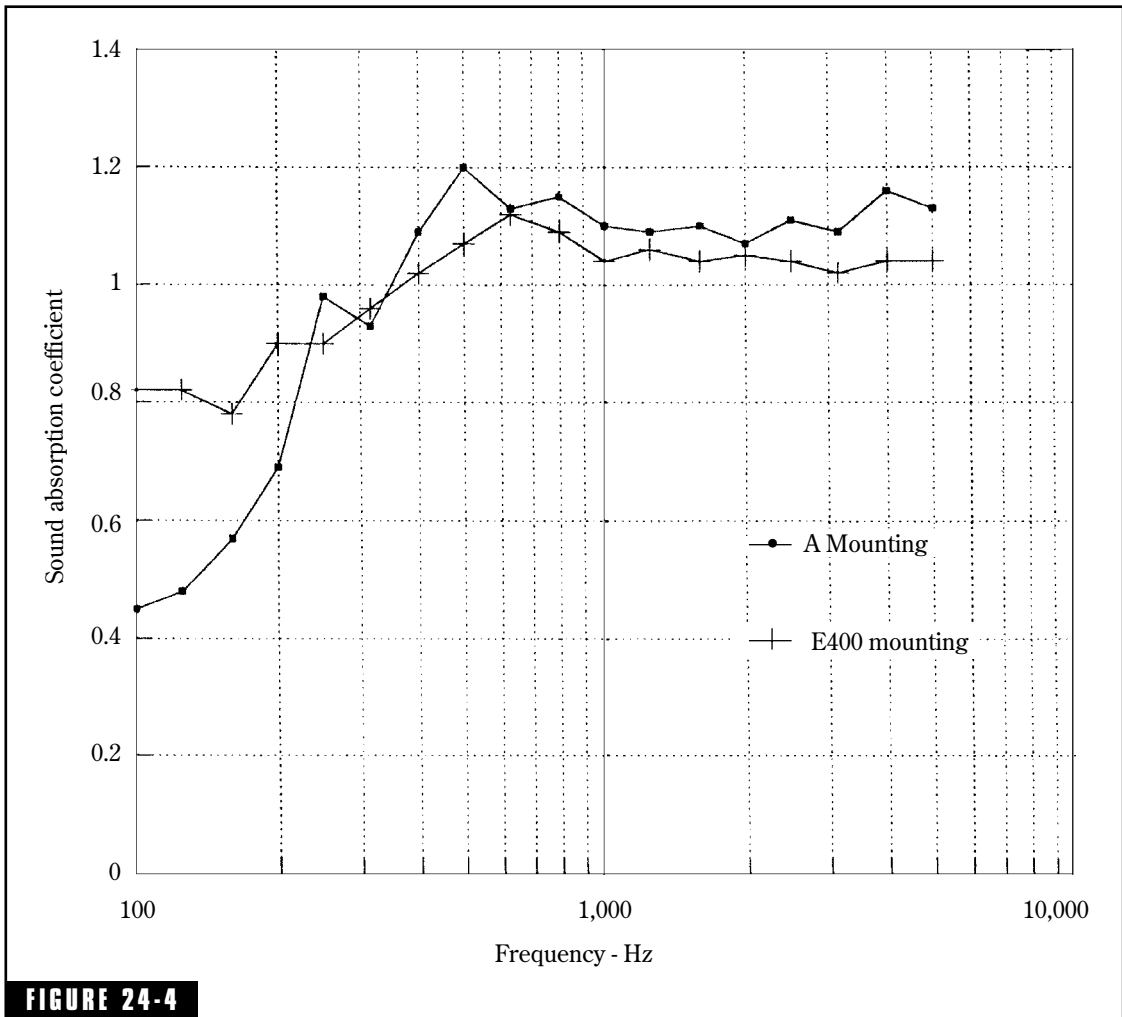
Abffusor™ absorption coefficients.
