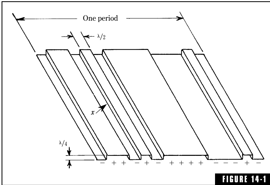
A metal sheet folded to conform to a maximum-length sequence used by Schroeder to check the diffusion of 3-cm radio waves. The wells are all 1/4 wavelength in depth.
