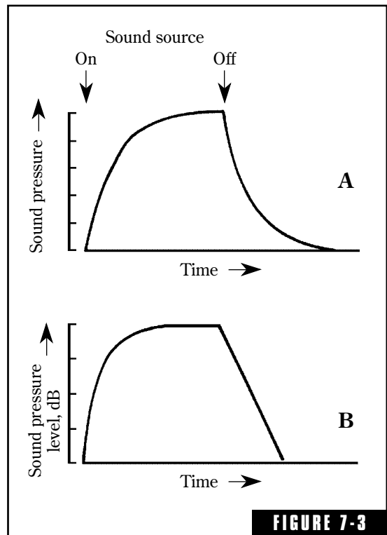
The growth and decay of sound in a room. (A) Vertical scale in linear sound pressure units. (B) The vertical scale in logarithmic units (decibels).
