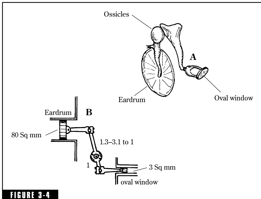
(A) The ossicles (hammer, anvil, and stirrup) of the middle ear, which transmit mechanical vibrations of the eardrum to the oval window of the cochlea. (B) A mechanical analog of the impedance-matching function of the middle ear. The difference in area between the eardrum and the oval window, coupled with the step-down mechanical linkage, match the motion of the air-actuated eardrum to the fluid-loaded oval window.
