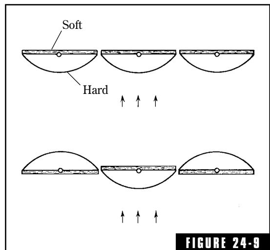
Rotating elements can vary the reverberation characteristics of a room. They have the disadvantage of requiring considerable space to accommodate the rotating elements.
