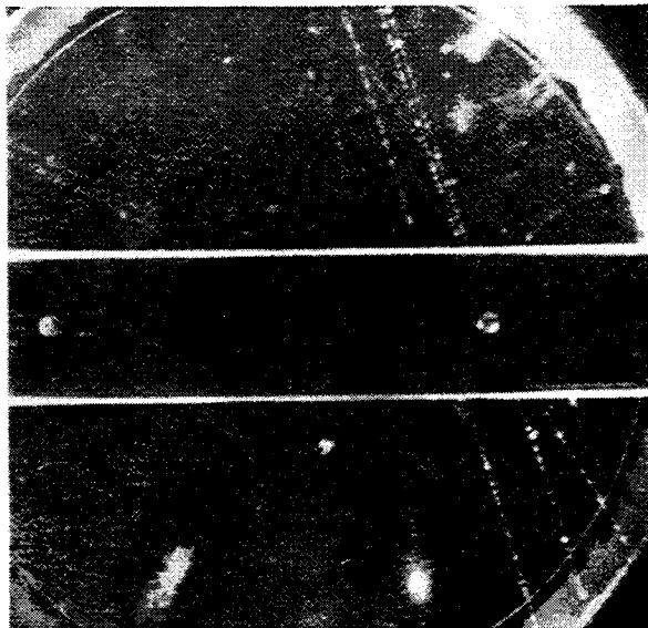
Fig. 17. Penetrating showers with no electronic component. Four associated positive particles traverse a 3.5 cm lead plate. The momenta of three of them are 3.3 , 0.9 and 1.0 \times 10^9 eV/c. One is anomalously scattered through 13^\circ . The nature of the particles in such showers is not yet certain, but they may consist of a mixture of protons and positive \pi -mesons. H = 7,000 gauss (Rochester and Butler, 1947)
