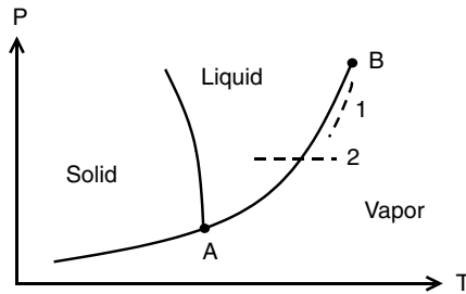
Fig. 1.1 The phase diagram for water.
