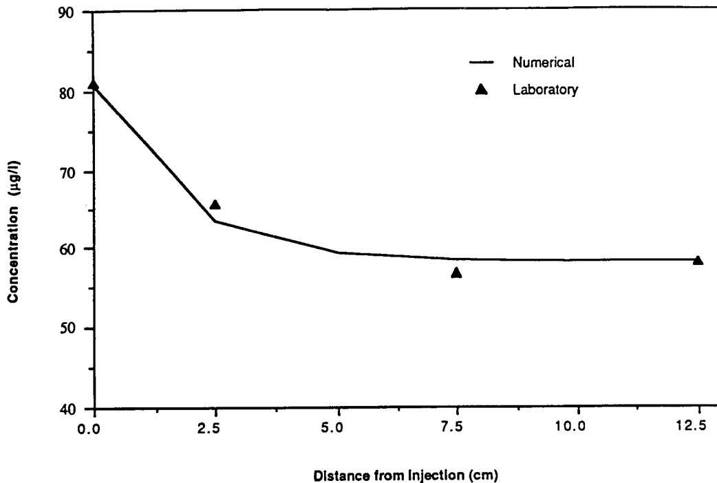
Figure 4. Numerical curve fit to the CTC profile at a detention time of 50.0 min. The k and K_s are 0.030 \mu\text{g}/\text{mg cell}\cdot\text{day} and 4.5 \mu\text{g}/\text{l} , respectively.
