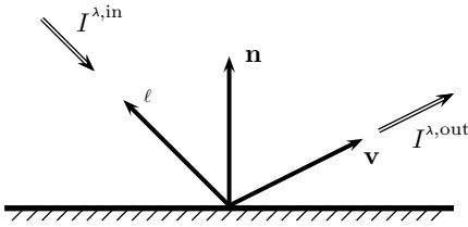
Figure III.13. The BRIDF function relates the outgoing light intensity and the incoming light intensity according to \text{BRIDF}(\ell, \mathbf{v}, \lambda) = I^{\lambda, \text{out}} / I^{\lambda, \text{in}} .
