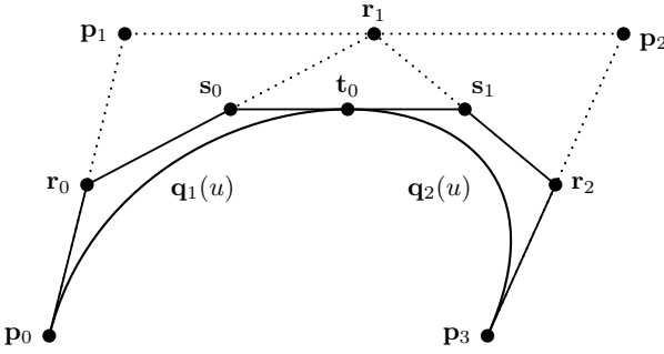
Figure VII.5. The de Casteljau method for computing \mathbf{q}(u) for \mathbf{q} a degree three Bézier curve is the basis for finding the new points needed for recursive subdivision. Shown here is the u = 1/2 case. The points \mathbf{p}_0, \mathbf{r}_0, \mathbf{s}_0, \mathbf{t}_0 are the control points for the Bézier curve \mathbf{q}_1(u) that is equal to the first half of the curve \mathbf{q}(u) , that is, starting at \mathbf{p}_0 and ending at \mathbf{t}_0 . The points \mathbf{t}_0, \mathbf{s}_1, \mathbf{r}_2, \mathbf{p}_3 are the control points for the curve \mathbf{q}_2(u) equal to the second half of \mathbf{q}(u) , that is, starting at \mathbf{t}_0 and ending at \mathbf{p}_3 .
