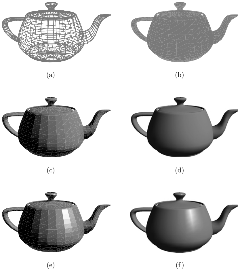
Figure III.1. Six teapots with various shading and lighting options. (a) Wireframe teapot. (b) Teapot drawn with solid color but no lighting or shading (c) Teapot with flat shading with only ambient and diffuse lighting. (d) Teapot drawn with Gouraud interpolation with only ambient and diffuse reflection. (e) Teapot drawn with flat shading with ambient, diffuse, and specular lighting. (f) Teapot with Gouraud shading with ambient, diffuse, and specular lighting. See Color Plate 4.
