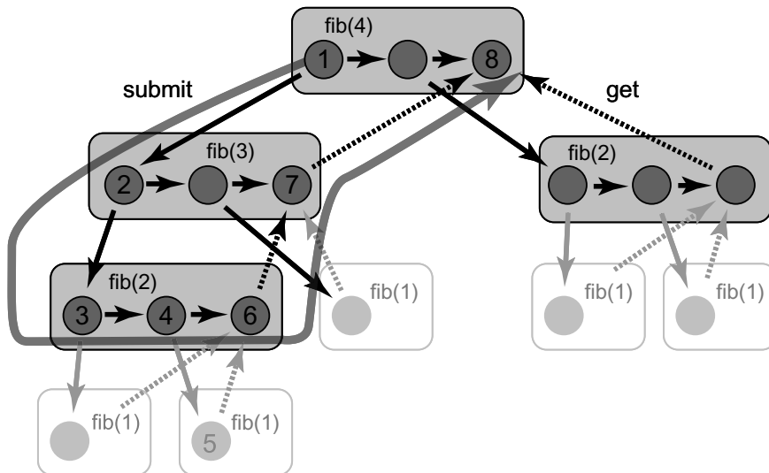
Figure 16.8 A sub-DAG in the 6th step of the FibTask(4) computation. The grey line marks the longest path. We know that the last step of FibTask(2) , which is next on the critical path, is ready to execute because the steps it depends on have been completed (it has no incoming edges apart from its preceding step in program order). Moreover, we know this is an idle step: there is not enough work for all the processors. But the scheduler is greedy, so we must have scheduled the last step of FibTask(2) in this step. This is an example of how every idle round shortens this critical path by one node (other steps may shorten it too, but we do not count them).
