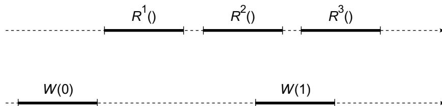
Figure 4.3 A single-writer, single-reader register execution: R^i is the i^{\text{th}} read and W(v) is a write of value v . Time flows from left to right. No matter whether the register is safe , regular , or atomic , R^1 must return 0, the most recently written value. If the register is safe then because R^2 and R^3 are concurrent with W(1) , they can return any value in the range of the register. If the register is regular , R^2 and R^3 can each return either 0 or 1. If the register is atomic then if R^2 returns 1 then R^3 also returns 1, and if R^2 returns 0 then R^3 could return 0 or 1.
