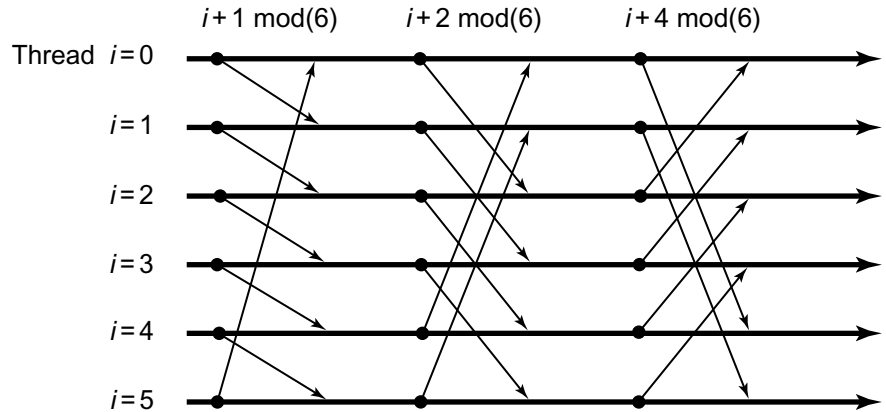
Figure 17.21 Communication in the dissemination barrier. In each round r a thread i communicates with thread i+2^r \pmod{n} .
