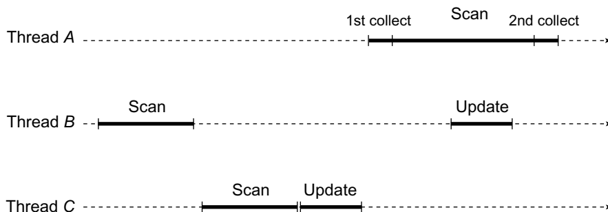
Figure 4.18 Here is why a thread A that fails to complete a clean double collect cannot simply take the latest snapshot of a thread B that performed an update() during A 's second collect. B 's snapshot was taken before A started its scan() , i.e., B 's snapshot did not overlap A 's scan. The danger, illustrated here, is that a thread C could have called update() after B 's scan() and before A 's scan() , making it incorrect for A to use the results of B 's scan() .
