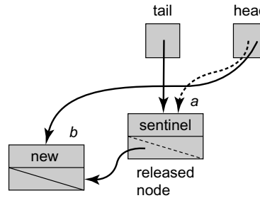
Figure 10.13 Why dequeuers must help advance tail in Line 35 of Fig. 10.11. Consider the scenario in which a thread enqueueing node b has redirected a 's next field to b , but has yet to redirect tail from a to b . If another thread starts dequeuing, it will read b 's value and redirect head from a to b , effectively removing a while tail still refers to it. To avoid this problem, the dequeuing thread must help advance tail from a to b before redirecting head .
