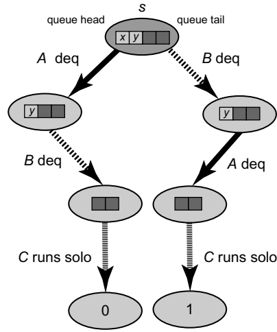
Figure 5.8 Case: A and B both call \text{deq}() .
