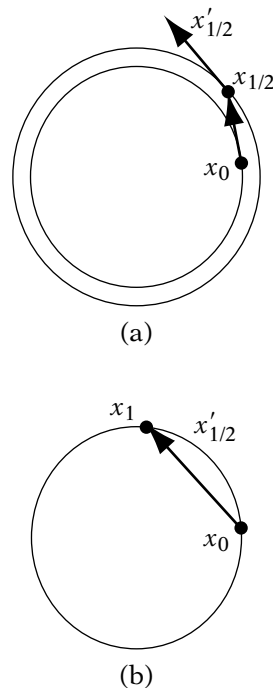
FIGURE 13.6 (a) Orbit example, showing first step of midpoint method: getting the midpoint derivative. (b) Orbit example, stepping with midpoint derivative to next estimate.
