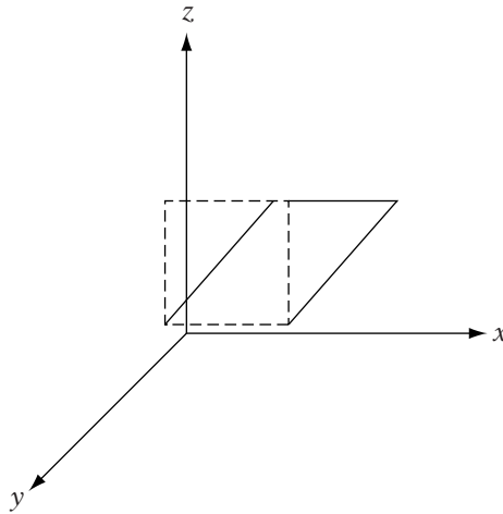
FIGURE 4.12 z -shear on square.
