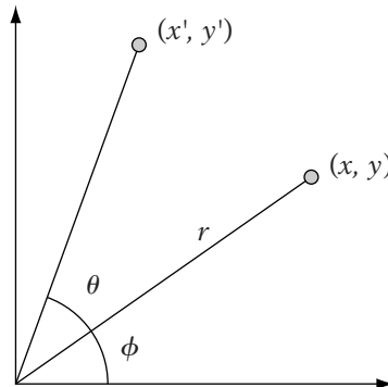
FIGURE 4.6 Rotation in xy plane.
