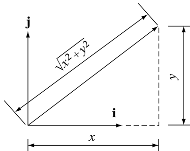
FIGURE 2.9 Length of 2D vector.
