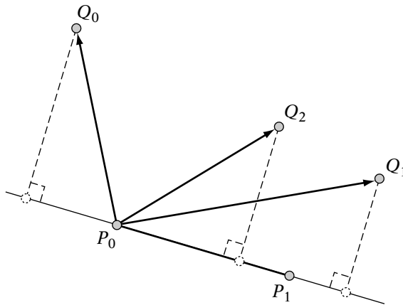
FIGURE 12.3 Three cases when projecting a point onto line segment.
