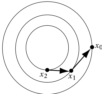
FIGURE 13.7 Implicit Euler. The arrows point backwards to indicate that we are getting the derivative from the next time step.
