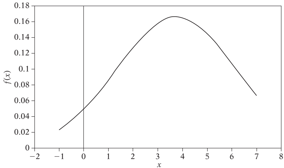
FIGURE 11.7 General normal distribution with mean of 3.75 and standard deviation of 2.4.
