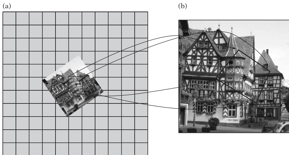
FIGURE 9.18 Mapping the square screen-space area of a pixel back into texel space: (a) screen space with pixel of interest highlighted and (b) texel-space back-projection of pixel area.
