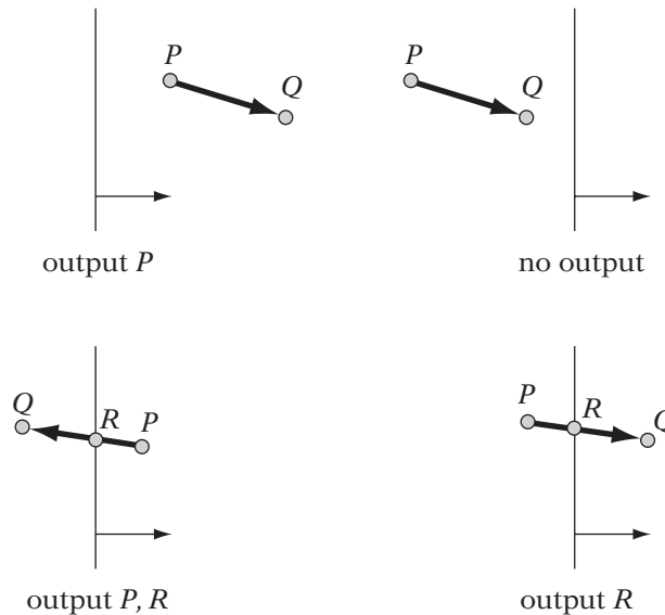
FIGURE 6.25 Four possible cases of clipping an edge against a plane.
