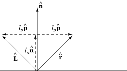
FIGURE 8.10 The relationship between the surface normal, light direction, and the reflection vector.
