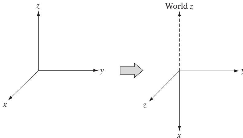
FIGURE 5.3 Demonstration of mathematical gimbal lock. A rotation of 90 degrees around y will lead to the local x -axis aligning with the -z world axis, and a loss of a degree of freedom.
