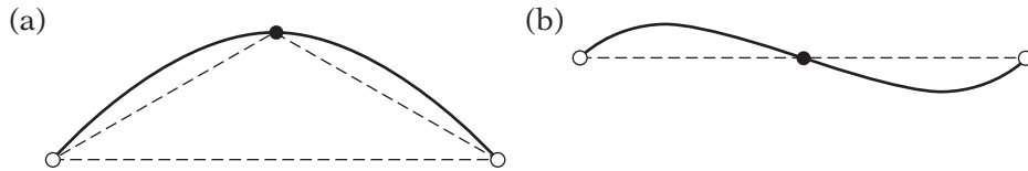
FIGURE 10.23 Midpoint test for curve straightness. (a) Total distance from endpoints to midpoint (black dot) is compared to distance between endpoints, (b) example of midpoint test failure.
