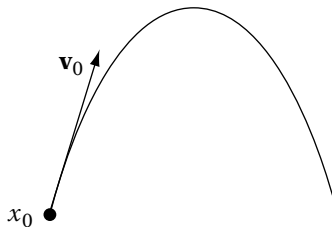
FIGURE 13.2 Parabolic path of object with initial velocity and affected only by gravity.
