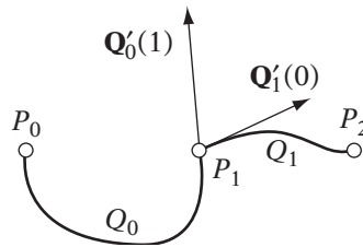
FIGURE 10.6 Piecewise Hermite curve. Tangents at P_1 have differing directions and magnitudes.
