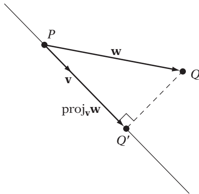
FIGURE 12.1 Closest point on a line.
