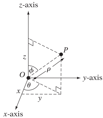
FIGURE 2.32 Relationship between spherical and Cartesian coordinates.
