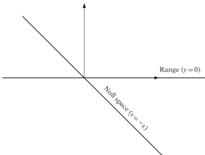
FIGURE 3.1 Range and null space for transformation \mathsf{T}(a, b) = (a + b, 0) .
