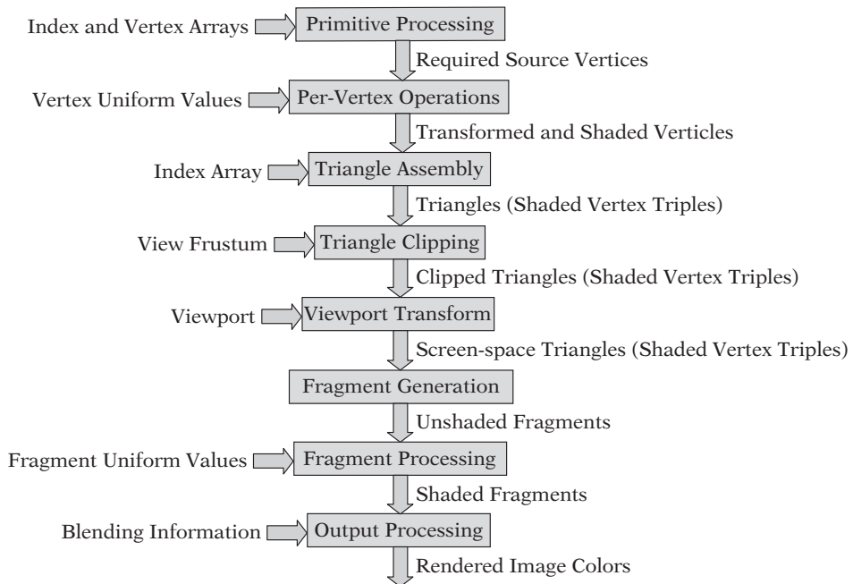
FIGURE 7.5 Details of the rendering pipeline.
