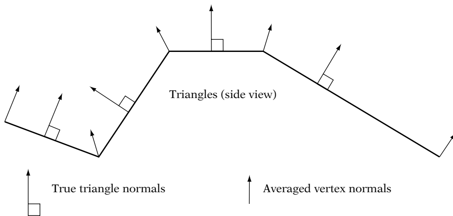
FIGURE 8.16 Averaging triangle normal vectors.
