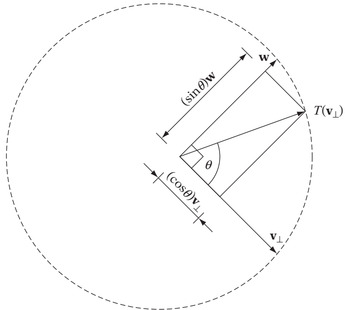
FIGURE 4.7 (a) General rotation, showing axis of rotation and rotation plane, and (b) general rotation, showing vectors on rotation plane.
