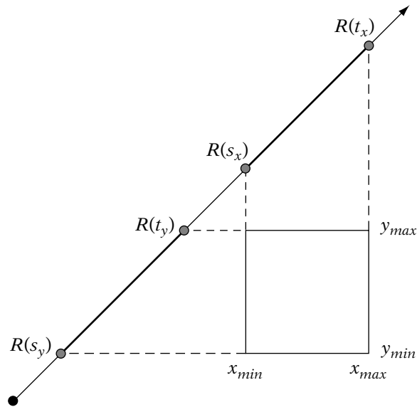
FIGURE 12.14 Axis-aligned box-ray separation test.
