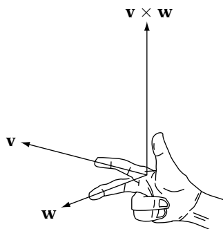
FIGURE 2.15 Cross product direction.
