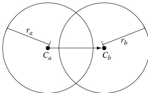
FIGURE 13.15 Determining penetration distance and collision normal.
