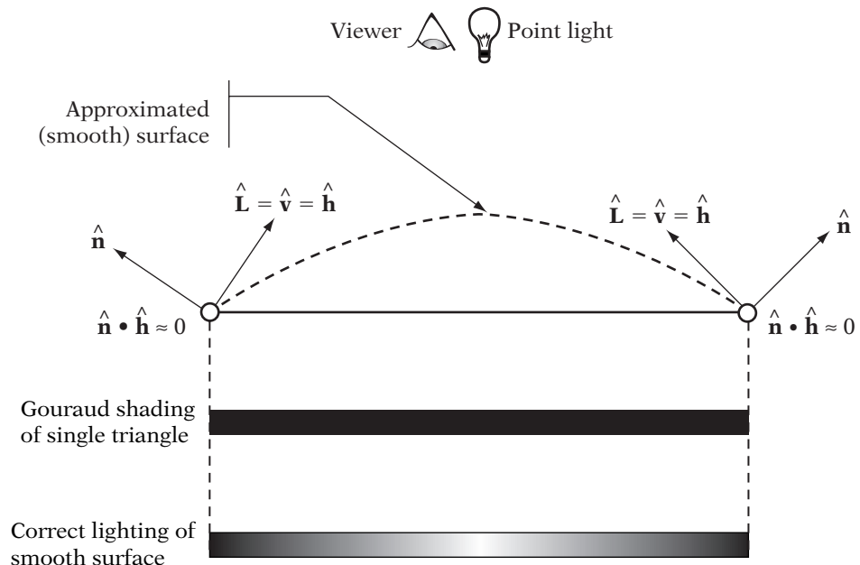
FIGURE 8.18 Gouraud shading can miss specular highlights.
