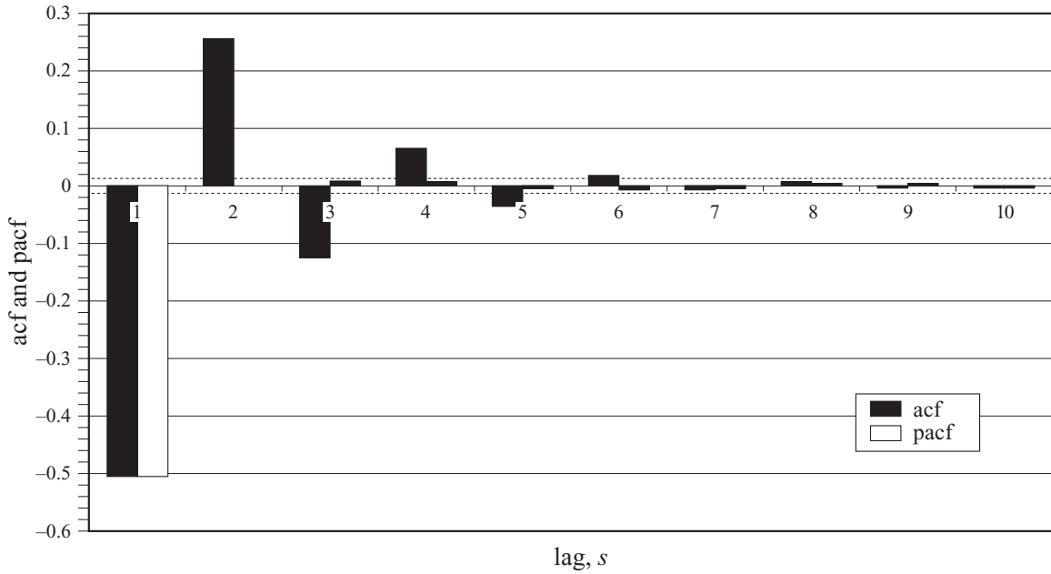
Figure 5.6 Sample autocorrelation and partial autocorrelation functions for a more rapidly decaying AR(1) model with negative coefficient: y_t = -0.5y_{t-1} + u_t
