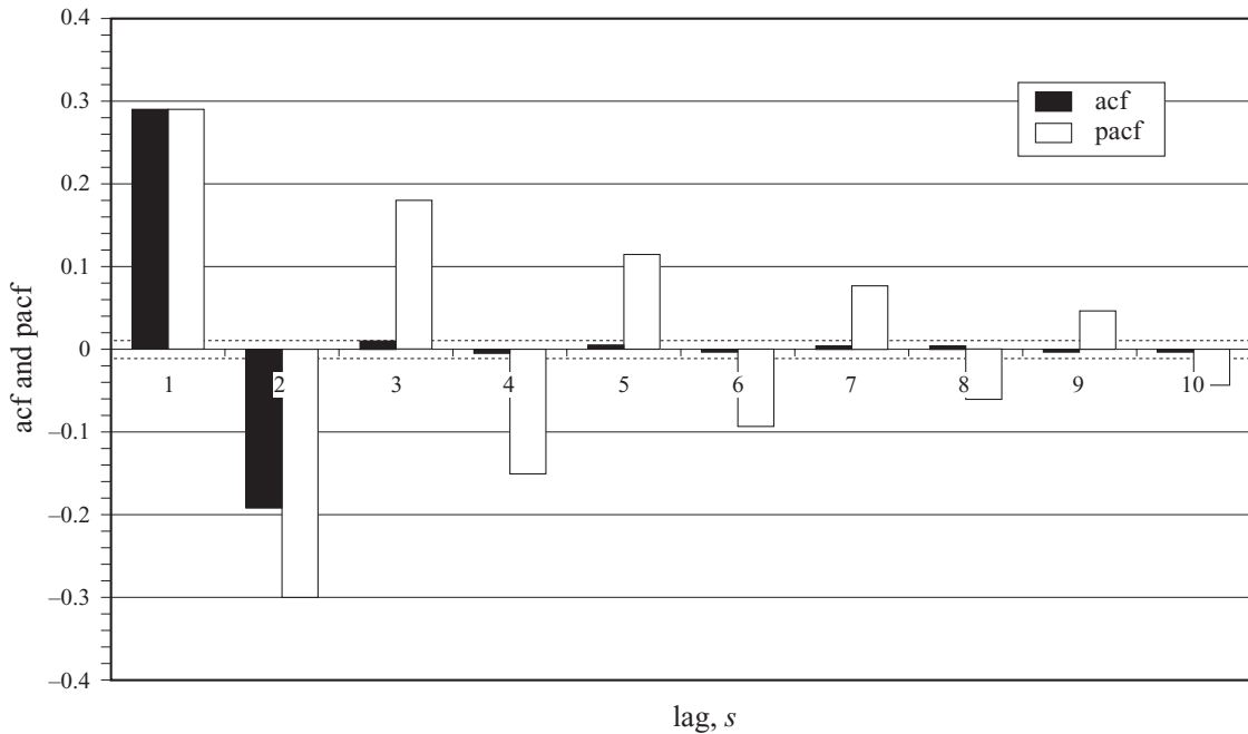
Figure 5.3 Sample autocorrelation and partial autocorrelation functions for an MA(2) model: y_t = 0.5u_{t-1} - 0.25u_{t-2} + u_t
