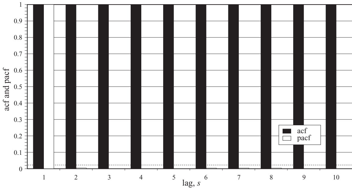
Figure 5.7 Sample autocorrelation and partial autocorrelation functions for a non-stationary model (i.e. a unit coefficient): y_t = y_{t-1} + u_t
