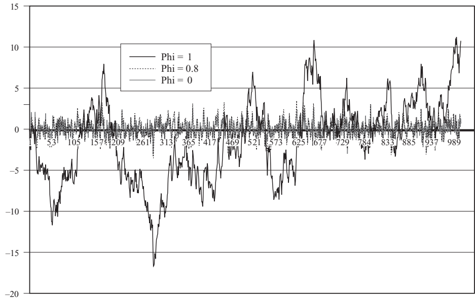
Figure 7.6 Autoregressive processes with differing values of \phi (0, 0.8, 1)
