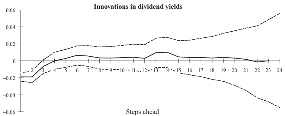
Figure 6.2 Impulse responses and standard error bands for innovations in the dividend yields
