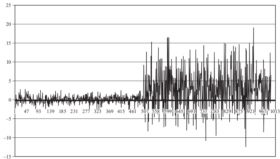
Figure 9.1 Sample time series plot illustrating a regime shift
