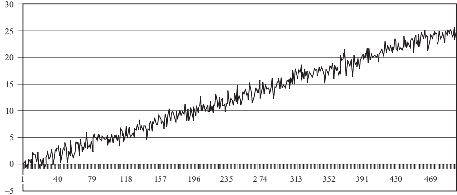
Figure 7.5 Time series plot of a deterministic trend process
