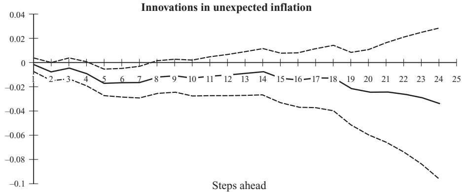
Figure 6.1 Impulse responses and standard error bands for innovations in unexpected inflation equation errors
