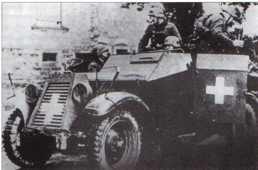
An SdKfz 13 'Bathtub' of an infantry division's reconnaissance battalion photographed during the campaign in Poland. The solid white national cross provided too good an aiming mark and was subsequently overlaid in black. (RAC Tank Museum)
