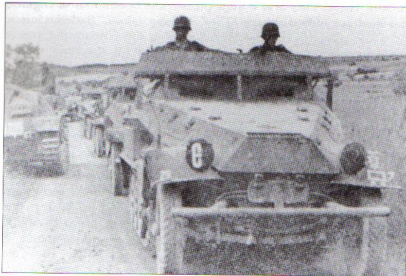
Reconnaissance troops regularly worked with the artillery's Forward Observation Officers. The vehicle shown here, photographed during the 1940 campaign in France, is the SdKfz 251/18 artillery observation half-track. The tactical markings are those of 1.Panzer-Division and No. 7 Company 1st Motor Rifle Regiment, suggesting that the latter have been required to surrender it to the FOO. The superstructure has been modified to provide a broad, flat surface for the FOO's maps and artillery board. The column is overtaking one of the few assault gun batteries to have fought in France at this time. (US National Archives)
