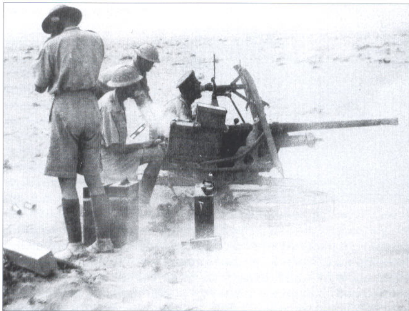
The British 2-pdr Mk I AT gun weighed 1,858lb, about twice as much as its US and German 37mm counterparts. It could be fired from its wheels, but they were normally removed for action and the gun set up on its integral three-legged mounting. Side shields were available, but seldom used.
