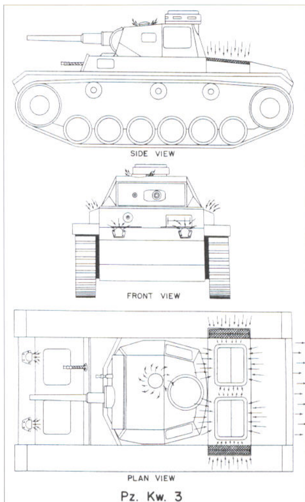
Tanks had other vulnerabilities apart from penetration of the armour. This diagram, from a US intelligence report, indicates air intakes for both the crew and engine, and engine exhausts, of a German PzKw III. Such vents were vulnerable to fire bombs, smoke and gas.
