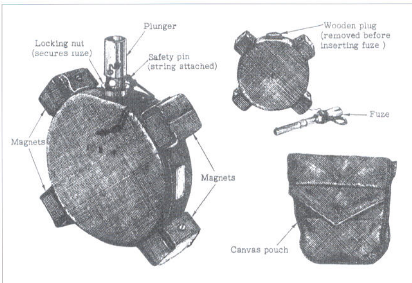
The Japanese Type 99 (1939) AT charge (99 hako-bakurai ) was small (about 4¾ in x 1½ in without the four magnets), but if two or more could be fastened together they caused a great deal of concern to tankers (see Plate H). It was issued in a canvas carrying pouch, with the fuze packed in a two-piece metal tube under the pouch flap.
