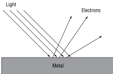
Figure 1.1: Photons hitting a material that then emits electrons
