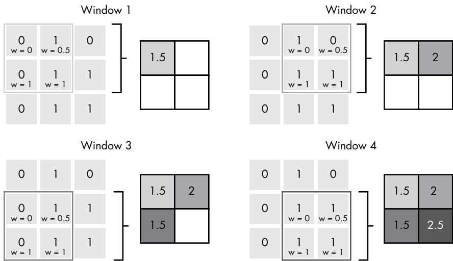
Figure 10-13: Visualization of a 2 × 2 convolutional window sliding over a 3 × 3 input space with a stride (step size) of 1, to yield a 2 × 2 output
