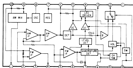
IC2 TA7758P
