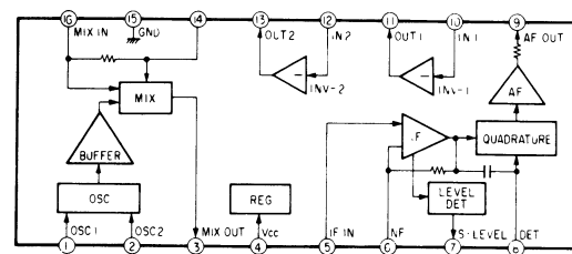
IC1 TA7761F
