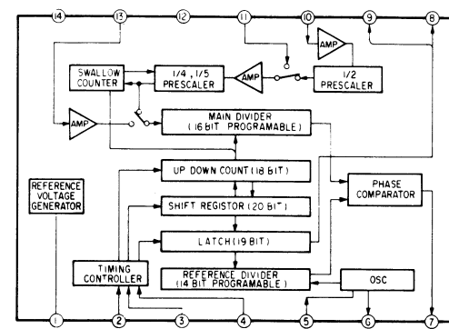
IC202 CXD1118M
