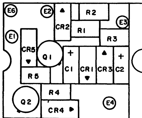
Circuit Board 1A1AIA10A2
