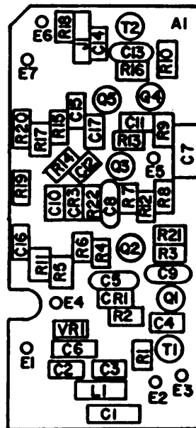
Circuit Board 1A6A1
