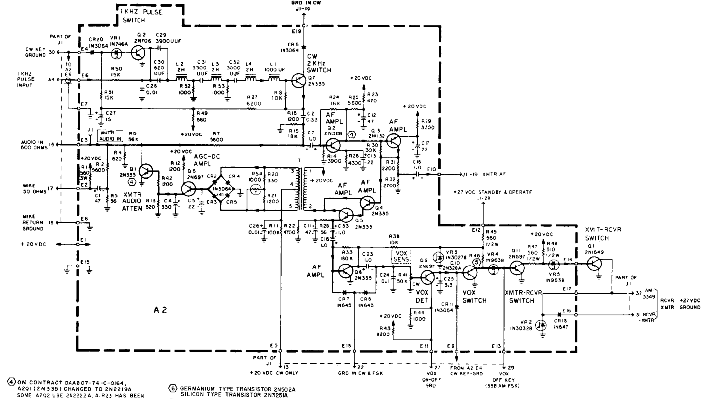
FIGURE FO-18 Transmitter IF and Audio Module 1A5 Schematic Diagram
