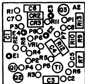
Circuit Board 1A3A1A2
