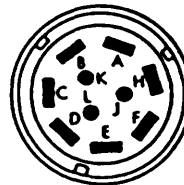
MICROPHONE, HEADSET, HANDSET, TELEGRAPH KEY OR LOUDSPEAKER CONNECTOR
