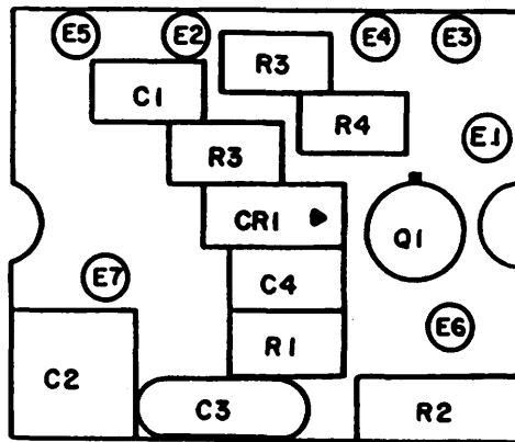
Circuit Board 1A1AIA10A1
