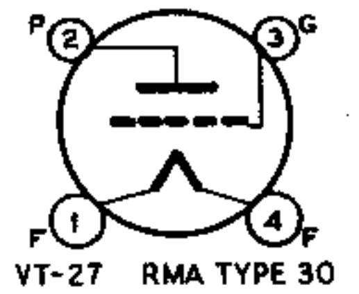
VT-27 RMA TYPE 30 Tube socket terminals, bottom view
