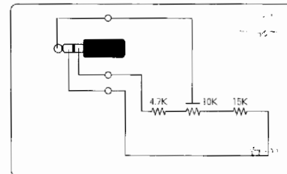
3.5mm stereo plug
