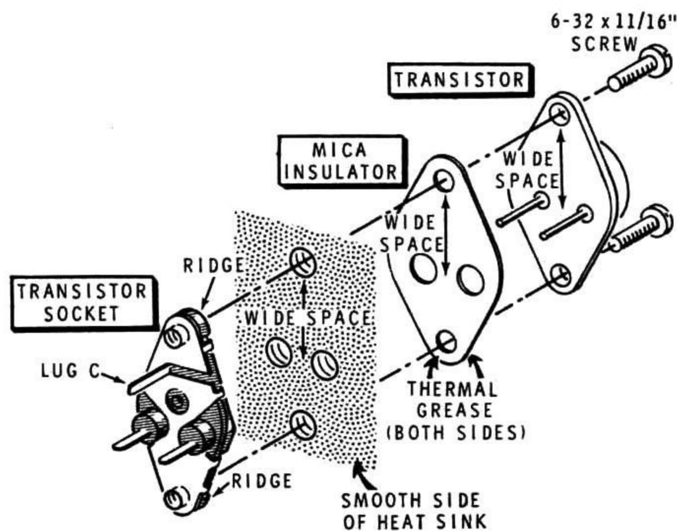
Detail 2-5A
