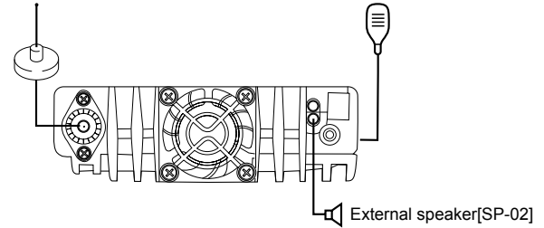
External speaker[SP-02]
