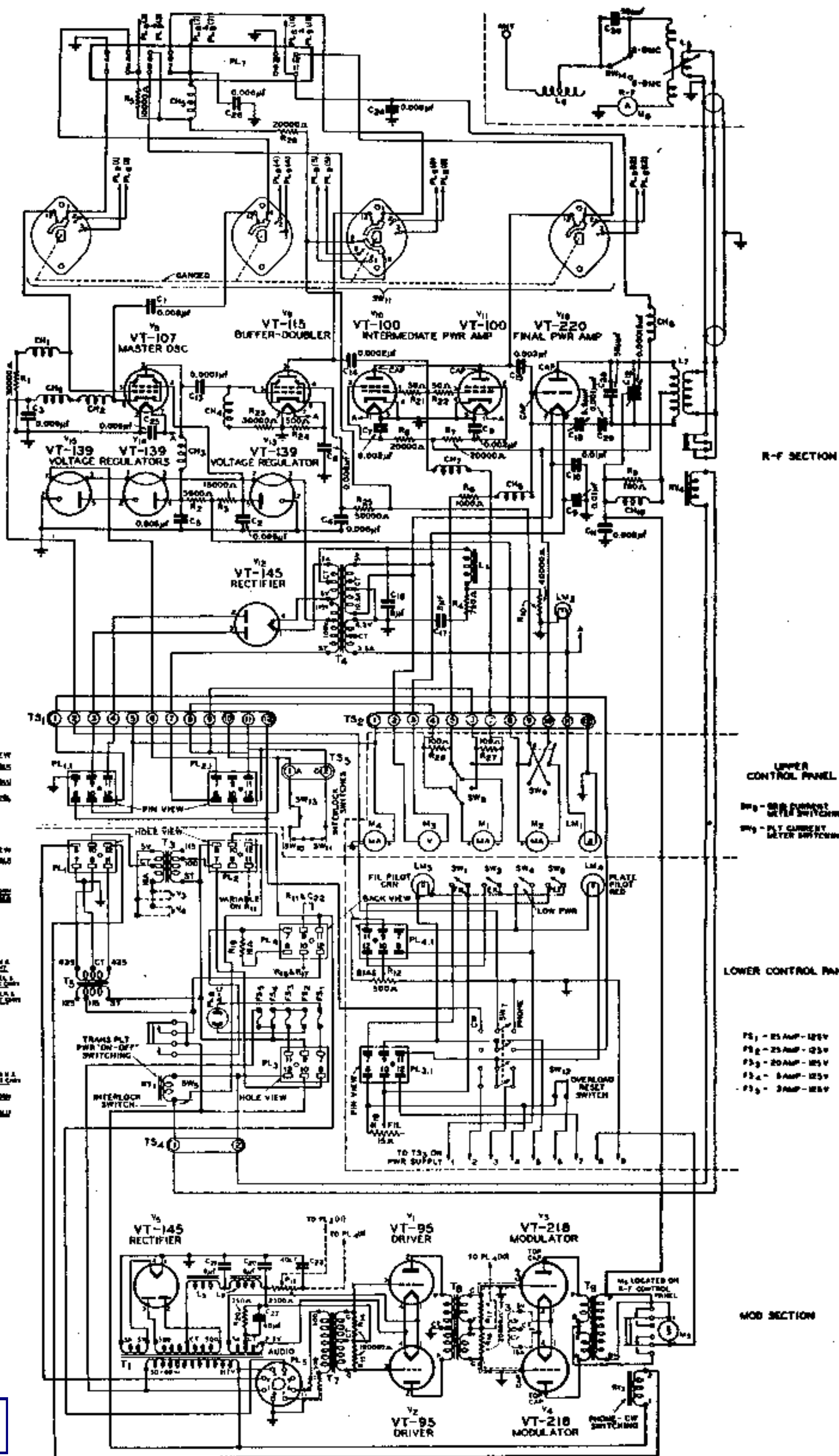
Fig. 7.—Schematic BC-610-A, BC-610-B
